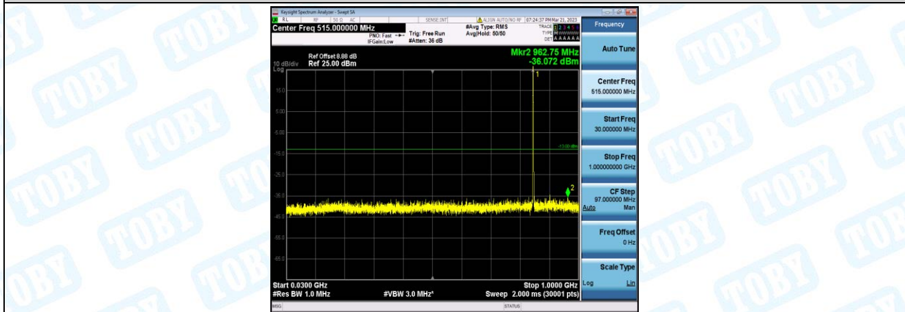
Band5-5MHz-16QAM-20625-1-0-High-30-1000--36.07-PASS
