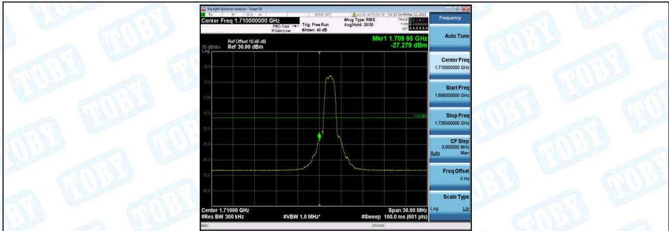
Band66-15MHz-QPSK-132047-6-0-Low--27.28-PASS
