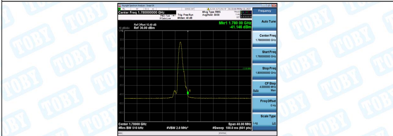
Band66-20MHz-16QAM-132572-1-0-High--41.15-PASS
