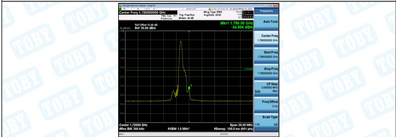
Band66-15MHz-QPSK-132597-1-0-High--34.85-PASS
