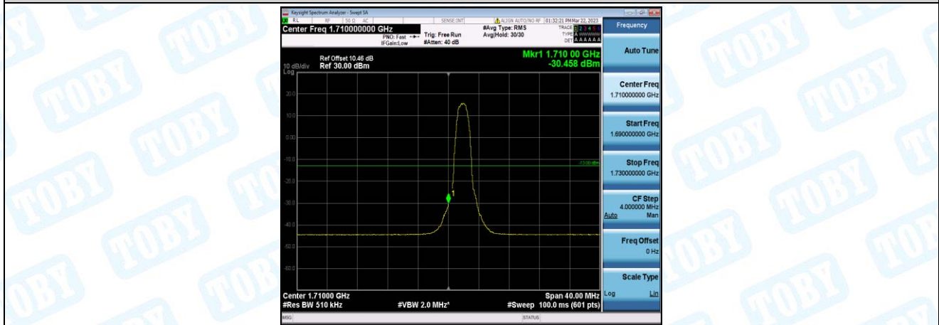
Band66-20MHz-QPSK-132072-6-0-Low--30.46-PASS
