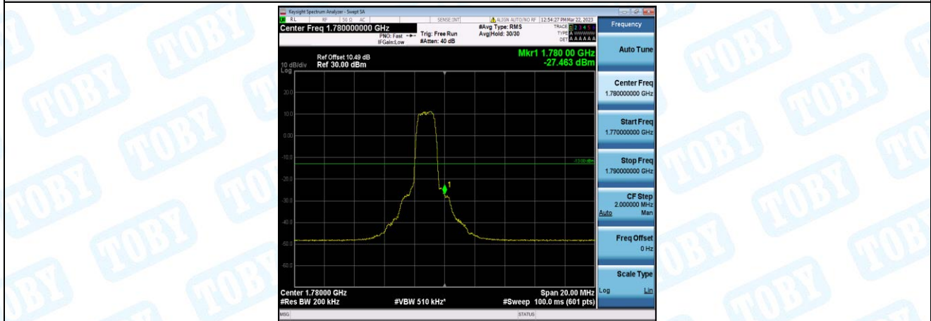
Band66-10MHz-16QAM-132622-6-0-High--27.46-PASS
