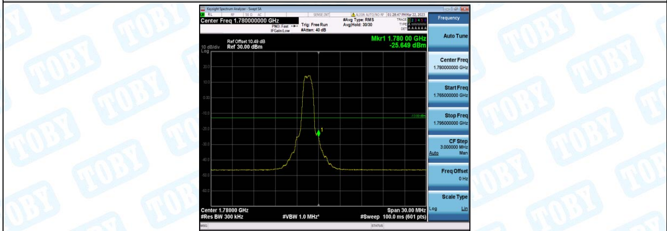
Band66-15MHz-QPSK-132597-6-0-High--25.65-PASS
