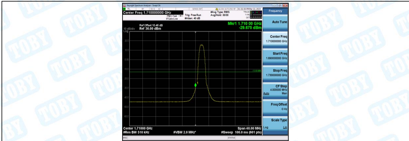
Band66-20MHz-16QAM-132072-6-0-Low--29.68-PASS
