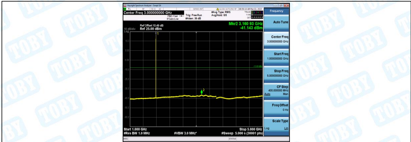
Band66-1.4MHz-16QAM-132665-1-0-High-1000-5000--41.14-PASS
