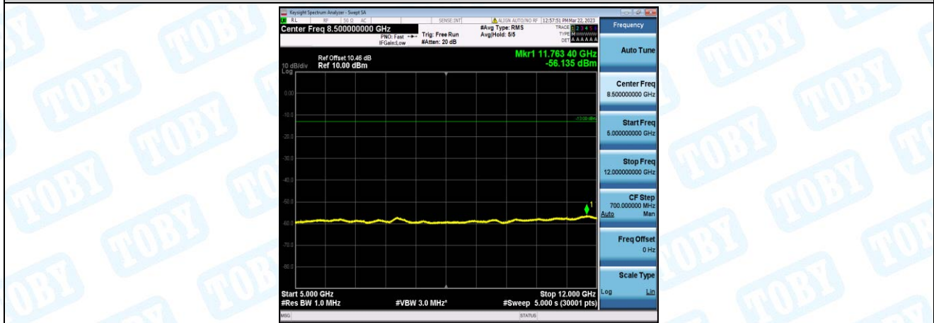
Band66-10MHz-16QAM-132022-1-0-Low-5000-12000--56.14-PASS
