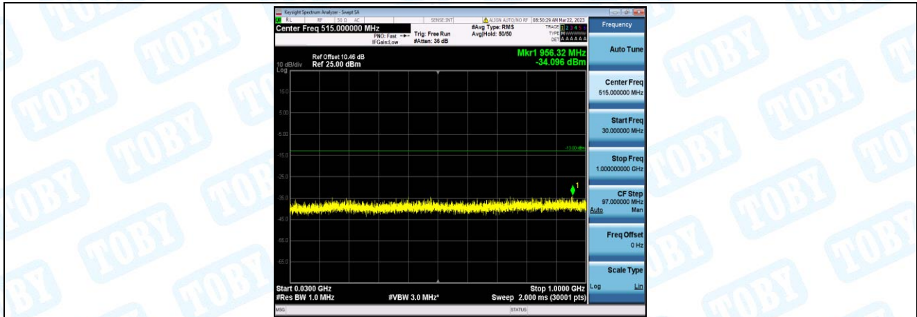
Band66-1.4MHz-16QAM-131979-1-0-Low-30-1000--34.1-PASS
