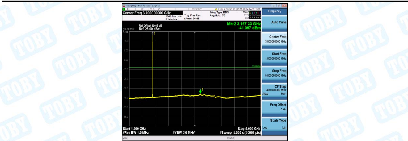
Band66-10MHz-16QAM-132022-1-0-Low-1000-5000--41.1-PASS
