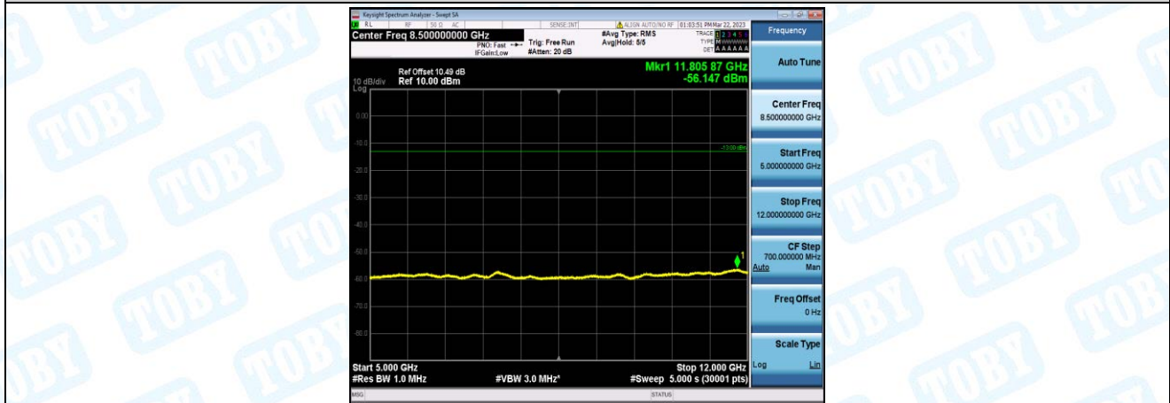
Band66-10MHz-QPSK-132622-1-0-High-5000-12000--56.15-PASS
