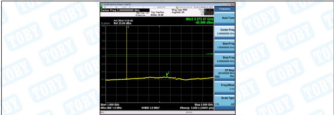
Band66-10MHz-16QAM-132622-1-0-High-1000-5000--40.99-PASS
