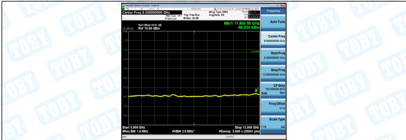
Band66-5MHz-QPSK-132322-1-0-Low-5000-12000--56.02-PASS
