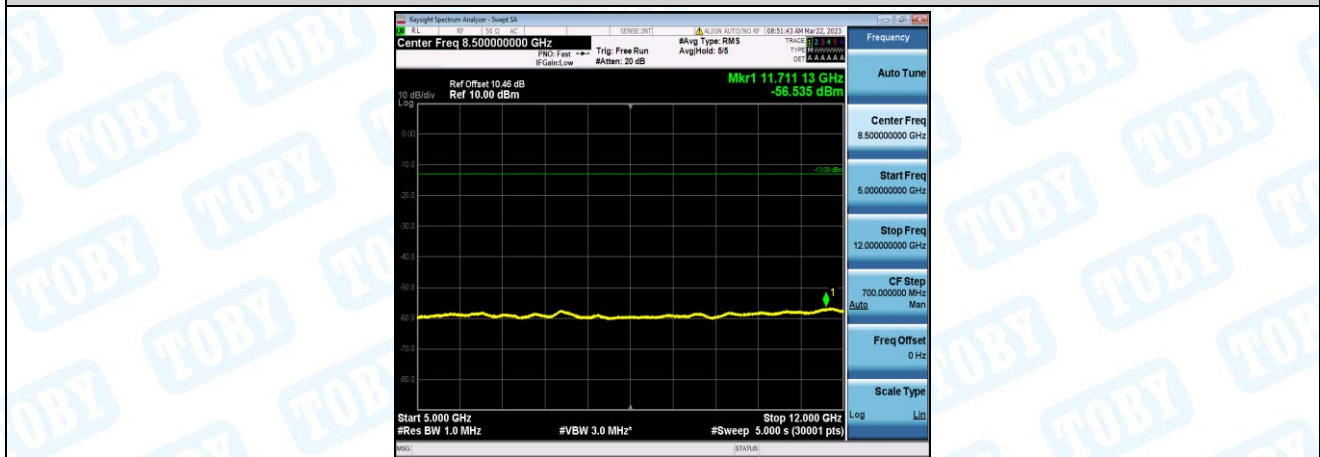
Band66-1.4MHz-16QAM-131979-1-0-Low-5000-12000--56.54-PASS
