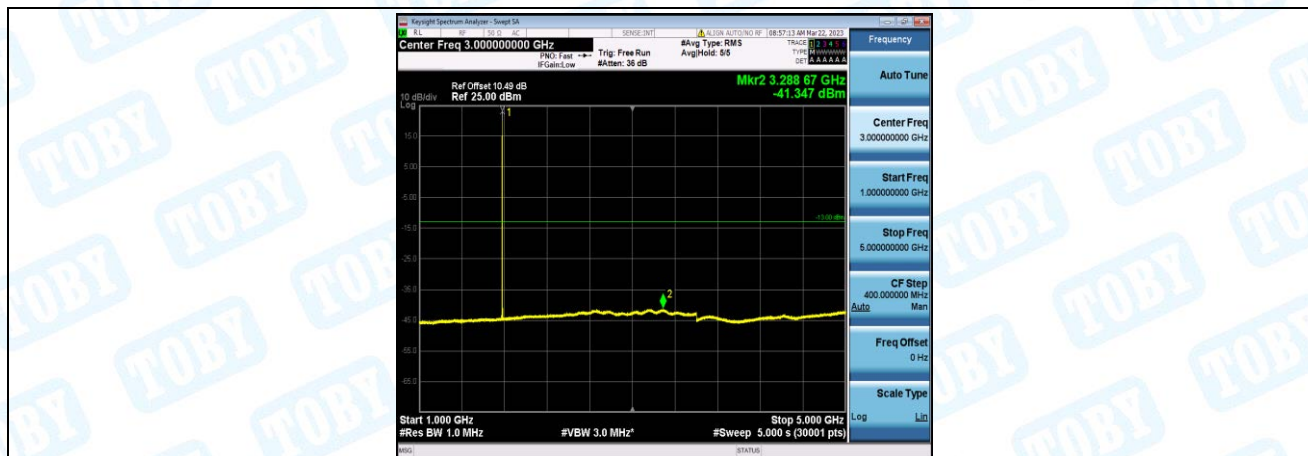
Band66-1.4MHz-QPSK-132665-1-0-High-1000-5000--41.35-PASS
