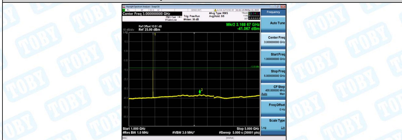
Band66-10MHz-16QAM-132322-1-0-Low-1000-5000--41.07-PASS
