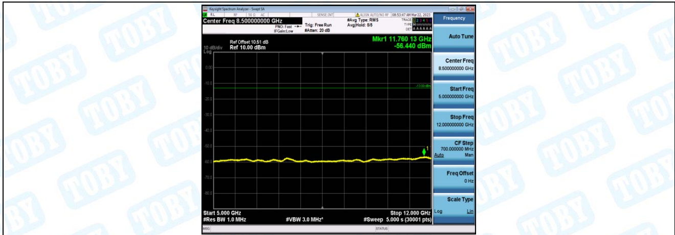
Band66-1.4MHz-QPSK-132322-1-0-Low-5000-12000--56.44-PASS
