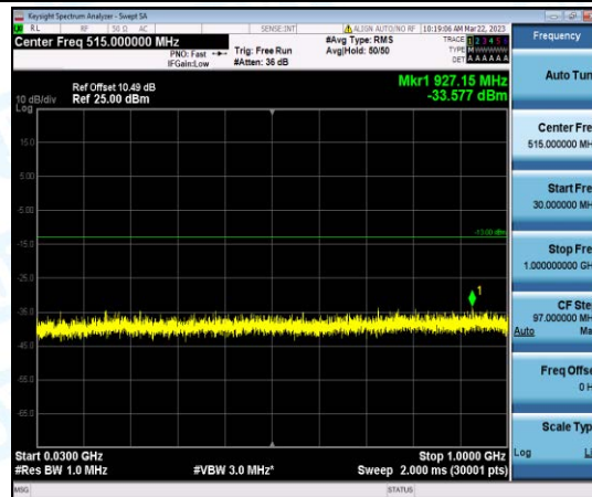
Band66-3MHz-QPSK-132657-1-0-High-30-1000--33.58-PASS
