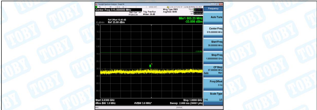
Band66-10MHz-16QAM-132022-1-0-Low-30-1000--33.86-PASS
