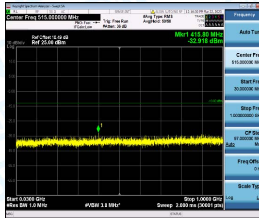
Band66-5MHz-16QAM-132647-1-0-High-30-1000--32.92-PASS
