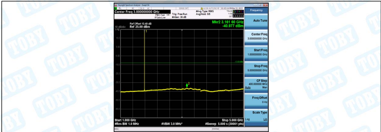
Band66-10MHz-QPSK-132622-1-0-High-1000-5000--40.98-PASS
