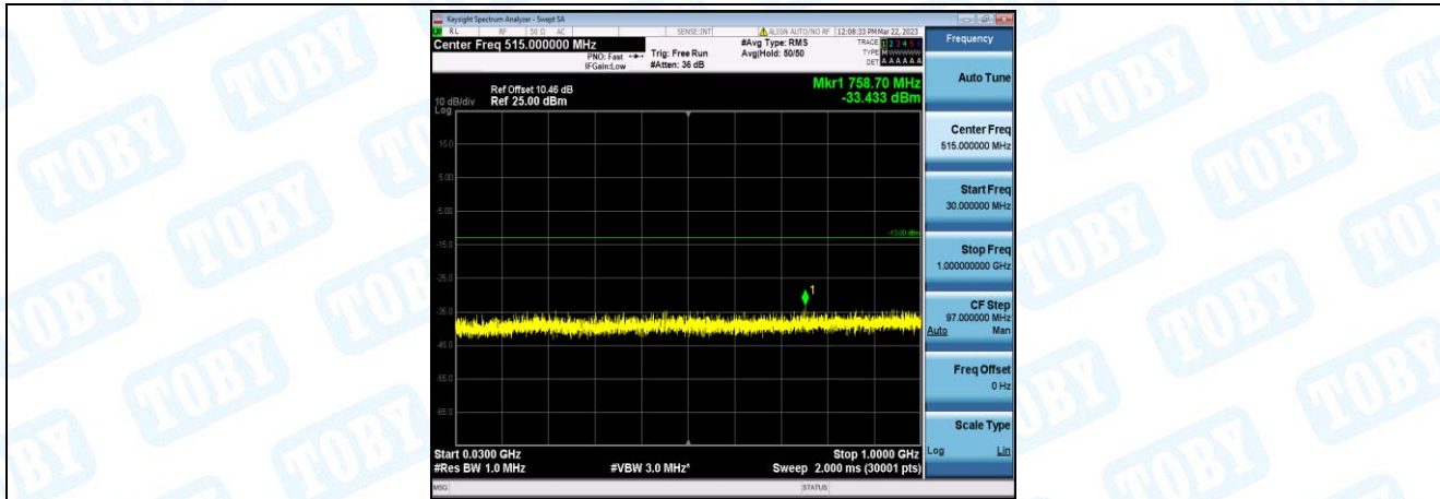
Band66-5MHz-16QAM-131997-1-0-Low-30-1000--33.43-PASS
