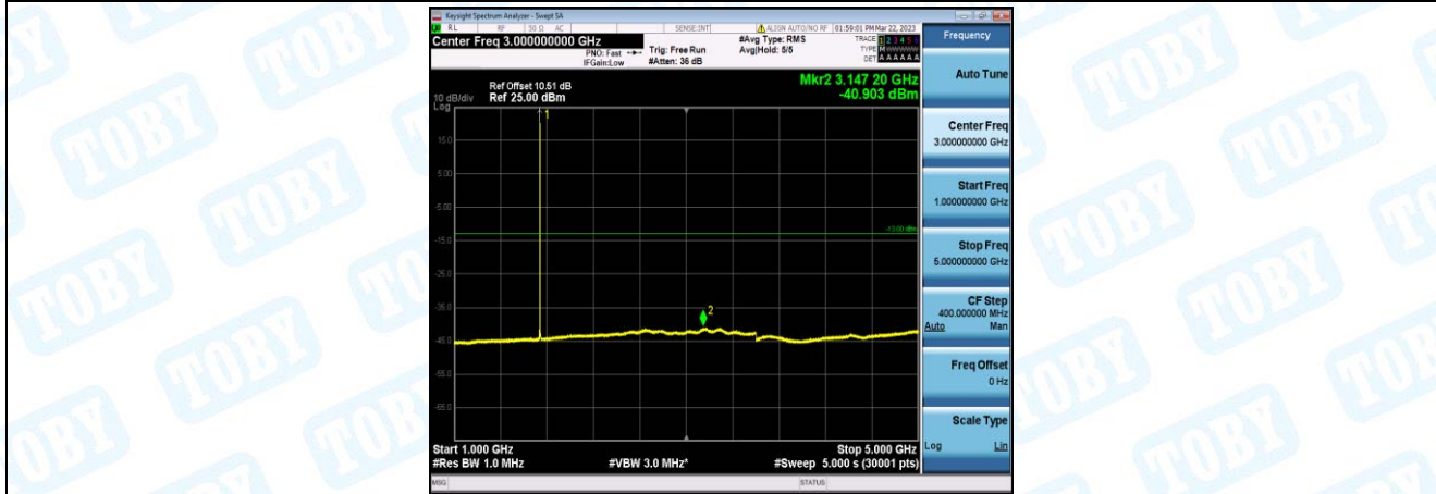
Band66-15MHz-QPSK-132322-1-0-Low-1000-5000--40.9-PASS
