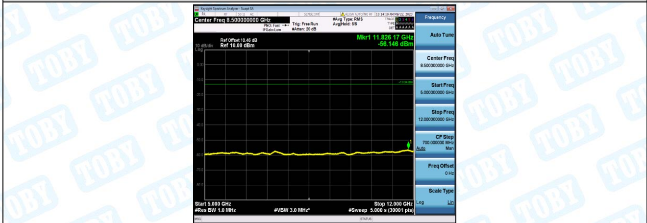
Band66-3MHz-16QAM-131987-1-0-Low-5000-12000--56.15-PASS
