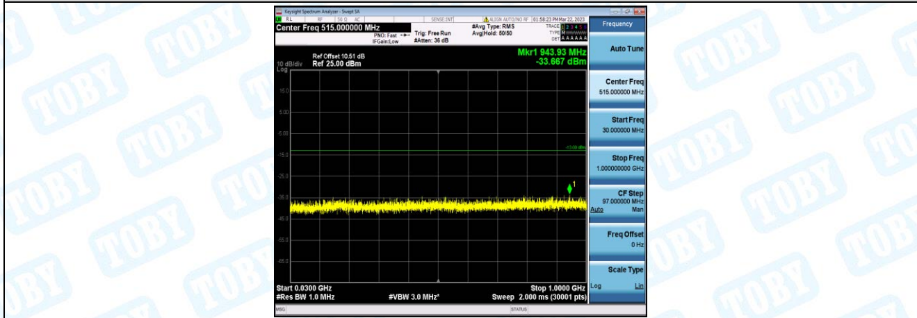
Band66-15MHz-QPSK-132322-1-0-Low-30-1000--33.67-PASS
