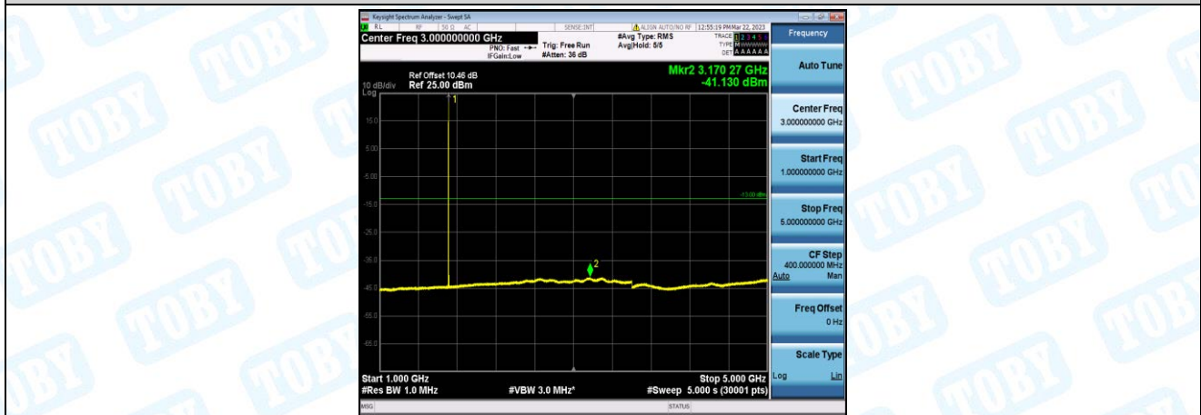
Band66-10MHz-QPSK-132022-1-0-Low-1000-5000--41.13-PASS
