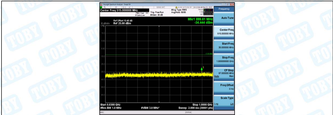
Band66-3MHz-16QAM-131987-1-0-Low-30-1000--34.44-PASS
