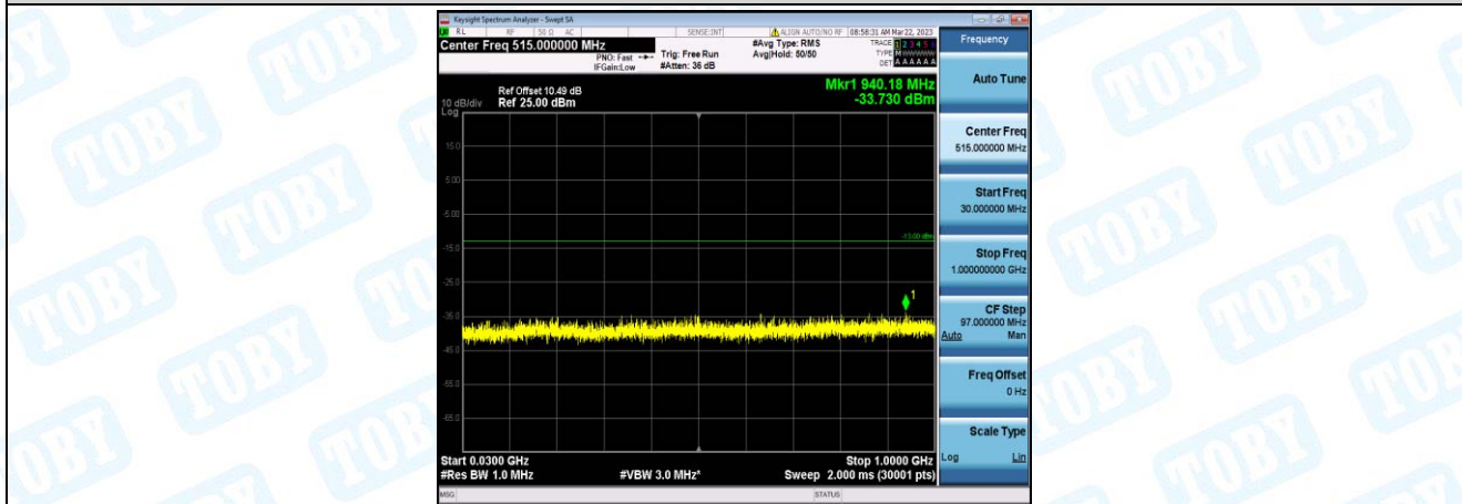
Band66-1.4MHz-16QAM-132665-1-0-High-30-1000--33.73-PASS
