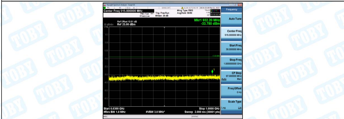
Band66-1.4MHz-16QAM-132322-1-0-Low-30-1000--33.78-PASS
