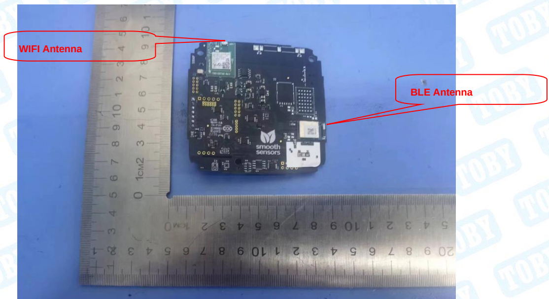
Photo 8 Appearance of PCB
