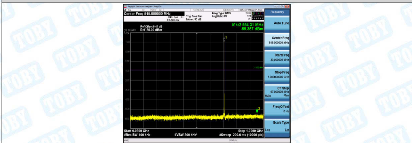
Band17-Stand-Alone-NaN-BPSK-23831-1@11-15kHz-30-1000-30~1000MHz@-59.36dBm--13-PASS
