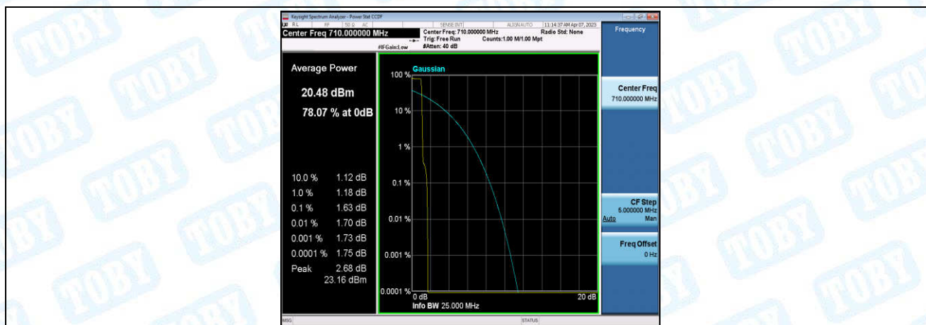
Band17-Stand-Alone-NaN-BPSK-23790-1@0-3.75kHz-1.63-<=13-PASS
