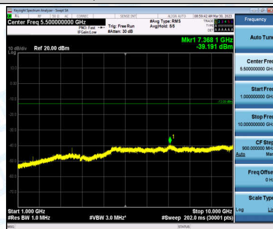
Band26-Stand-Alone-NaN-QPSK-26740-1@0-3.75kHz-1000-10000-1000-10000MHz@-39.19dBm--13-PASS
