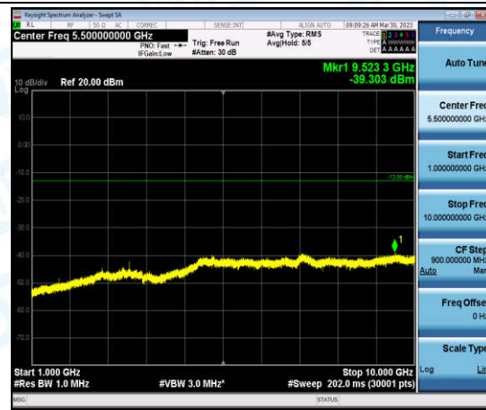
Band26-Stand-Alone-NaN-BPSK-26783-1@0-15kHz-1000-10000-1000-10000MHz@-39.3dBm--13-PASS
