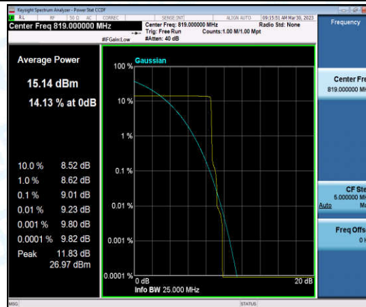
Band26-Stand-Alone-NaN-QPSK-26915-1@11-15kHz-9.01-<=13-PASS
