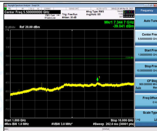
Band26-Stand-Alone-Na-N-QPSK-26783-1@47-3.75kHz-1000-10000-1000-10000MHz@-39.04dBm--13-PASS
