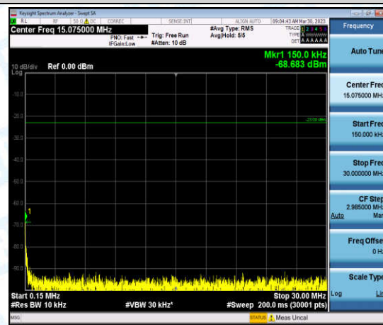
Band26-Stand-Alone-Na-N-QPSK-26783-12@0-15kHz-0.15-30-0.15-30MHz@-68.68dBm--23-PASS
