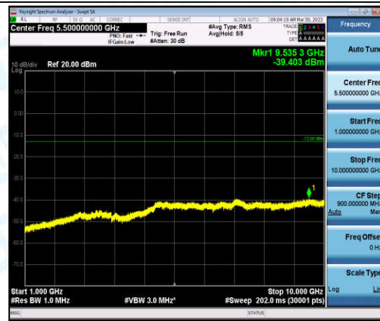
Band26-Stand-Alone-Na-N-QPSK-26740-12@0-15kHz-1000-10000-1000-10000MHz@-39.4dBm--13-PASS
