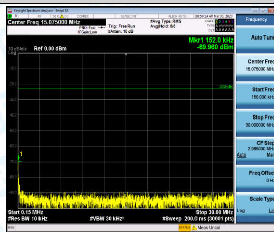
Band26-Stand-Alone-NaN-QPSK-26740-1@0-3.75kHz-0.15-30-0.15-30MHz@-69.96dBm--23-PASS
