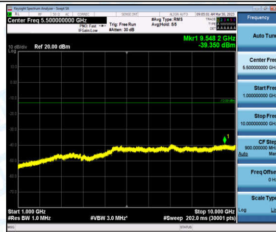
Band26-Stand-Alone-Na-N-QPSK-26783-12@0-15kHz-1000-10000-1000-10000MHz@-39.35dBm--13-PASS
