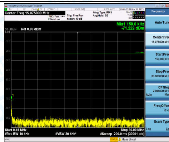
Band26-Stand-Alone-NaN-QPSK-26740-1@47-3.75kHz-0.15-30-0.15-30MHz@-71.22dBm--23-PASS
