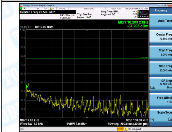
Band26-Stand-Alone-Na-N-QPSK-26783-12@0-15kHz-0.009-0.15-0.009-0.15MHz@-67.29dBm--33-PASS
