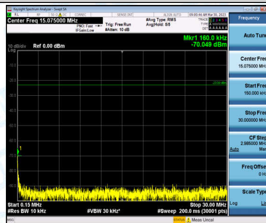
Band26-Stand-Alone-NaN-QPSK-26783-1@0-3.75kHz-0.15-30-0.15-30MHz@-70.05dBm--23-PASS
