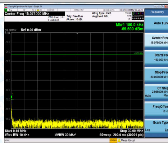
Band26-Stand-Alone-Na-N-QPSK-26783-1@47-3.75kHz-0.15-30-0.15-30MHz@-69.69dBm--23-PASS
