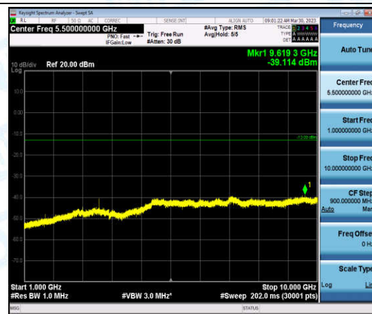
Band26-Stand-Alone-Na-N-QPSK-26783-1@0-3.75kHz-1000-10000-1000-10000MHz@-39.11dBm--13-PASS
