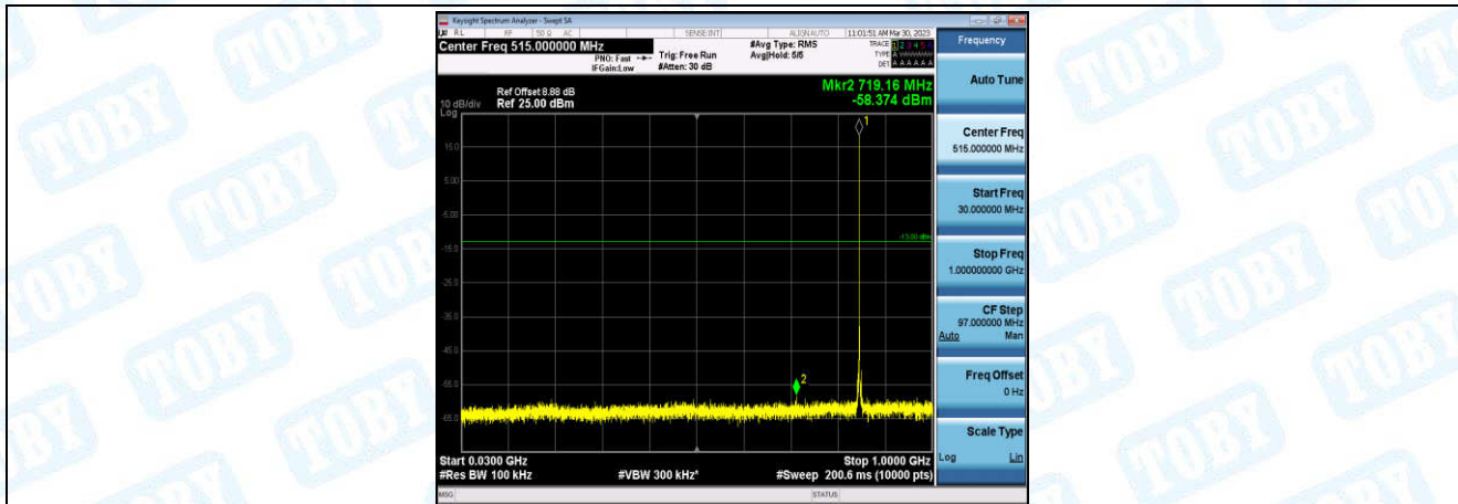
Band5-Stand-Alone-NaN-BPSK-20649-1@0-15kHz-30-1000-30~1000MHz@-58.37dBm--13-PASS
