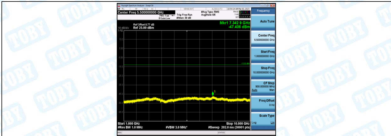
Band5-Stand-Alone-NaN-QPSK-20401-12@0-15kHz-1000-10000-1000~10000MHz@-47.41dBm--13-PASS
