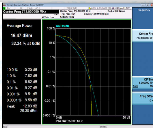
Band12-5MHz-QPSK-23155-6-0-High-8.82-<=13-PASS
