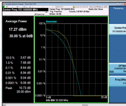
Band12-5MHz-QPSK-23095-1-0-Low-8.64-<=13-PASS
