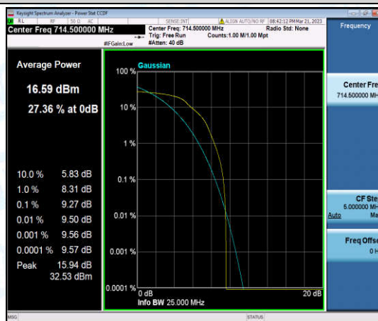
Band12-3MHz-QPSK-23165-1-0-High-9.27-<=13-PASS
