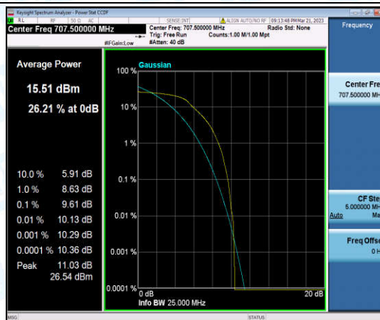
Band12-5MHz-16QAM-23095-6-0-Low-9.61-<=13-PASS
