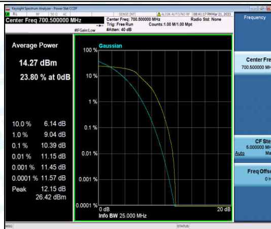
Band12-3MHz-16QAM-23025-6-0-Low-10.39-<=13-PASS
