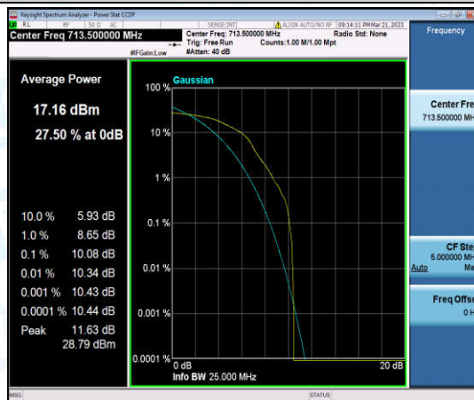
Band12-5MHz-16QAM-23155-1-0-High-10.08-<=13-PASS
