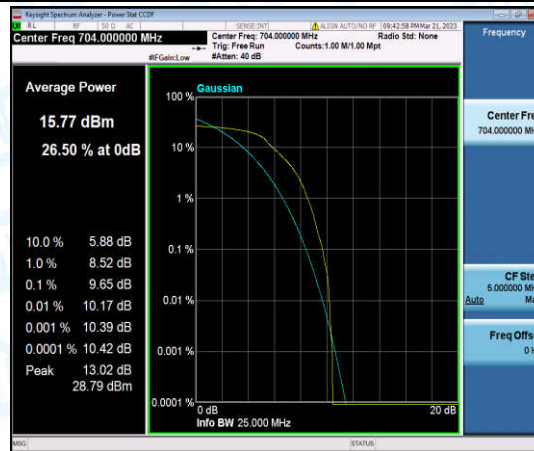
Band12-10MHz-16QAM-23060-6-0-Low-9.65-<=13-PASS
