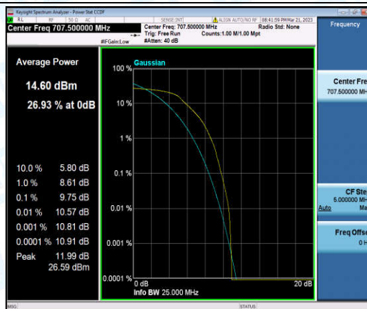
Band12-3MHz-16QAM-23095-6-0-Low-9.75-<=13-PASS
