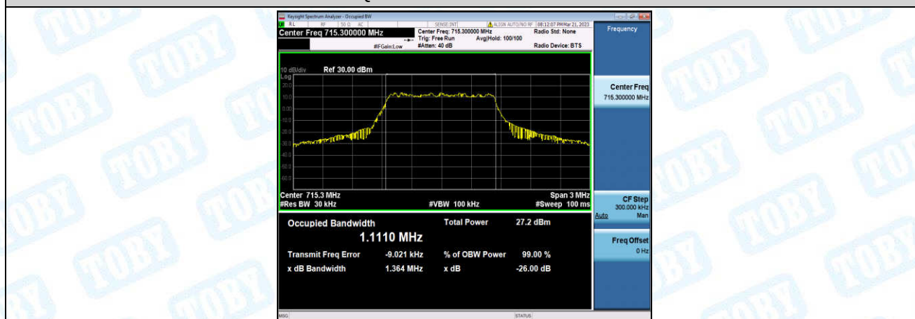
Band12-1.4MHz-QPSK-23173-6-0-High-1.1110-1.364-PASS
