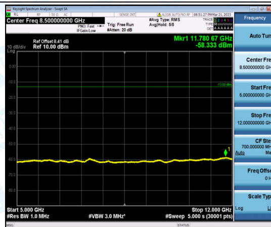
Band12-3MHz-QPSK-23095-1-0-Low-5000-12000--58.33-PASS
