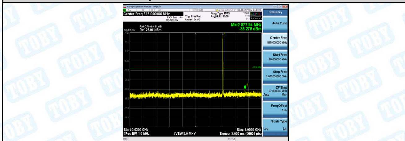
Band12-1.4MHz-QPSK-23173-1-0-High-30-1000--35.28-PASS
