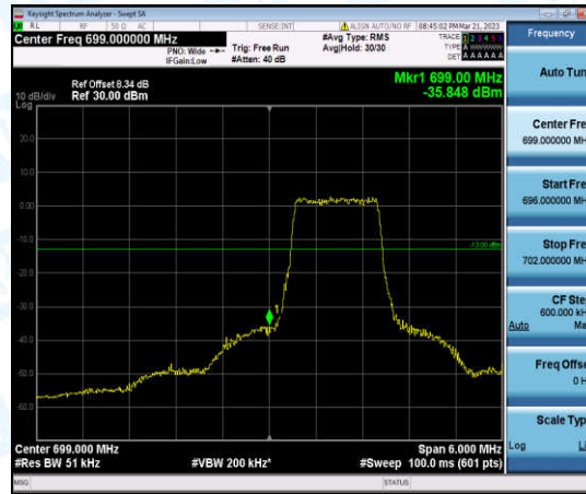
Band12-3MHz-QPSK-23025-6-0-Low--35.85-PASS
