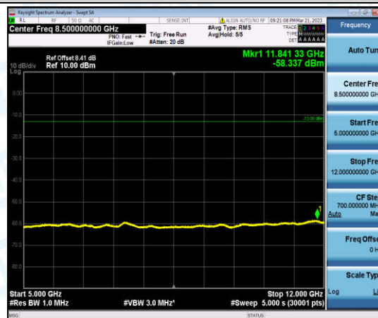
Band12-5MHz-16QAM-23035-1-0-Low-5000-12000--58.34-PASS
