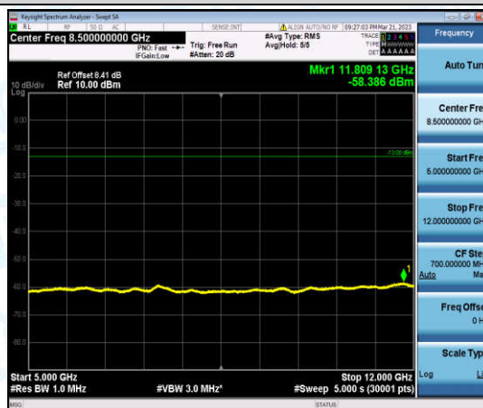
Band12-5MHz-QPSK-23155-1-0-High-5000-12000--58.39-PASS
