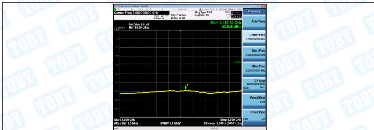
Band12-3MHz-16QAM-23165-1-0-High-1000-5000--43.05-PASS
