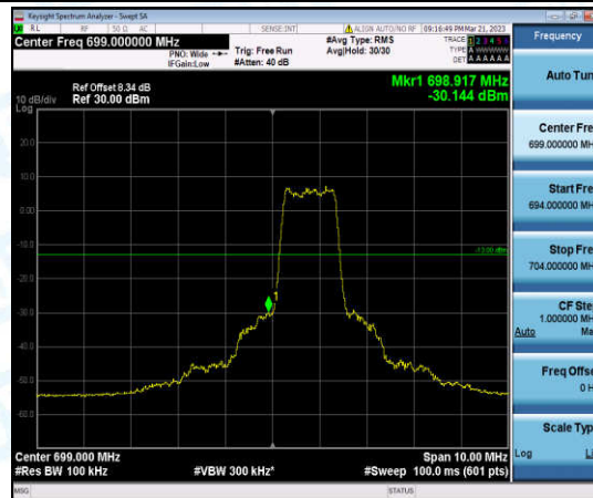
Band12-5MHz-QPSK-23035-6-0-Low--30.14-PASS
