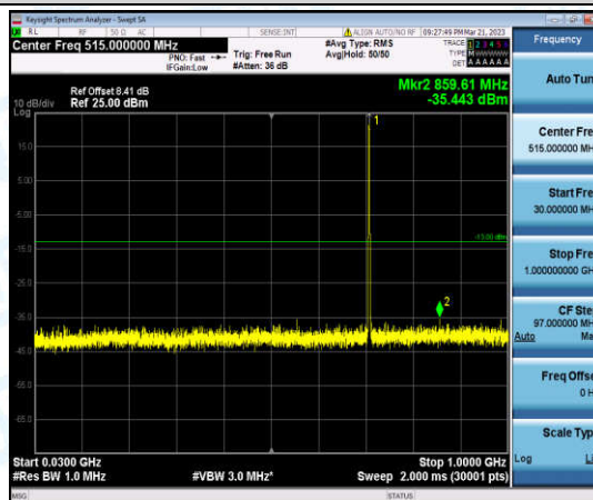
Band12-5MHz-16QAM-23155-1-0-High-30-1000--35.44-PASS
