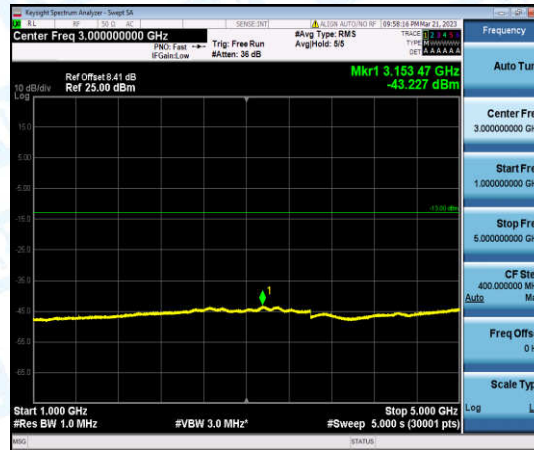
Band12-10MHz-16QAM-23130-1-0-High-1000-5000--43.23-PASS
