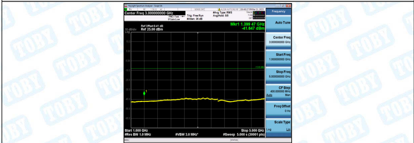
Band12-10MHz-QPSK-23060-1-0-Low-1000-5000--41.65-PASS
