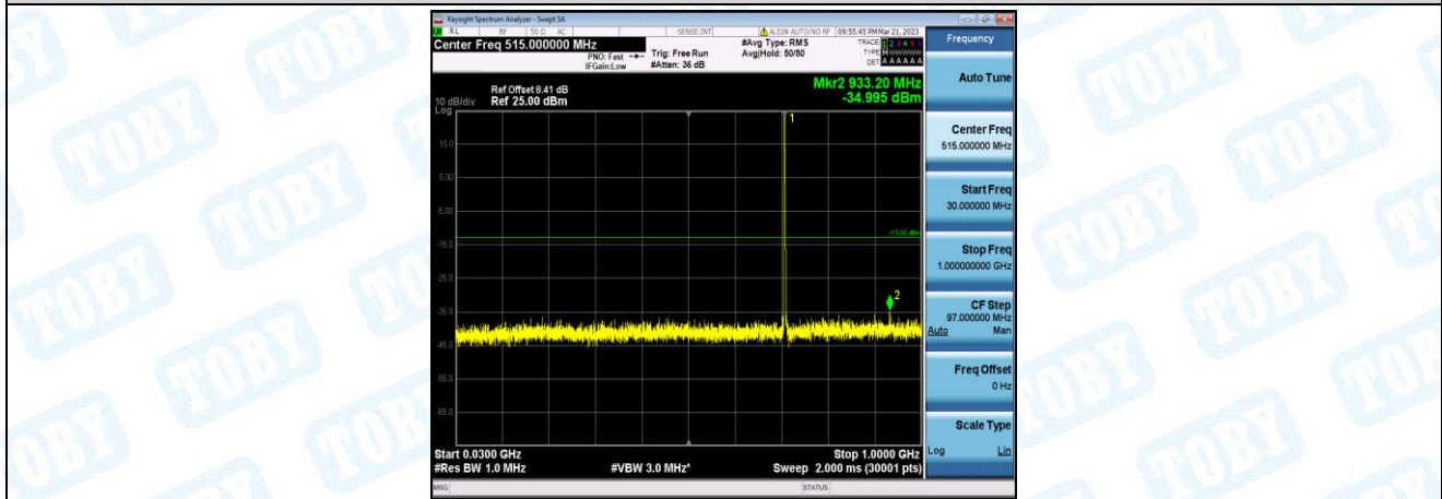
Band12-10MHz-QPSK-23130-1-0-High-30-1000--35-PASS
