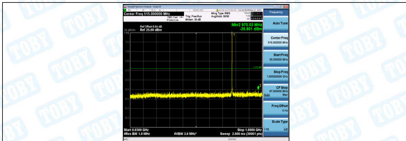
Band13-5MHz-16QAM-23205-1-0-Low-30-1000--35.8-PASS
