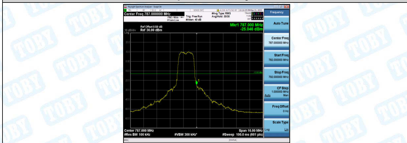
Band13-5MHz-16QAM-23255-6-0-High--25.05-PASS
