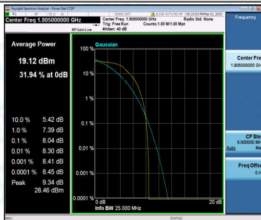
Band2-15MHz-16QAM-19150-6-0-High-8.04-<=13-PASS
