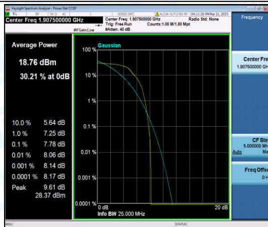
Band2-5MHz-QPSK-19175-1-0-High-7.78-<=13-PASS
