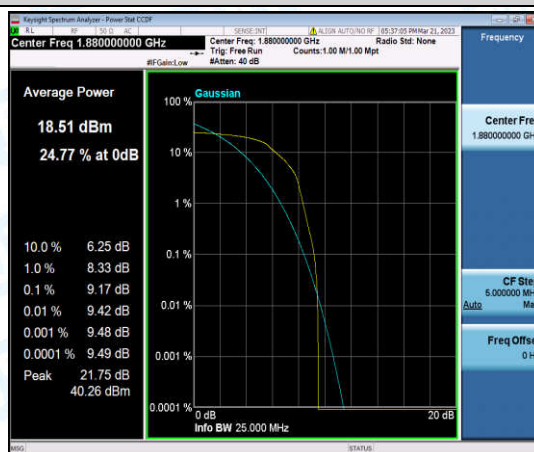
Band2-20MHz-QPSK-18900-1-0-Low-9.17-<=13-PASS
