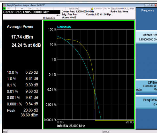
Band2-15MHz-QPSK-19150-6-0-High-9.39-<=13-PASS
