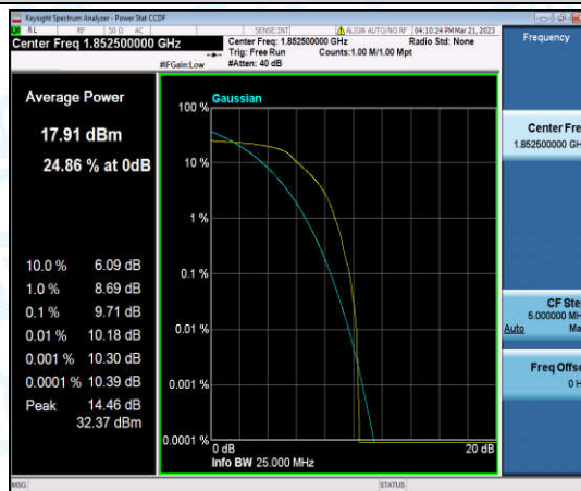
Band2-5MHz-QPSK-18625-6-0-Low-9.71-<=13-PASS
