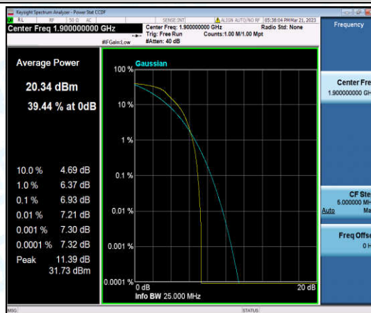
Band2-20MHz-QPSK-19100-6-0-High-6.93-<=13-PASS
