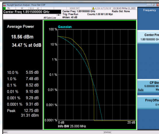
Band2-3MHz-16QAM-18615-6-0-Low-8.52-<=13-PASS
