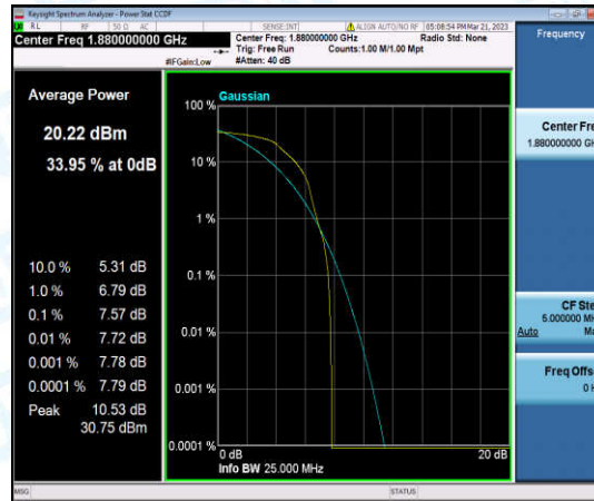
Band2-15MHz-QPSK-18900-1-0-Low-7.57-<=13-PASS
