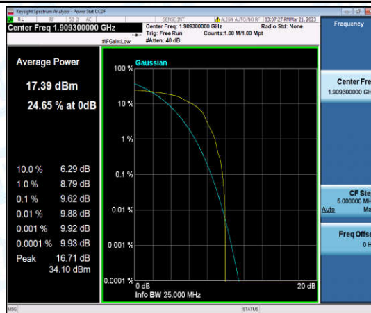
Band2-1.4MHz-16QAM-19193-1-0-High-9.62-<=13-PASS
