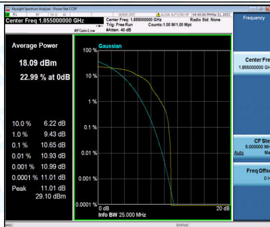
Band2-10MHz-16QAM-18650-1-0-Low-10.65-<=13-PASS
