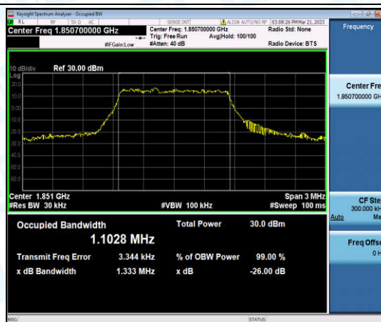
Band2-1.4MHz-16QAM-18507-6-0-Low-1.1028-1.333-PASS
