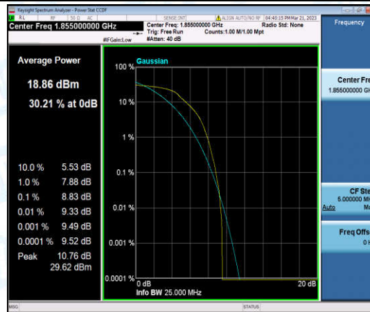
Band2-10MHz-QPSK-18650-6-0-Low-8.83-<=13-PASS
