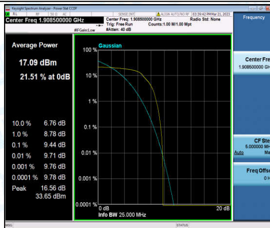
Band2-3MHz-QPSK-19185-1-0-High-9.44-<=13-PASS
