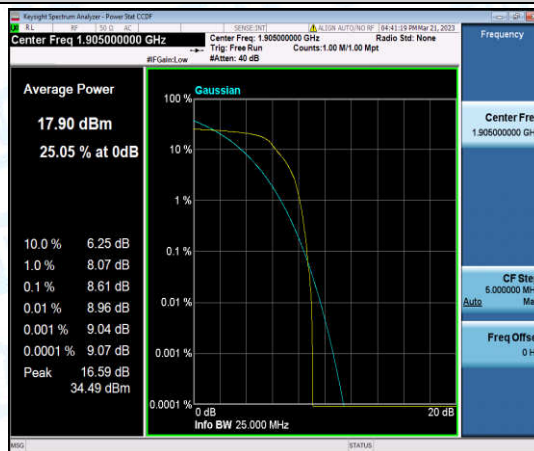
Band2-10MHz-QPSK-19150-1-0-High-8.61-<=13-PASS
