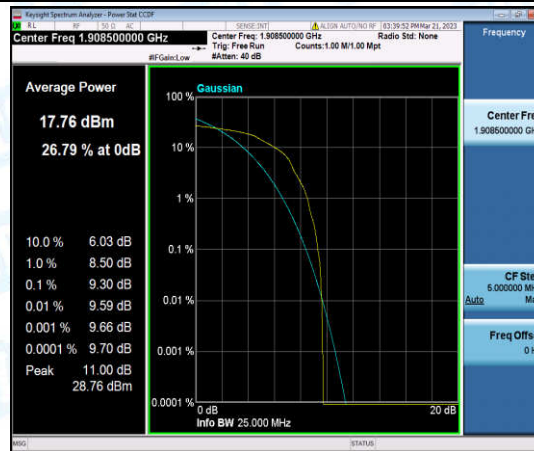
Band2-3MHz-16QAM-19185-1-0-High-9.30-<=13-PASS
