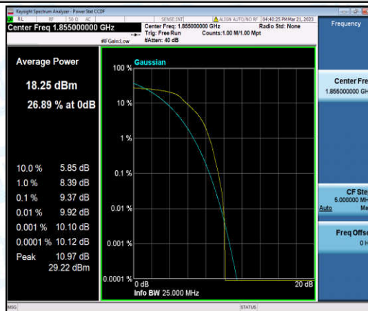
Band2-10MHz-16QAM-18650-6-0-Low-9.37-<=13-PASS
