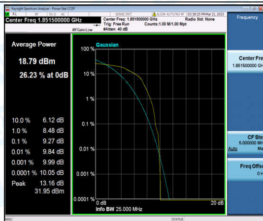
Band2-3MHz-16QAM-18615-1-0-Low-9.27-<=13-PASS
