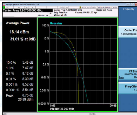
Band2-5MHz-16QAM-19175-6-0-High-8.12-<=13-PASS
