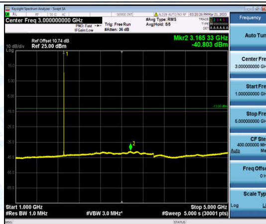
Band2-1.4MHz-QPSK-19193-1-0-High-1000-5000--40.8-PASS
