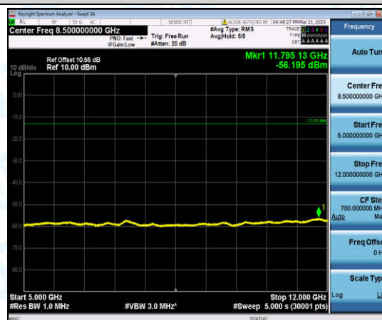
Band2-10MHz-16QAM-18650-1-0-Low-5000-12000--56.2-PASS
