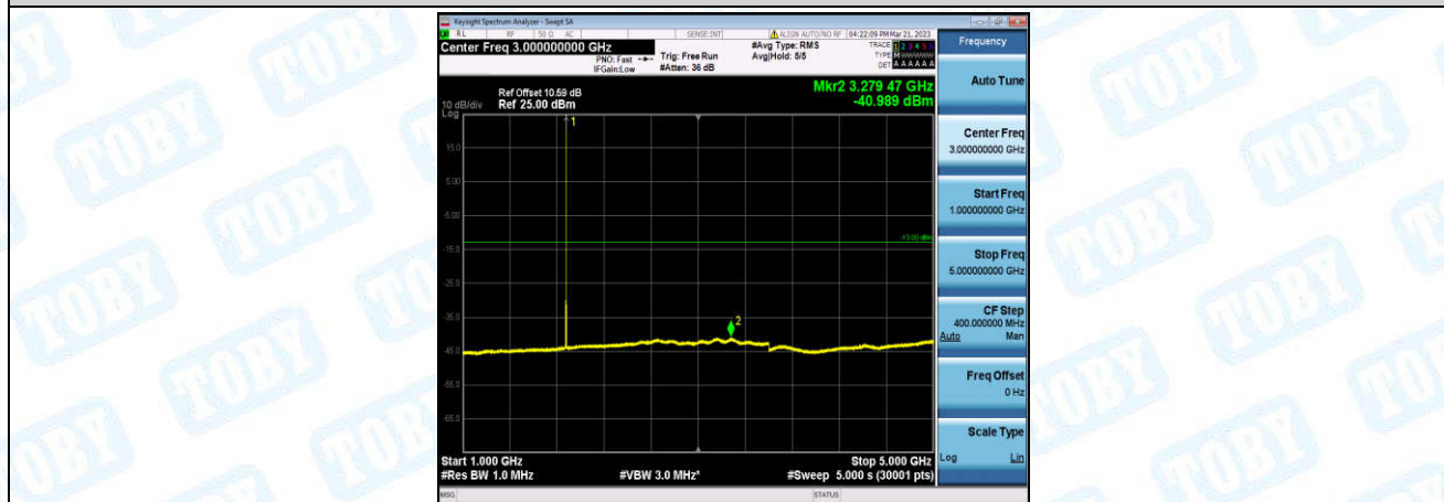
Band2-5MHz-16QAM-18900-1-0-Low-1000-5000--40.99-PASS
