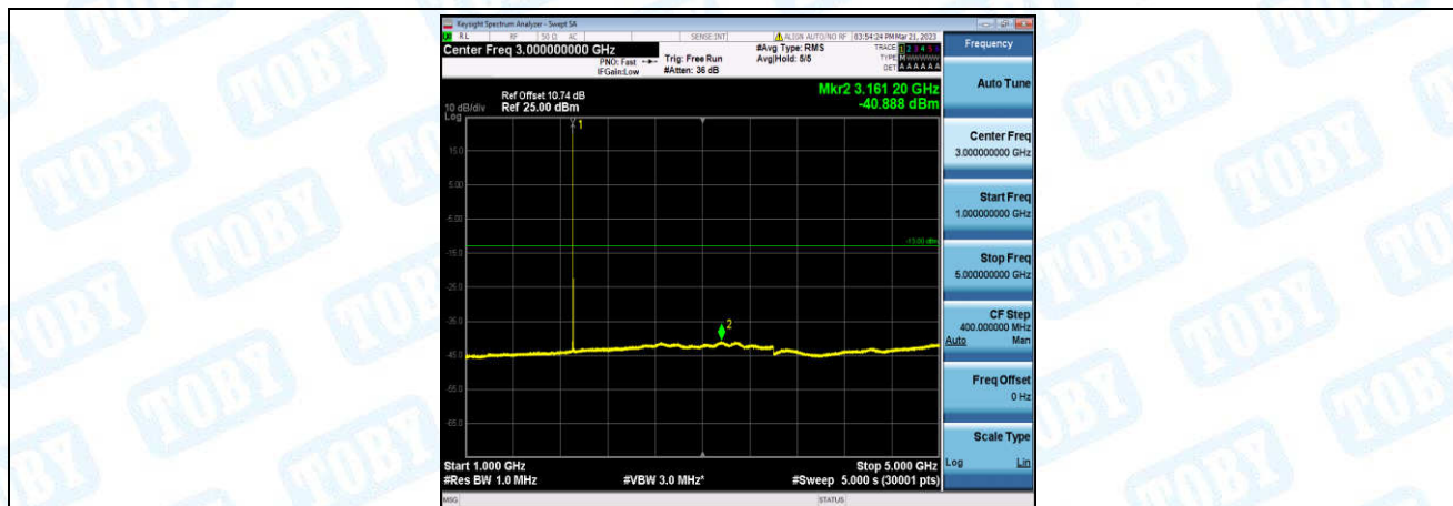
Band2-3MHz-16QAM-19185-1-0-High-1000-5000--40.89-PASS
