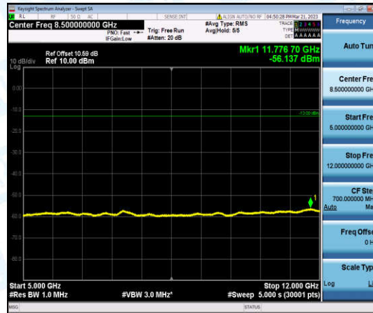
Band2-10MHz-QPSK-18900-1-0-Low-5000-12000--56.14-PASS
