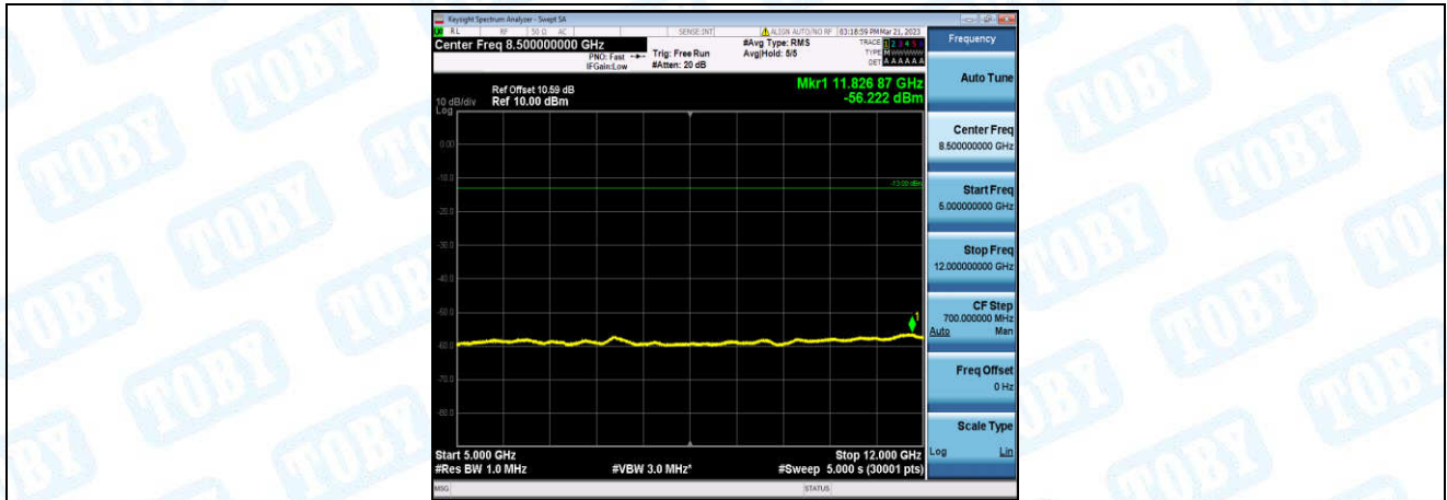
Band2-1.4MHz-16QAM-18900-1-0-Low-5000-12000--56.22-PASS
