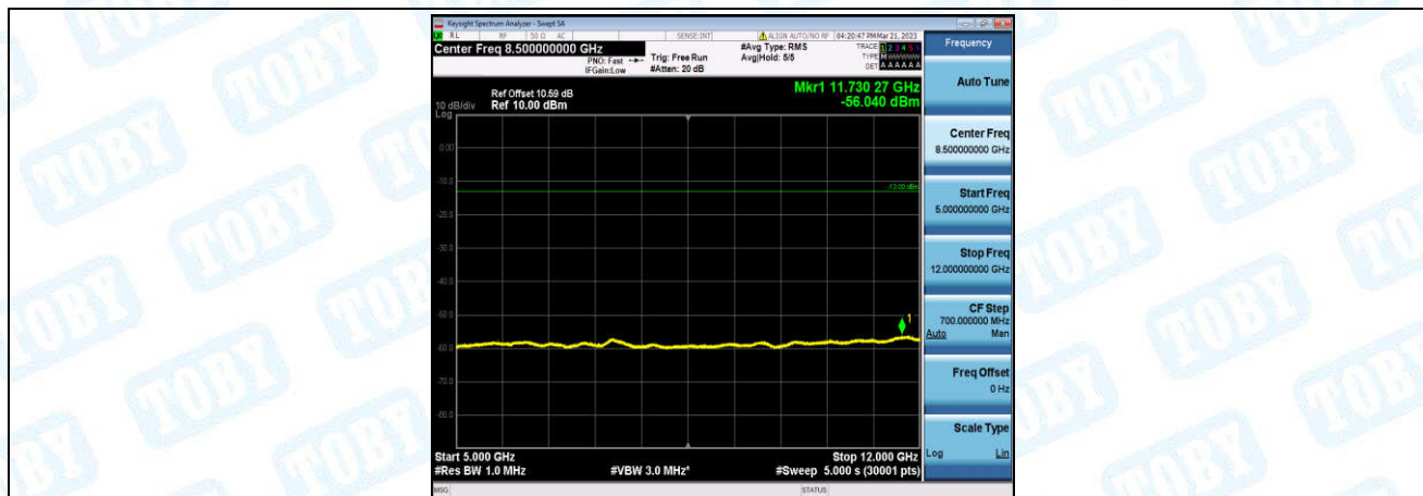
Band2-5MHz-QPSK-18900-1-0-Low-5000-12000--56.04-PASS
