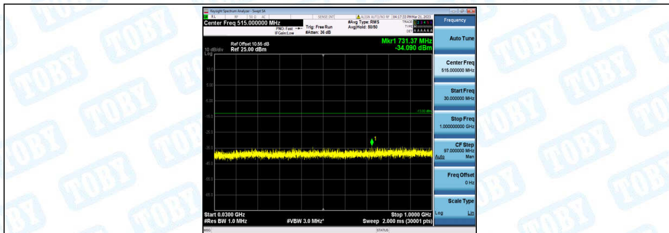
Band2-5MHz-16QAM-18625-1-0-Low-30-1000--34.09-PASS
