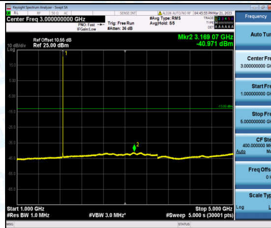
Band2-10MHz-QPSK-18650-1-0-Low-1000-5000--40.97-PASS
