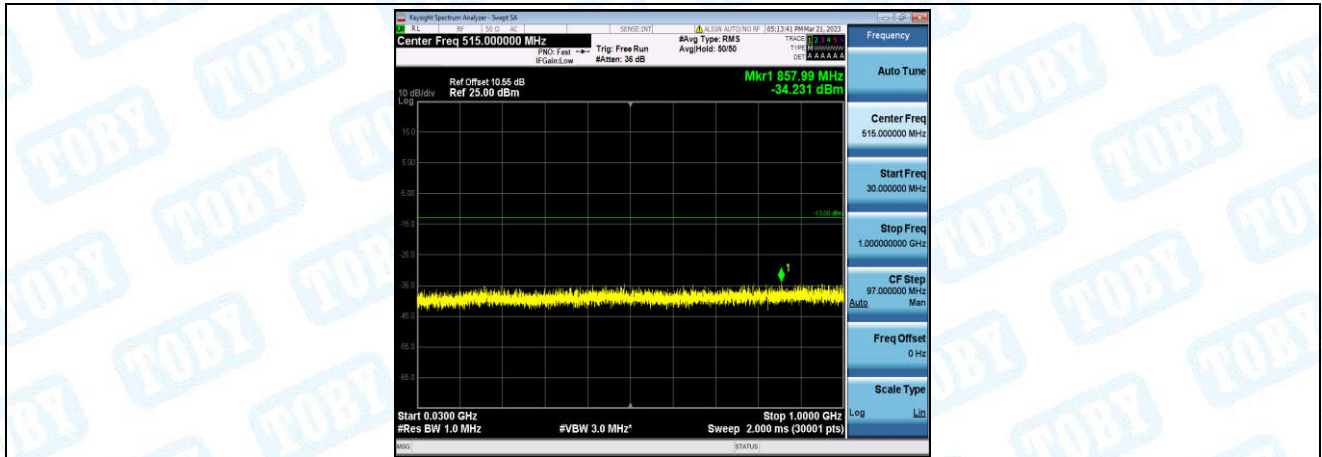
Band2-15MHz-QPSK-18675-1-0-Low-30-1000--34.23-PASS
