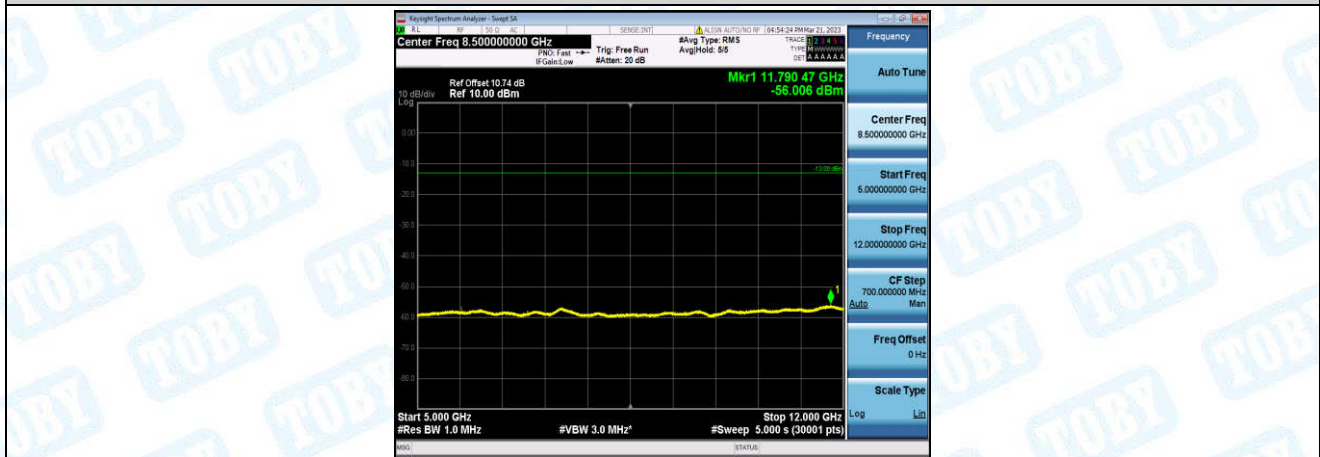
Band2-10MHz-QPSK-19150-1-0-High-5000-12000--56.01-PASS
