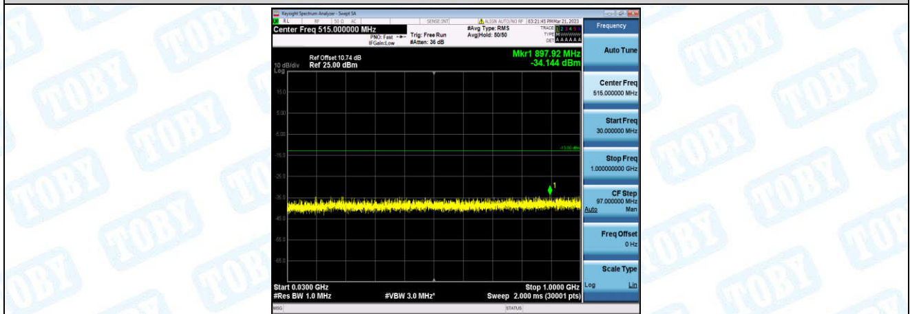
Band2-1.4MHz-16QAM-19193-1-0-High-30-1000--34.14-PASS
