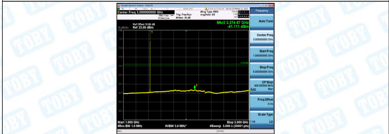
Band2-5MHz-QPSK-18625-1-0-Low-1000-5000--41.11-PASS
