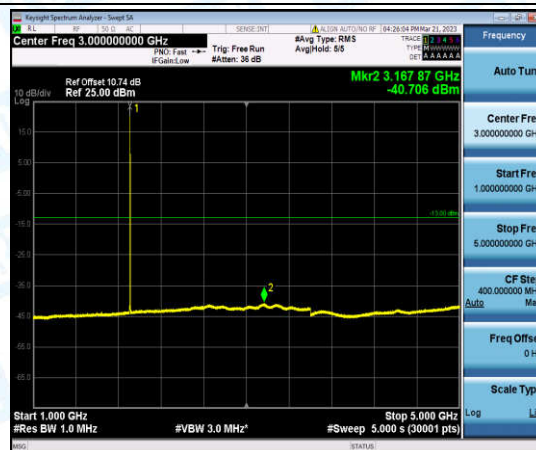
Band2-5MHz-16QAM-19175-1-0-High-1000-5000--40.71-PASS
