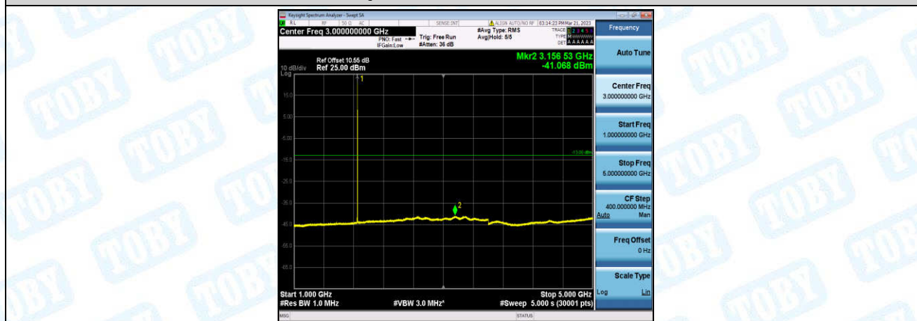
Band2-1.4MHz-16QAM-18607-1-0-Low-1000-5000--41.07-PASS
