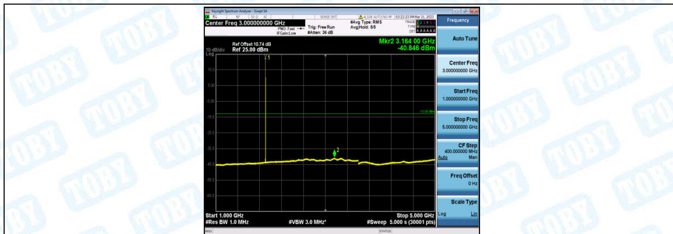
Band2-1.4MHz-16QAM-19193-1-0-High-1000-5000--40.85-PASS
