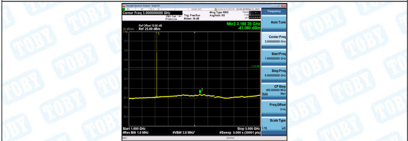
Band2-3MHz-QPSK-18615-1-0-Low-1000-5000--41.08-PASS
