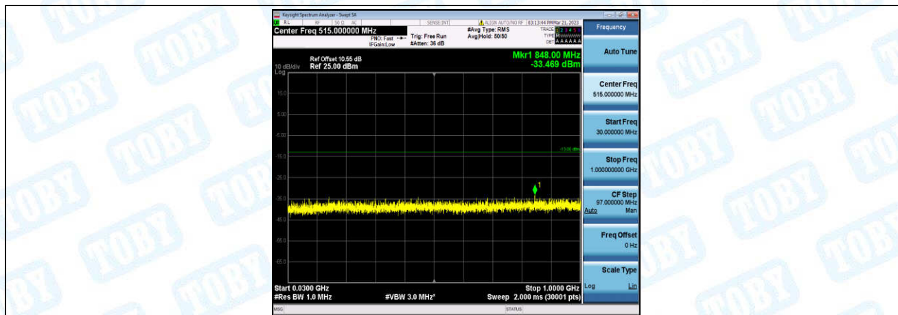
Band2-1.4MHz-16QAM-18607-1-0-Low-30-1000--33.47-PASS
