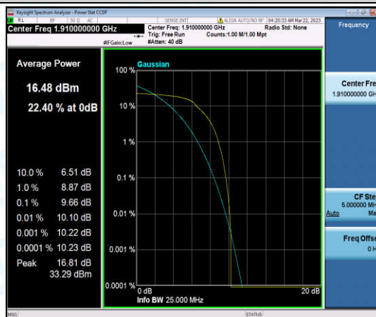
Band25-10MHz-QPSK-26640-6-0-High-9.66-<=13-PASS
