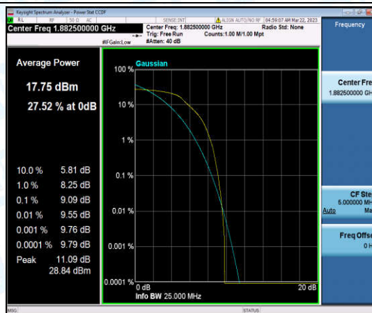
Band25-10MHz-QPSK-26365-6-0-Low-9.09-<=13-PASS
