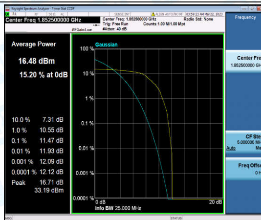
Band25-5MHz-QPSK-26065-1-0-Low-11.47-<=13-PASS
