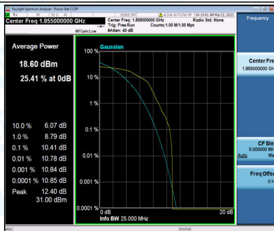
Band25-10MHz-16QAM-26090-1-0-Low-10.41-<=13-PASS
