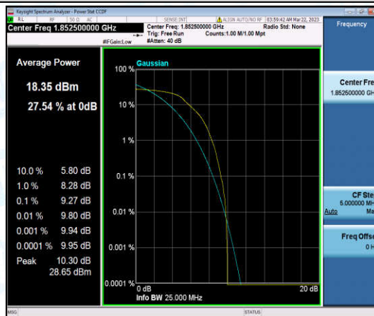
Band25-5MHz-QPSK-26065-6-0-Low-9.27-<=13-PASS
