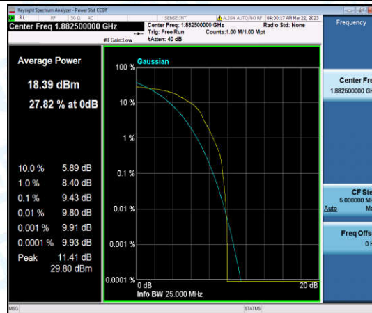
Band25-5MHz-16QAM-26365-1-0-Low-9.43-<=13-PASS
