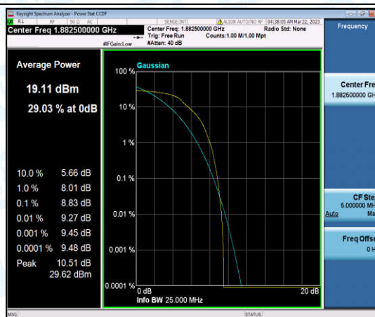
Band25-15MHz-16QAM-26365-6-0-Low-8.83-<=13-PASS
