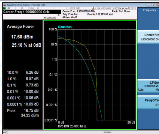
Band25-20MHz-16QAM-26590-1-0-High-9.73-<=13-PASS
