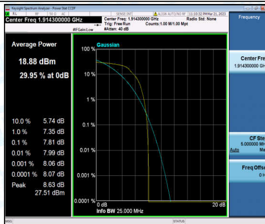
Band25-1.4MHz-QPSK-26683-1-0-High-7.81-<=13-PASS
