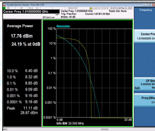
Band25-10MHz-QPSK-26640-1-0-High-8.85-<=13-PASS
