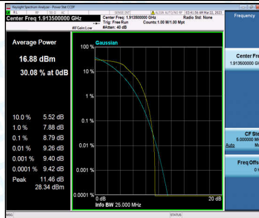
Band25-3MHz-QPSK-26675-6-0-High-8.79-<=13-PASS
