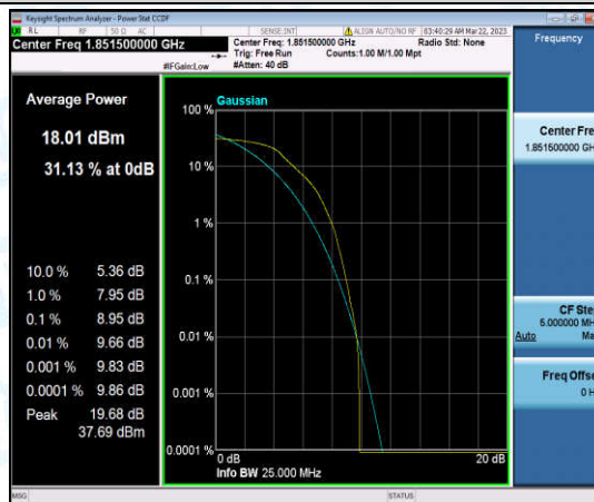
Band25-3MHz-QPSK-26055-6-0-Low-8.95-<=13-PASS
