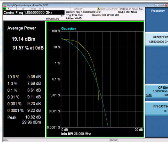
Band25-10MHz-16QAM-26090-6-0-Low-8.61-<=13-PASS
