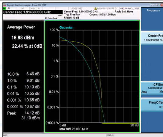
Band25-1.4MHz-16QAM-26683-1-0-High-10.13-<=13-PASS
