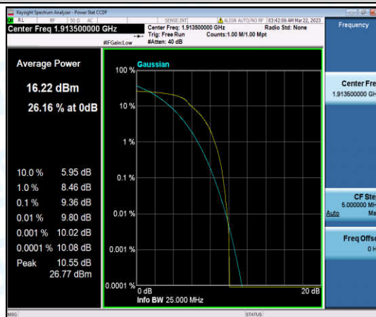
Band25-3MHz-16QAM-26675-6-0-High-9.36-<=13-PASS
