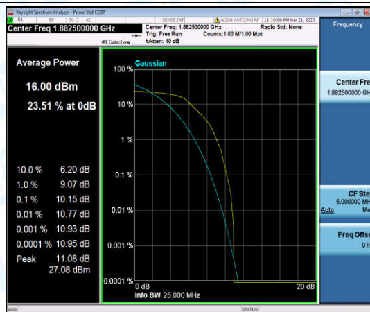
Band25-1.4MHz-QPSK-26365-6-0-Low-10.15-<=13-PASS
