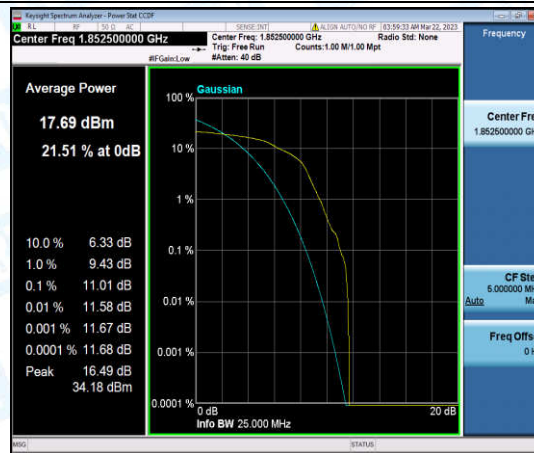
Band25-5MHz-16QAM-26065-1-0-Low-11.01-<=13-PASS
