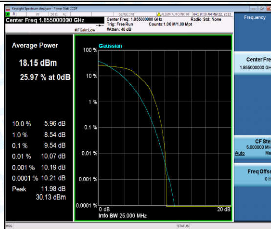
Band25-10MHz-QPSK-26090-6-0-Low-9.54-<=13-PASS
