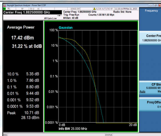
Band25-1.4MHz-16QAM-26365-6-0-Low-8.80-<=13-PASS
