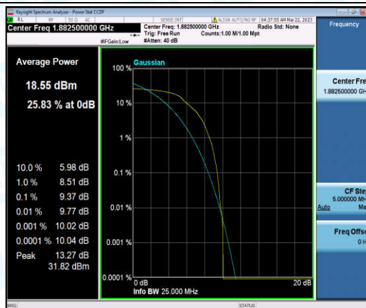
Band25-15MHz-QPSK-26365-6-0-Low-9.37-<=13-PASS
