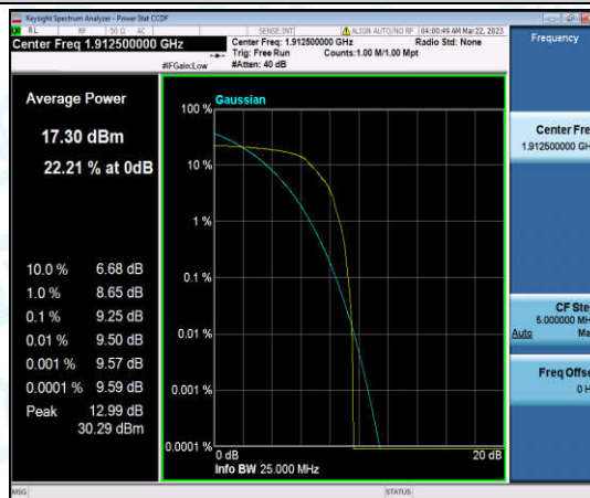
Band25-5MHz-QPSK-26665-1-0-High-9.25-<=13-PASS
