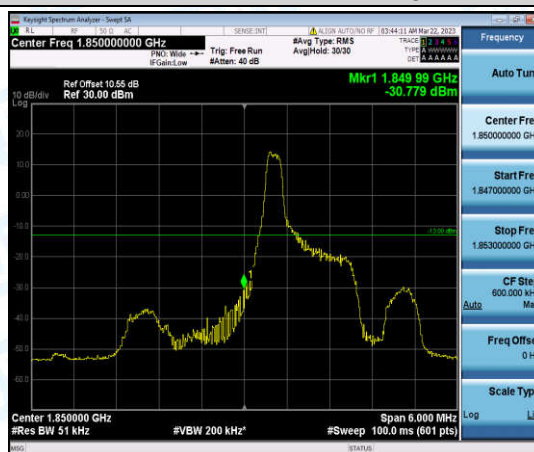
Band25-3MHz-QPSK-26055-1-0-Low--30.78-PASS
