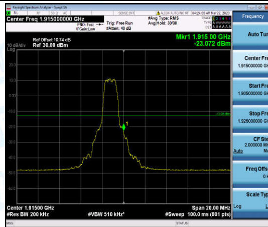
Band25-10MHz-16QAM-26640-6-0-High--23.07-PASS
