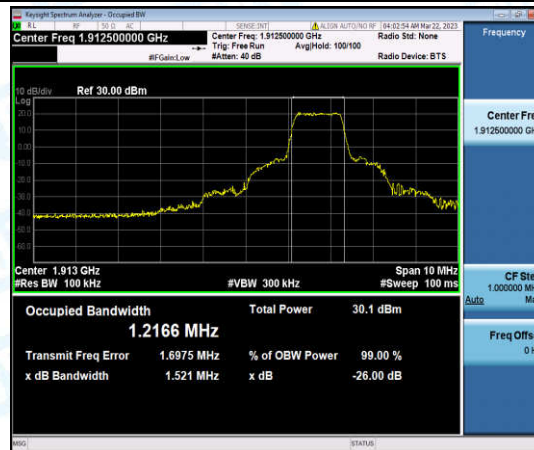
Band25-5MHz-QPSK-26665-6-0-High-1.2166-1.521-PASS
