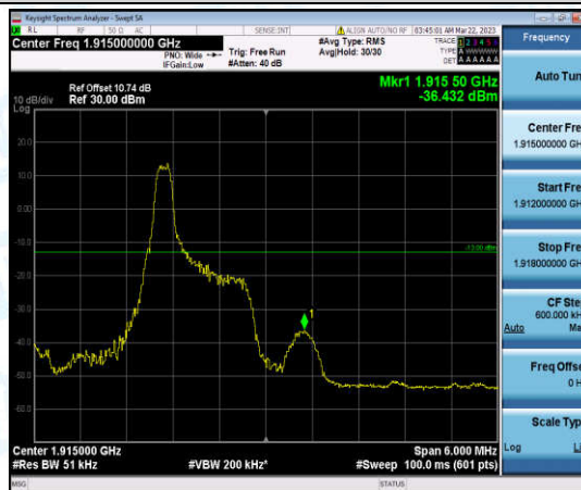
Band25-3MHz-QPSK-26675-1-0-High--36.43-PASS
