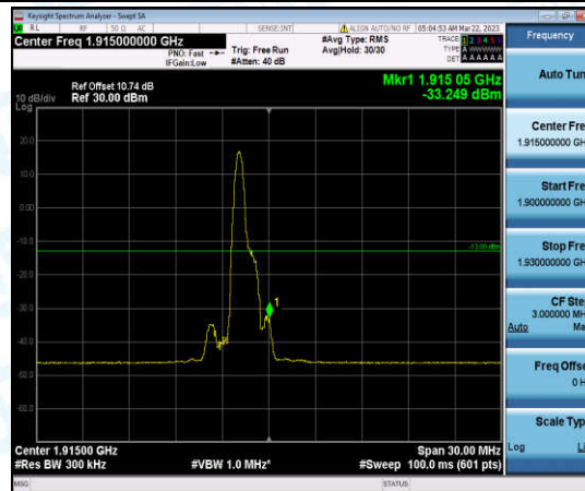
Band25-15MHz-16QAM-26615-1-0-High--33.25-PASS
