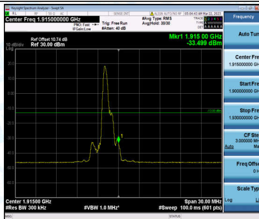
Band25-15MHz-QPSK-26615-1-0-High--33.50-PASS
