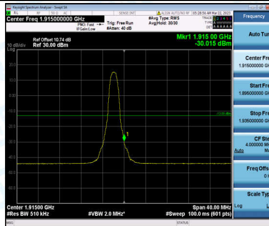
Band25-20MHz-16QAM-26590-6-0-High--30.01-PASS
