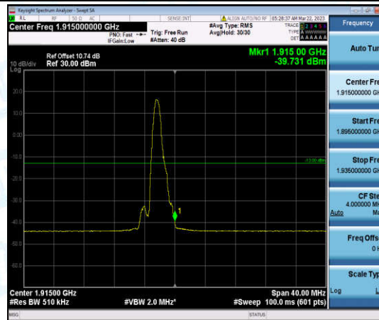
Band25-20MHz-16QAM-26590-1-0-High--39.73-PASS
