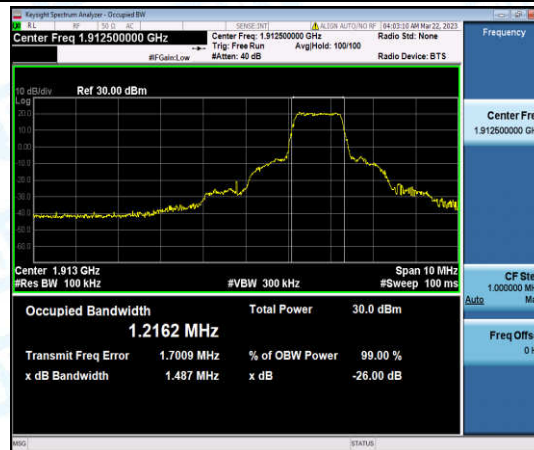
Band25-5MHz-16QAM-26665-6-0-High-1.2162-1.487-PASS
