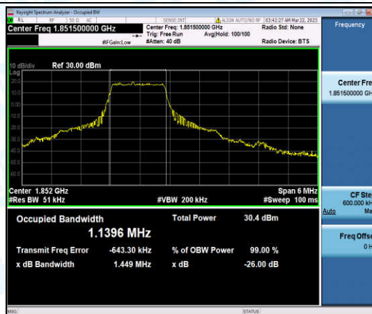
Band25-3MHz-QPSK-26055-6-0-Low-1.1396-1.449-PASS
