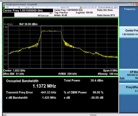
Band25-3MHz-16QAM-26055-6-0-Low-1.1372-1.425-PASS
