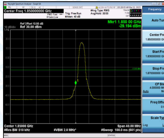
Band25-20MHz-16QAM-26140-6-0-Low--29.19-PASS
