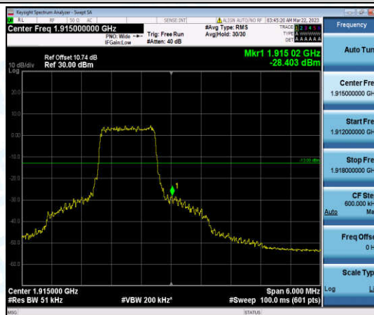
Band25-3MHz-QPSK-26675-6-0-High--28.40-PASS
