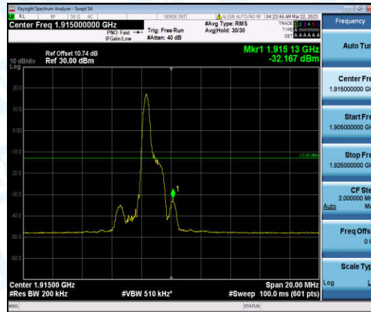
Band25-10MHz-16QAM-26640-1-0-High--32.17-PASS
