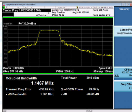
Band25-3MHz-16QAM-26365-6-0-Low-1.1467-1.566-PASS
