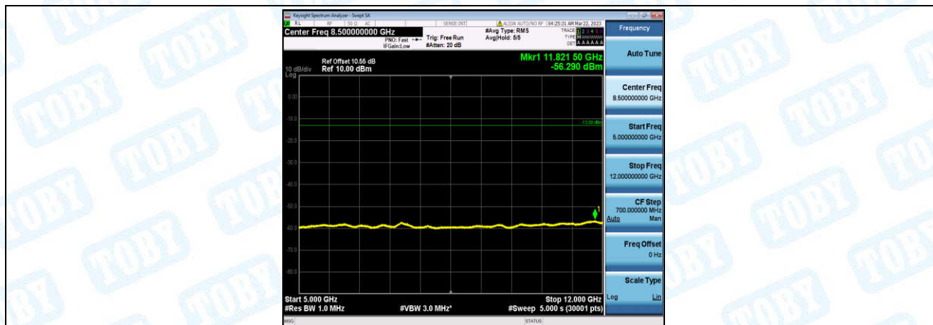
Band25-10MHz-QPSK-26090-1-0-Low-5000-12000--56.29-PASS
