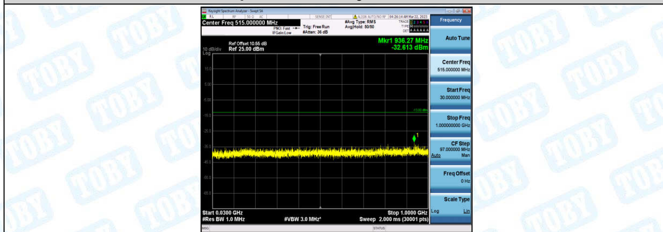
Band25-10MHz-16QAM-26090-1-0-Low-30-1000--32.61-PASS
