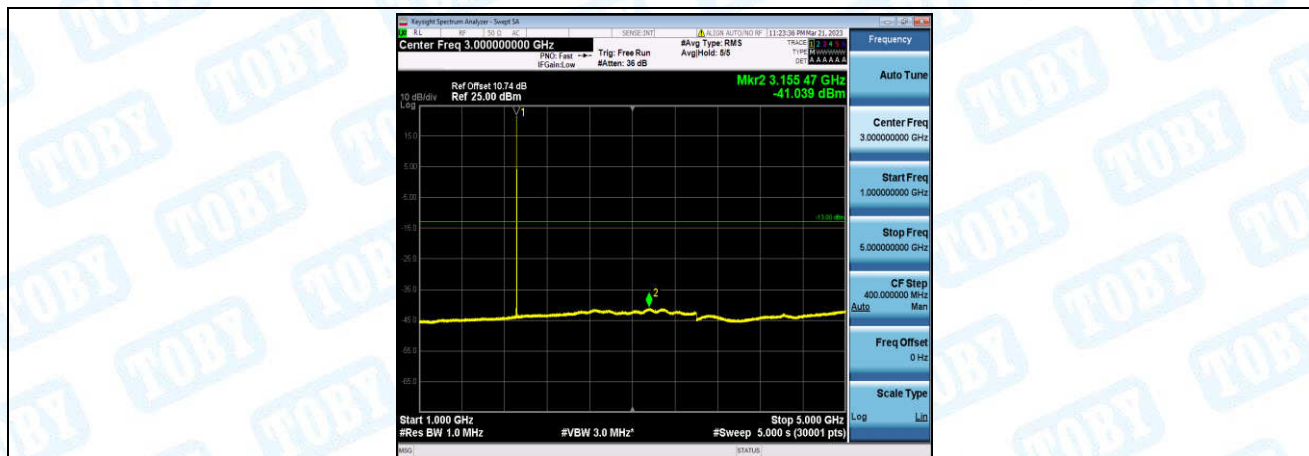
Band25-1.4MHz-QPSK-26683-1-0-High-1000-5000--41.04-PASS
