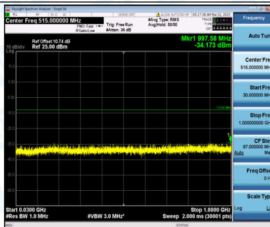
Band25-15MHz-QPSK-26615-1-0-High-30-1000--34.17-PASS
