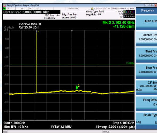
Band25-5MHz-16QAM-26365-1-0-Low-1000-5000--41.12-PASS
