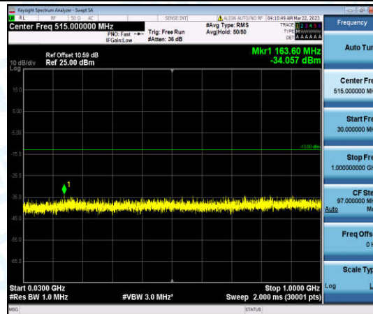
Band25-5MHz-16QAM-26365-1-0-Low-30-1000--34.06-PASS
