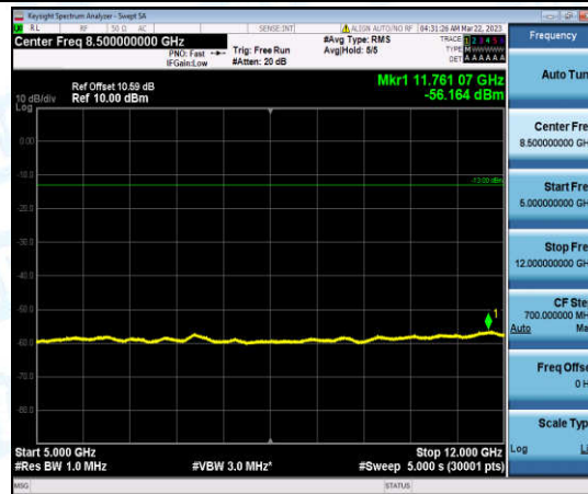
Band25-10MHz-16QAM-26365-1-0-Low-5000-12000--56.16-PASS
