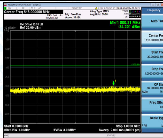
Band25-5MHz-16QAM-26665-1-0-High-30-1000--34.2-PASS
