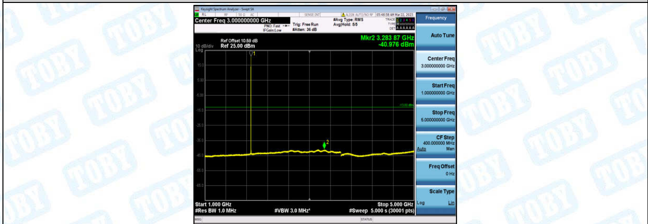
Band25-3MHz-16QAM-26365-1-0-Low-1000-5000--40.98-PASS
