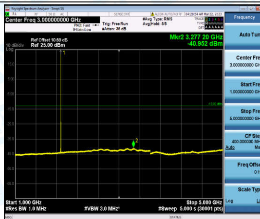
Band25-10MHz-QPSK-26365-1-0-Low-1000-5000--40.95-PASS
