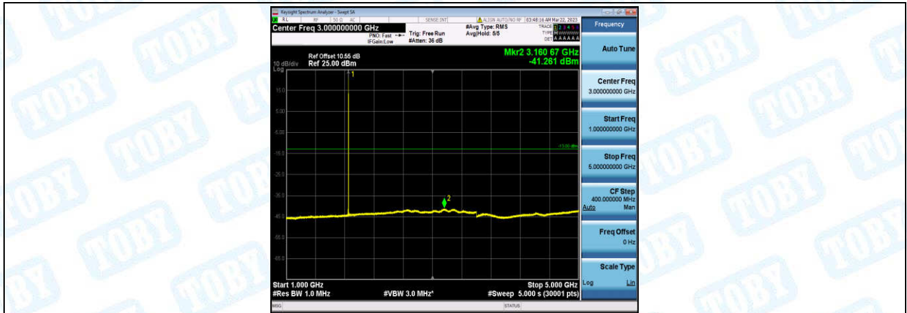
Band25-3MHz-16QAM-26055-1-0-Low-1000-5000--41.26-PASS
