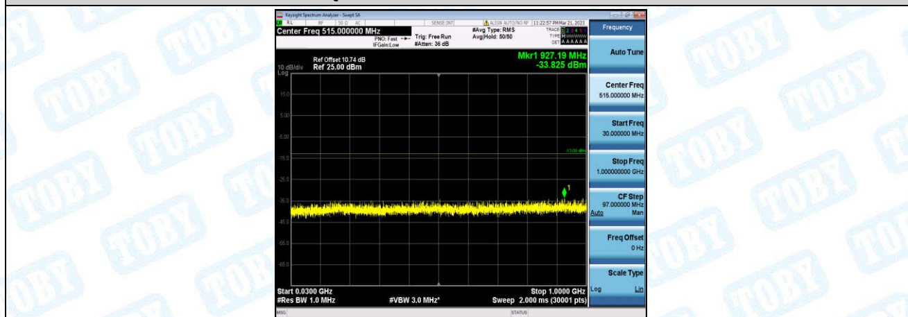
Band25-1.4MHz-QPSK-26683-1-0-High-30-1000--33.83-PASS
