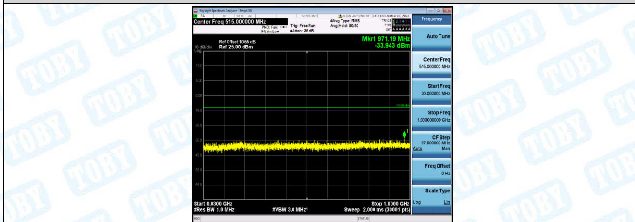
Band25-5MHz-QPSK-26065-1-0-Low-30-1000--33.94-PASS
