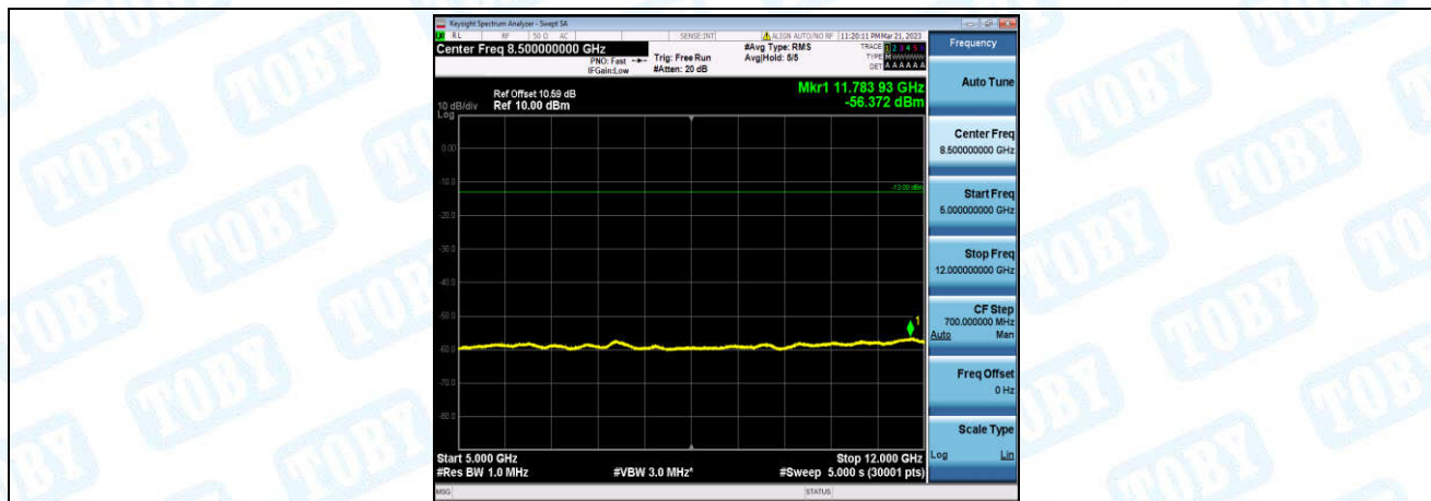
Band25-1.4MHz-QPSK-26365-1-0-Low-5000-12000--56.37-PASS
