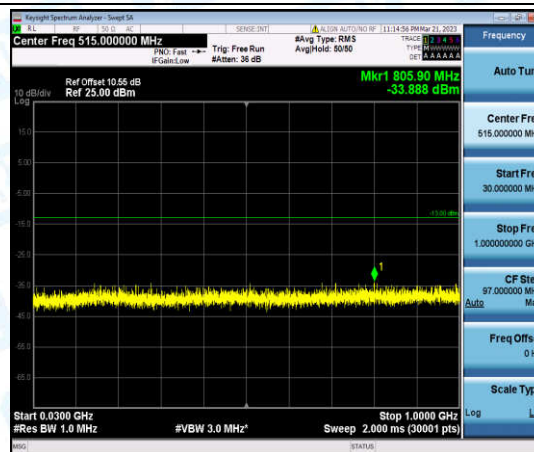
Band25-1.4MHz-QPSK-26047-1-0-Low-30-1000--33.89-PASS
