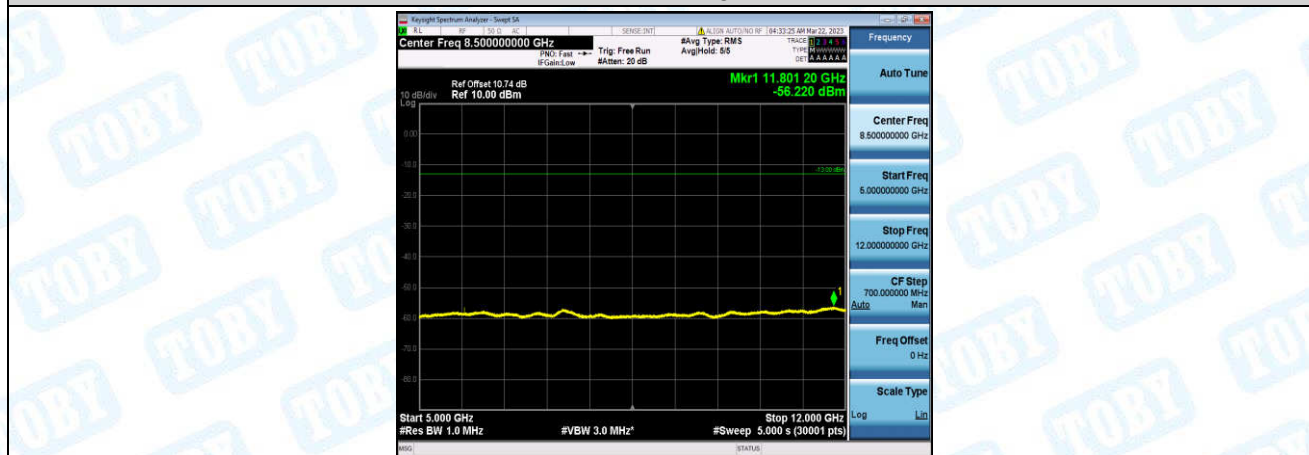
Band25-10MHz-QPSK-26640-1-0-High-5000-12000--56.22-PASS
