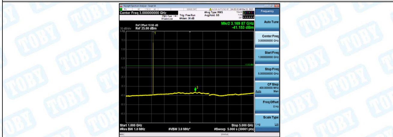
Band25-5MHz-QPSK-26065-1-0-Low-1000-5000--41.15-PASS
