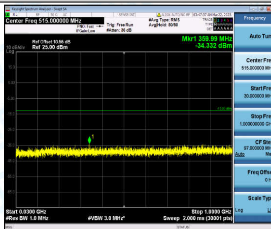
Band25-3MHz-16QAM-26055-1-0-Low-30-1000--34.33-PASS
