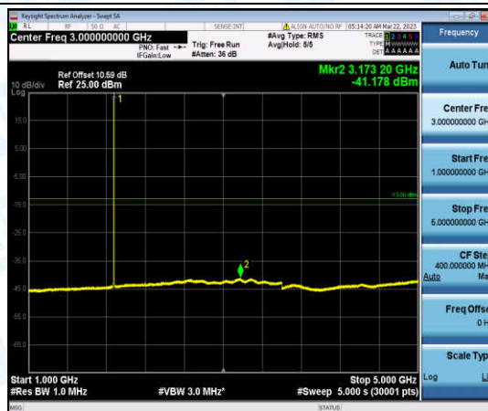
Band25-15MHz-QPSK-26365-1-0-Low-1000-5000--41.18-PASS
