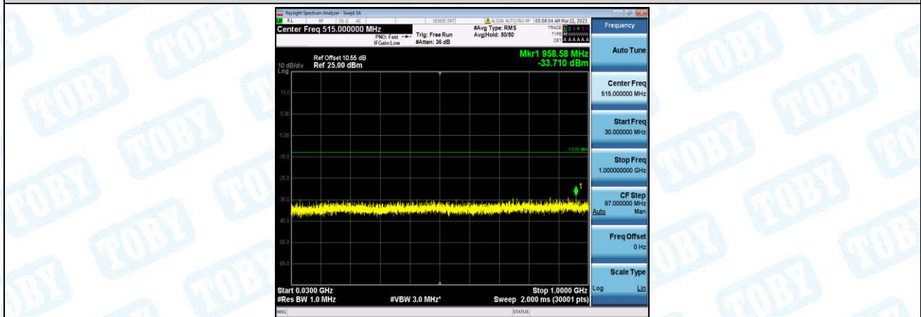
Band25-15MHz-QPSK-26115-1-0-Low-30-1000--33.71-PASS
