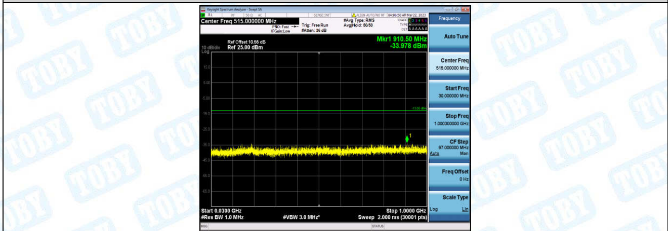
Band25-5MHz-16QAM-26065-1-0-Low-30-1000--33.98-PASS
