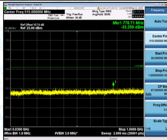
Band25-1.4MHz-16QAM-26683-1-0-High-30-1000--33.26-PASS
