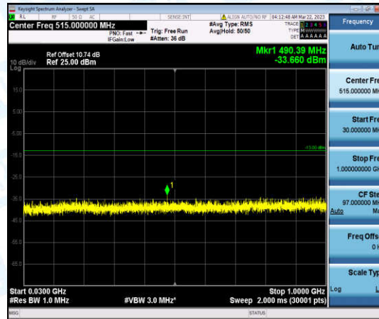
Band25-5MHz-QPSK-26665-1-0-High-30-1000--33.66-PASS
