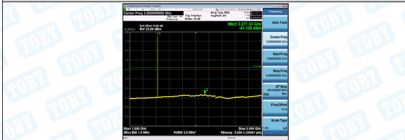
Band25-10MHz-16QAM-26090-1-0-Low-1000-5000--41.13-PASS
