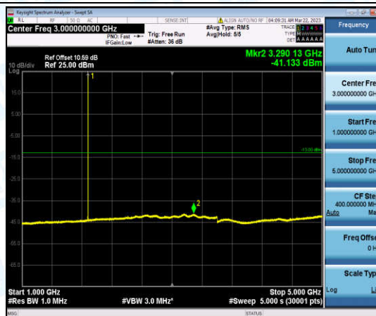
Band25-5MHz-QPSK-26365-1-0-Low-1000-5000--41.13-PASS
