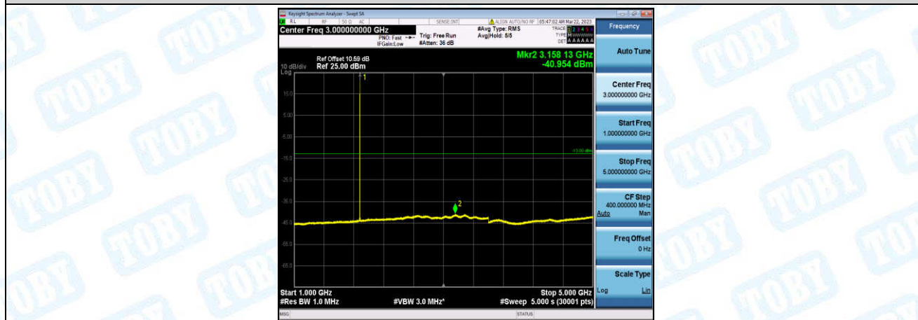
Band25-3MHz-QPSK-26365-1-0-Low-1000-5000--40.95-PASS
