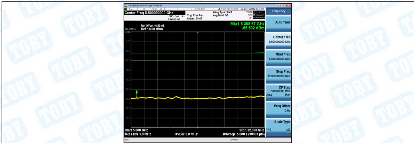
Band25-20MHz-QPSK-26140-1-0-Low-5000-12000--55.59-PASS
