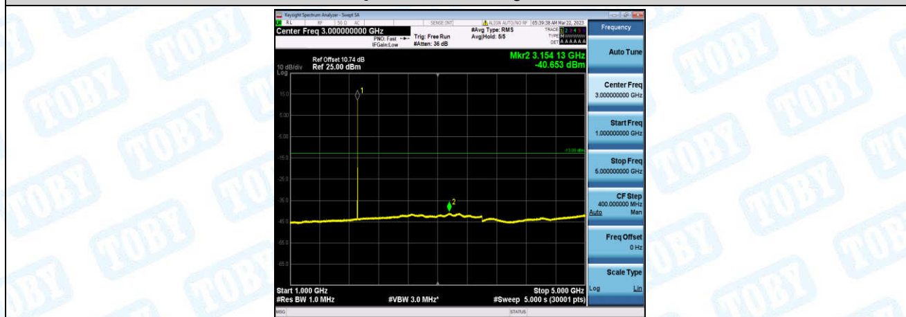
Band25-20MHz-16QAM-26590-1-0-High-1000-5000--40.65-PASS
