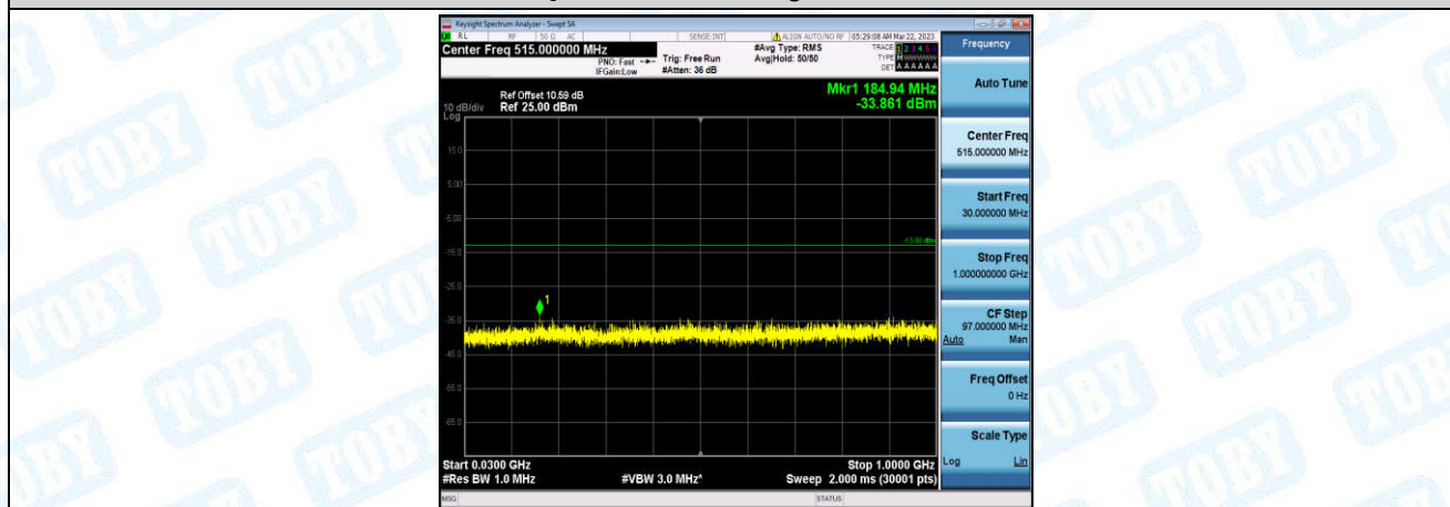
Band25-20MHz-QPSK-26140-1-0-Low-30-1000--33.86-PASS
