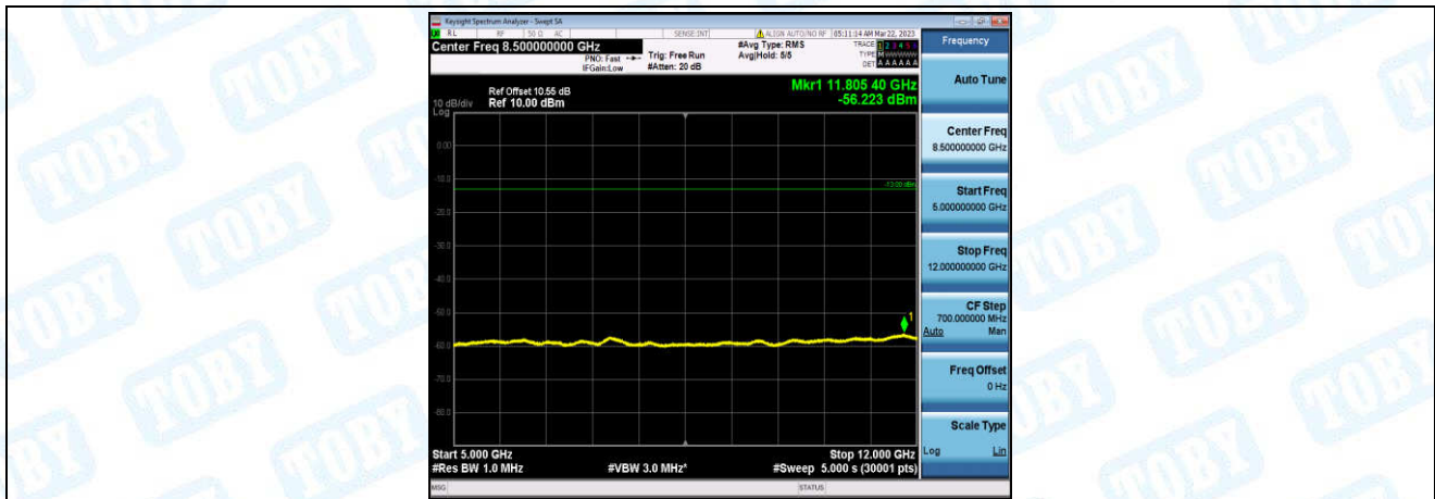
Band25-15MHz-16QAM-26115-1-0-Low-5000-12000--56.22-PASS
