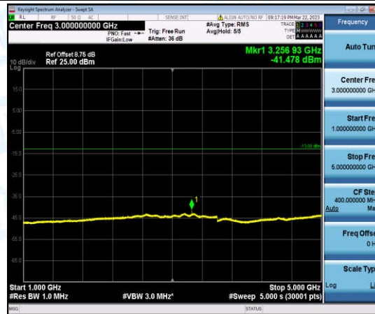
Band26-1.4MHz-QPSK-26697-1-0-Low-1000-5000--41.48-PASS
