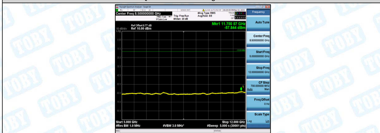
Band26-1.4MHz-QPSK-26783-1-0-High-5000-12000--57.84-PASS
