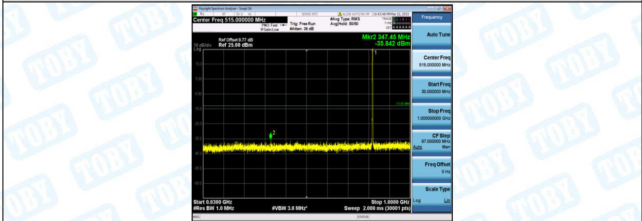
Band26-3MHz-QPSK-26775-1-0-High-30-1000--35.84-PASS
