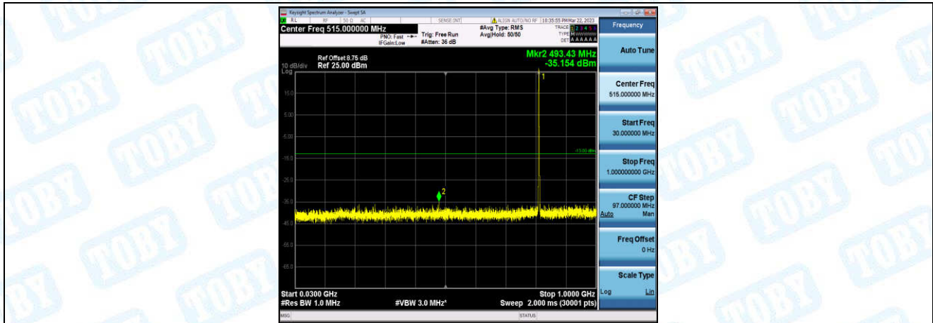
Band26-3MHz-QPSK-26705-1-0-Low-30-1000--35.15-PASS
