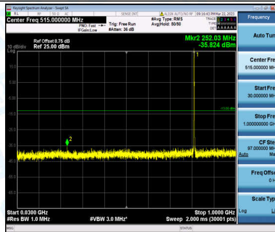
Band26-1.4MHz-QPSK-26697-1-0-Low-30-1000--35.82-PASS
