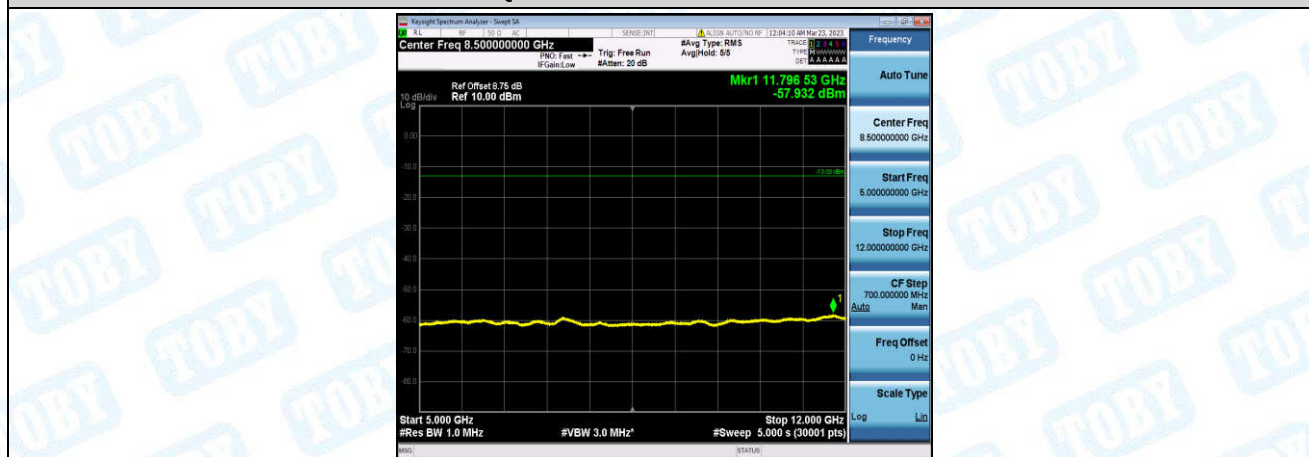
Band26-5MHz-16QAM-26715-1-0-Low-5000-12000--57.93-PASS
