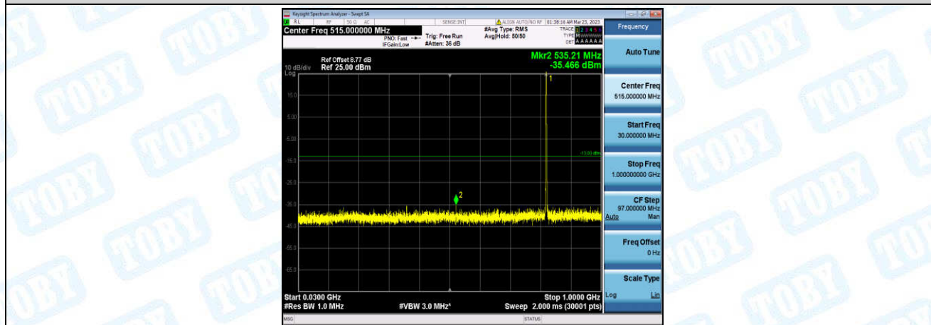
Band26-5MHz-QPSK-26765-1-0-High-30-1000--35.47-PASS
