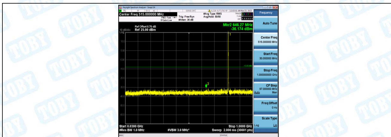
Band26-5MHz-16QAM-26715-1-0-Low-30-1000--36.17-PASS
