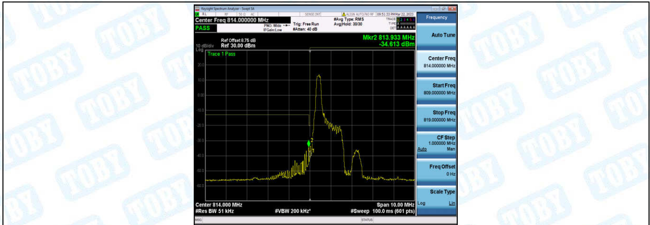
Band26-3MHz-16QAM-26705-1-0-Low--41.58,-34.61-PASS
