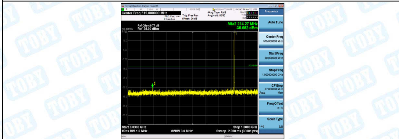
Band26-3MHz-16QAM-26775-1-0-High-30-1000--35.65-PASS
