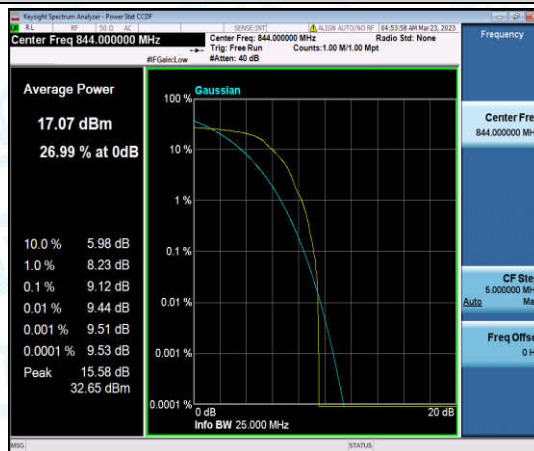
Band26-10MHz-QPSK-26990-1-0-High-9.12-<=13-PASS
