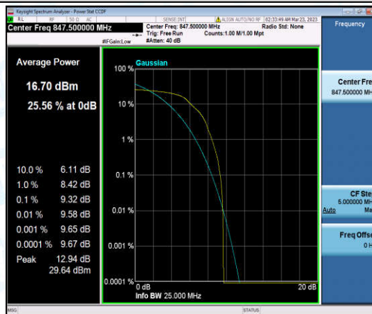
Band26-3MHz-QPSK-27025-1-0-High-9.32-<=13-PASS
