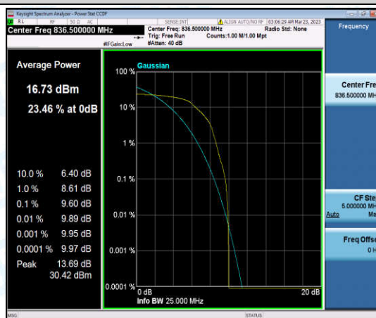
Band26-5MHz-QPSK-26915-1-0-Low-9.60-<=13-PASS
