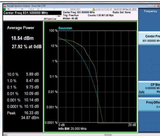
Band26-15MHz-16QAM-26865-1-0-Low-9.75-<=13-PASS
