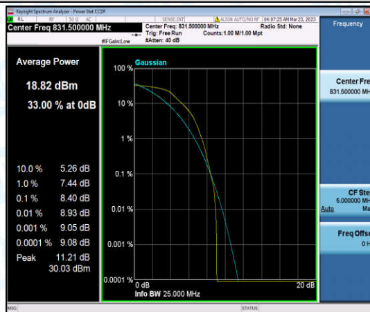
Band26-15MHz-16QAM-26865-6-0-Low-8.40-<=13-PASS
