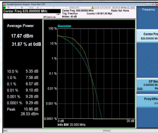
Band26-10MHz-QPSK-26840-6-0-Low-8.57-≤13-PASS
