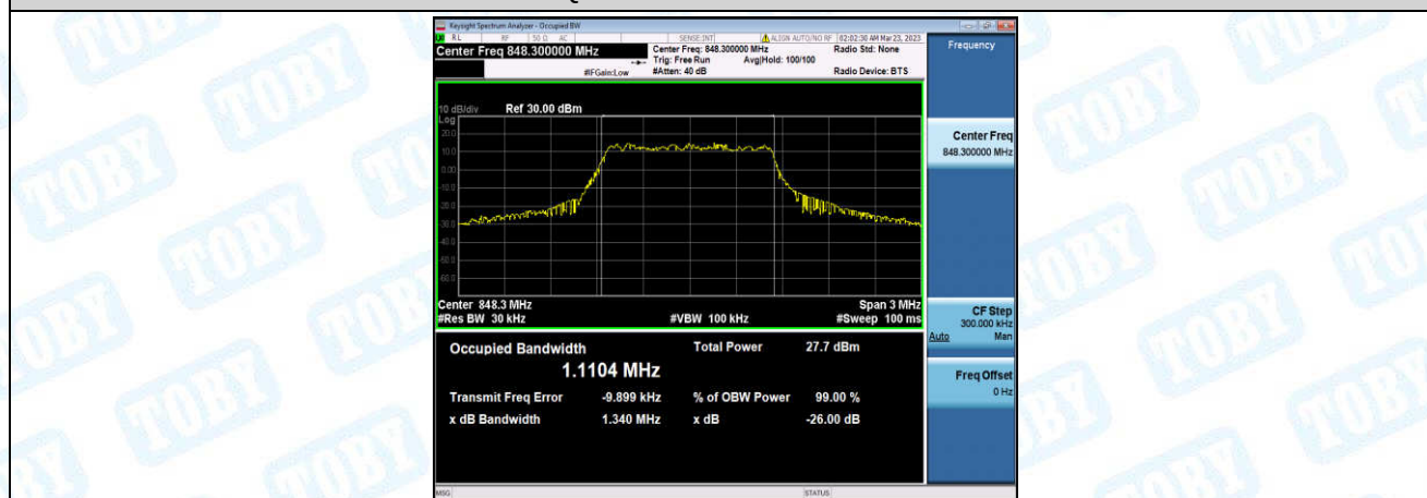
Band26-1.4MHz-QPSK-27033-6-0-High-1.1104-1.340-PASS
