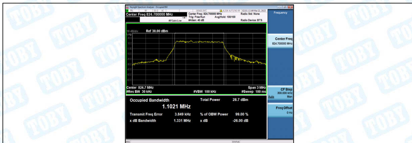
Band26-1.4MHz-QPSK-26797-6-0-Low-1.1021-1.331-PASS
