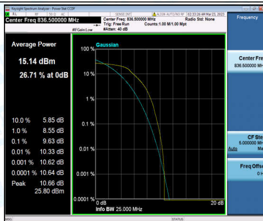
Band26-3MHz-QPSK-26915-6-0-Low-9.63-<=13-PASS
