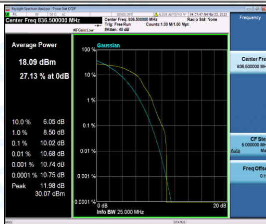
Band26-15MHz-16QAM-26915-1-0-Low-10.02-<=13-PASS
