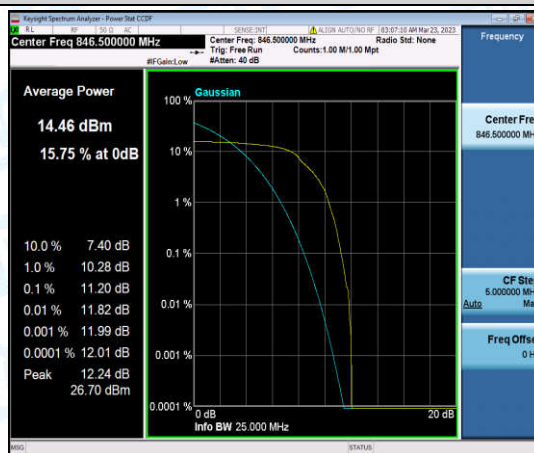
Band26-5MHz-QPSK-27015-1-0-High-11.20-=<=13-PASS
