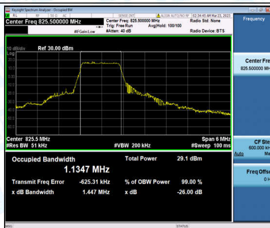
Band26-3MHz-QPSK-26805-6-0-Low-1.1347-1.447-PASS
