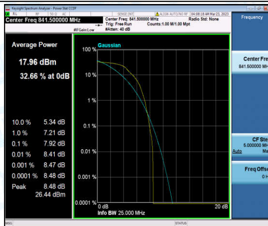
Band26-15MHz-QPSK-26965-1-0-High-7.92-<=13-PASS
