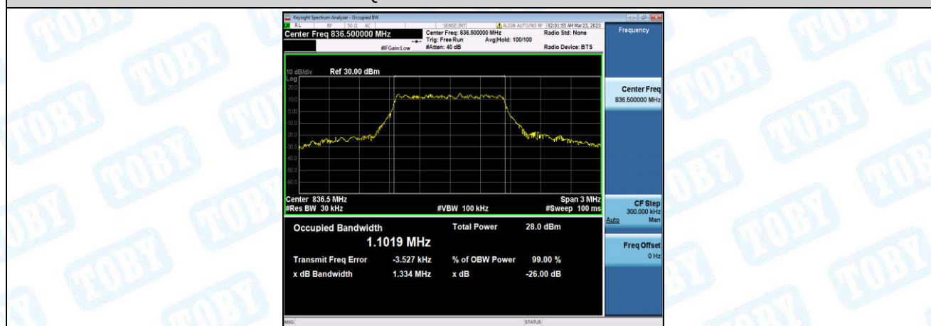
Band26-1.4MHz-QPSK-26915-6-0-Low-1.1019-1.334-PASS
