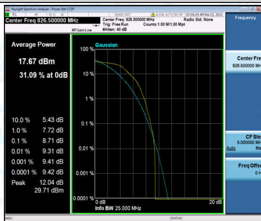
Band26-5MHz-QPSK-26815-6-0-Low-8.71-<=13-PASS
