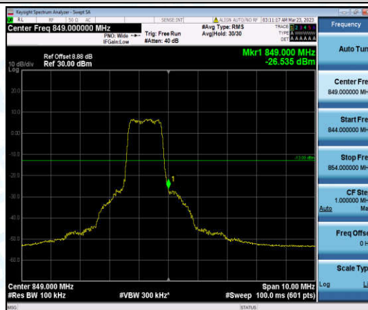
Band26-5MHz-QPSK-27015-6-0-High--26.53-PASS
