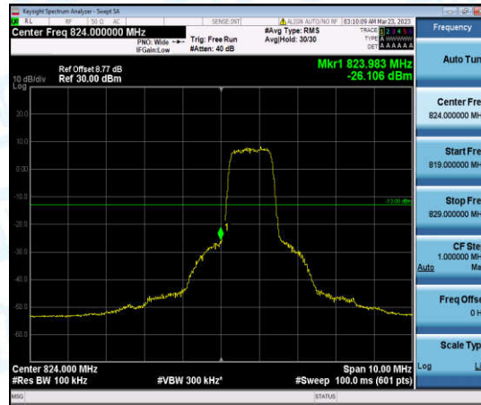
Band26-5MHz-16QAM-26815-6-0-Low--26.11-PASS
