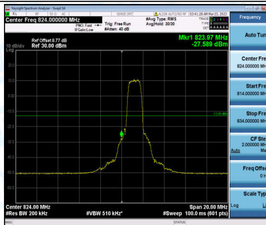
Band26-10MHz-16QAM-26840-6-0-Low--27.59-PASS
