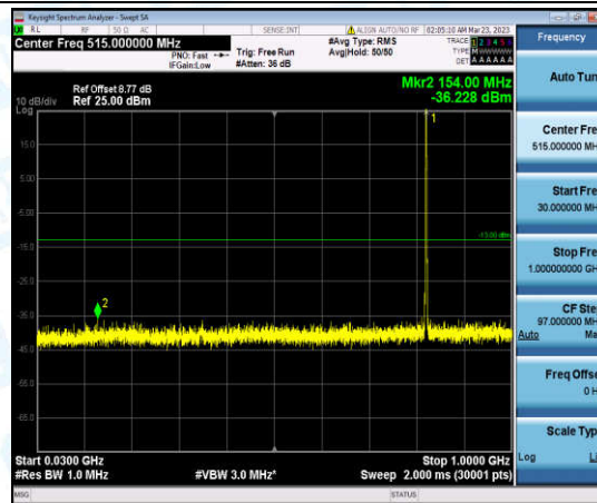
Band26-1.4MHz-QPSK-26797-1-0-Low-30-1000--36.23-PASS
