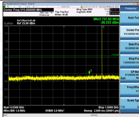
Band26-1.4MHz-16QAM-27033-1-0-High-30-1000--36.33-PASS
