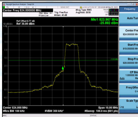
Band26-5MHz-QPSK-26815-6-0-Low--25.89-PASS
