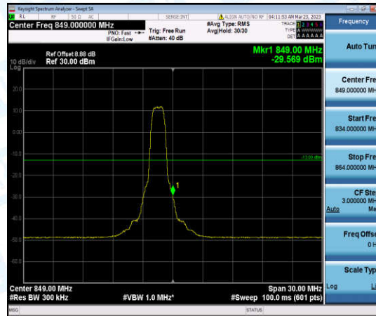
Band26-15MHz-QPSK-26965-6-0-High--29.57-PASS
