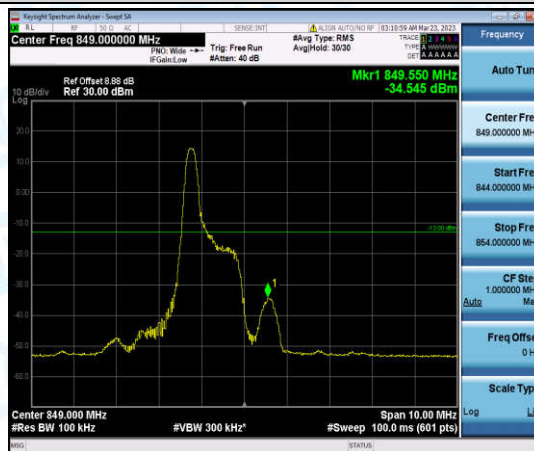
Band26-5MHz-QPSK-27015-1-0-High--34.54-PASS
