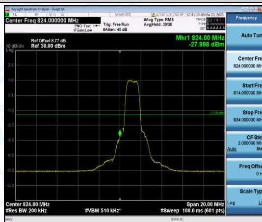
Band26-10MHz-QPSK-26840-6-0-Low--28.00-PASS
