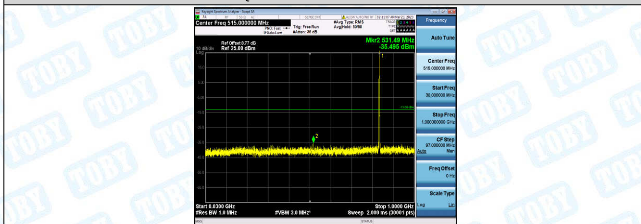
Band26-1.4MHz-16QAM-26915-1-0-Low-30-1000--35.5-PASS
