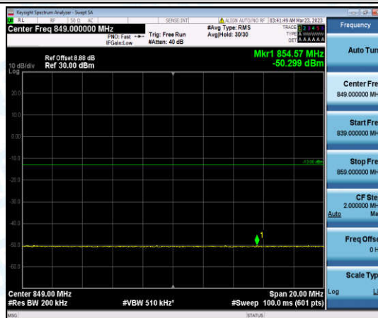
Band26-10MHz-16QAM-26915-1-0-Low--50.30-PASS
