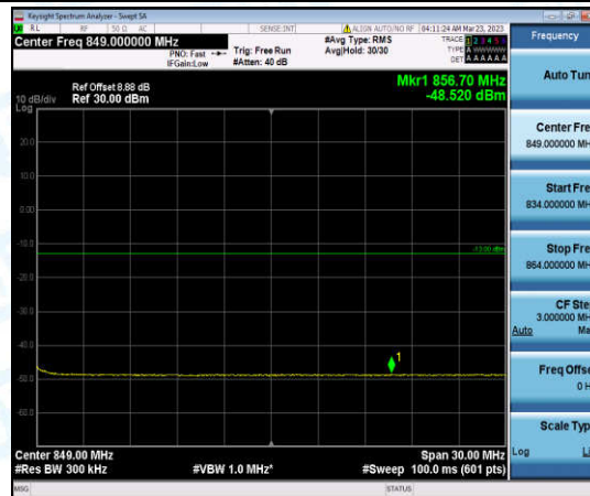
Band26-15MHz-16QAM-26915-6-0-Low--48.52-PASS
