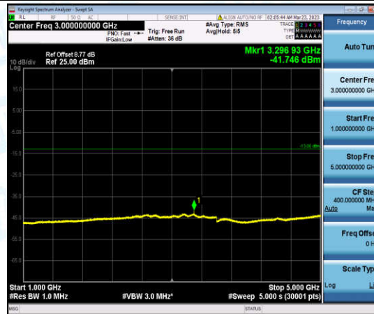
Band26-1.4MHz-QPSK-26797-1-0-Low-1000-5000--41.75-PASS
