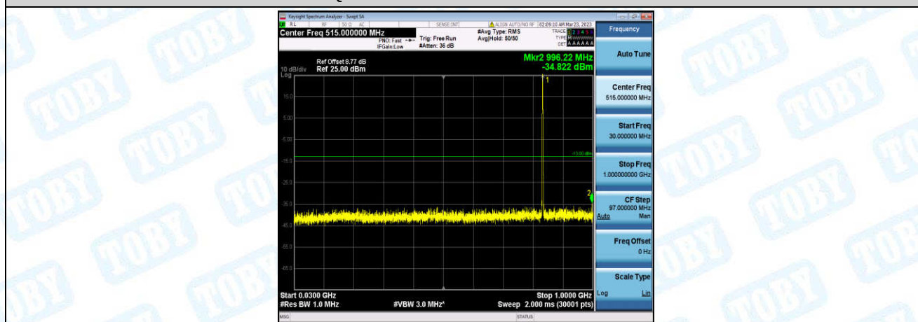
Band26-1.4MHz-QPSK-26915-1-0-Low-30-1000--34.82-PASS
