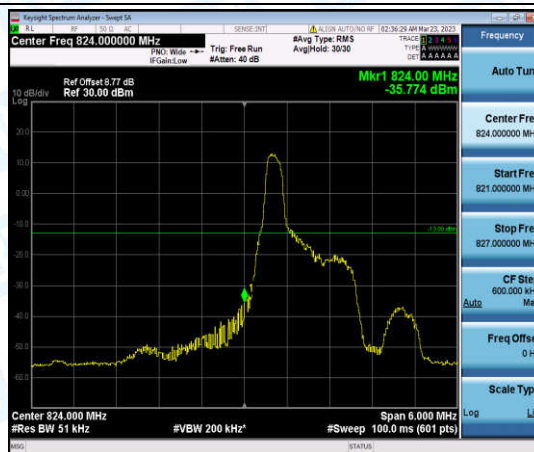
Band26-3MHz-QPSK-26805-1-0-Low--35.77-PASS
