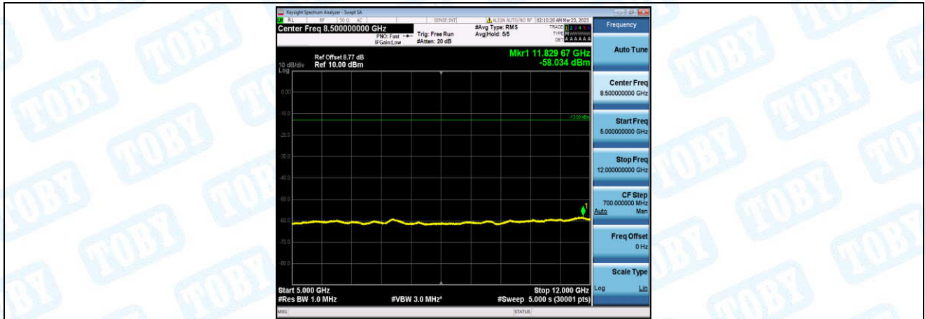
Band26-1.4MHz-QPSK-26915-1-0-Low-5000-12000--58.03-PASS
