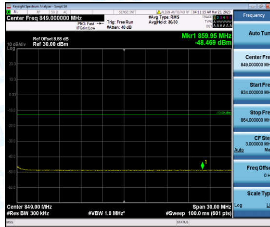
Band26-15MHz-QPSK-26915-6-0-Low--48.47-PASS
