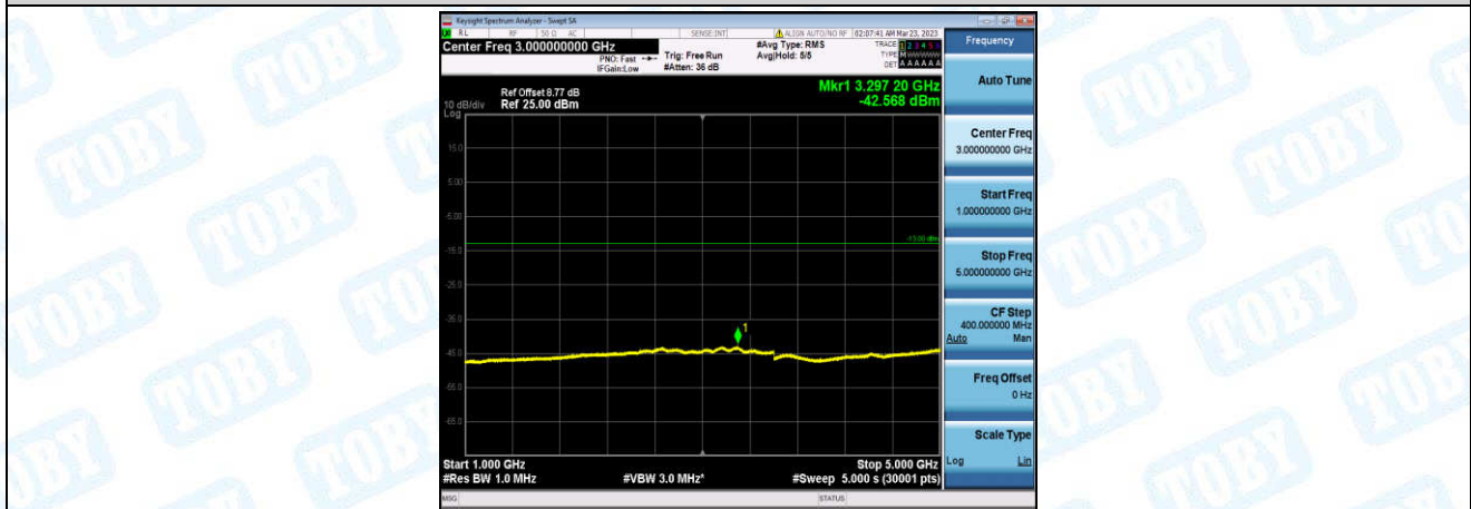
Band26-1.4MHz-16QAM-26797-1-0-Low-1000-5000--42.57-PASS
