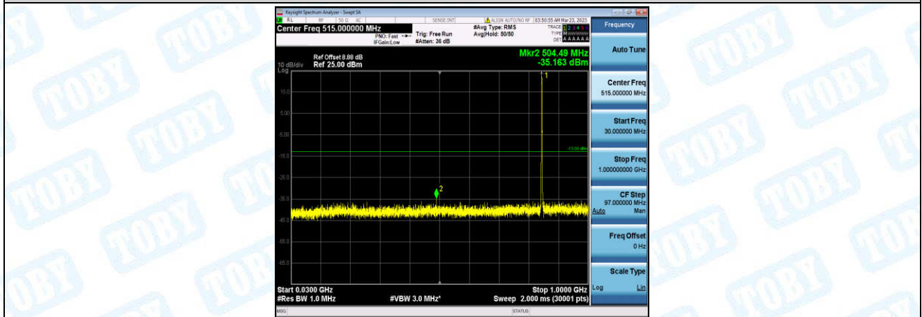
Band26-10MHz-QPSK-26990-1-0-High-30-1000--35.16-PASS
