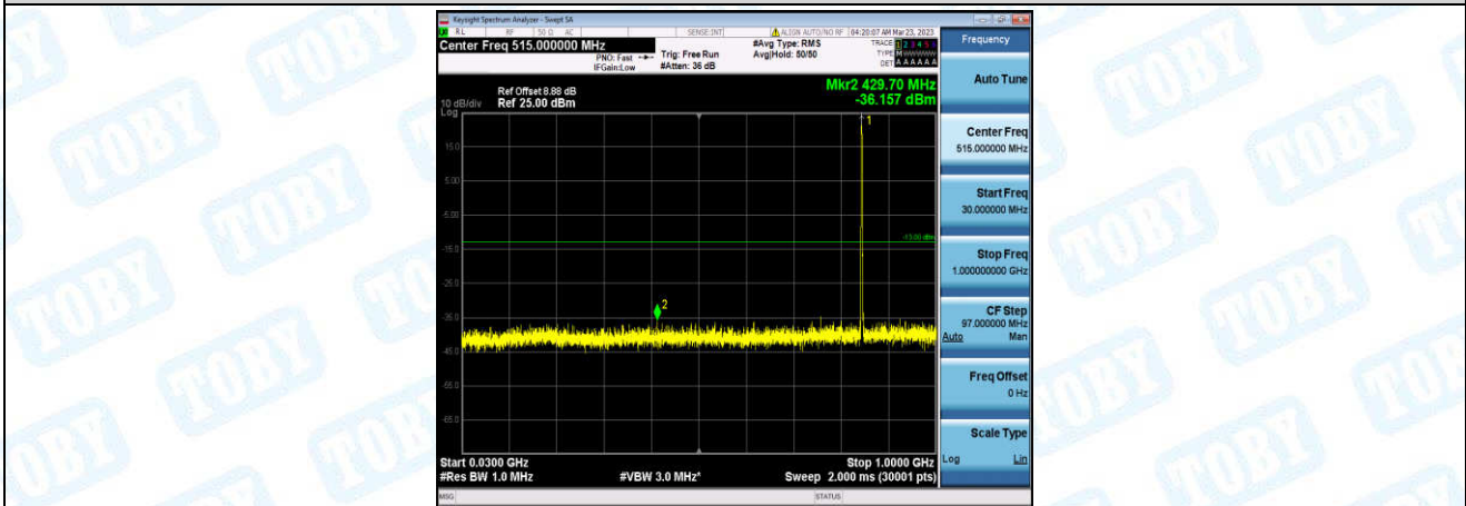
Band26-15MHz-QPSK-26965-1-0-High-30-1000--36.16-PASS
