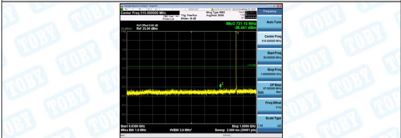
Band26-5MHz-QPSK-27015-1-0-High-30-1000--36.44-PASS
