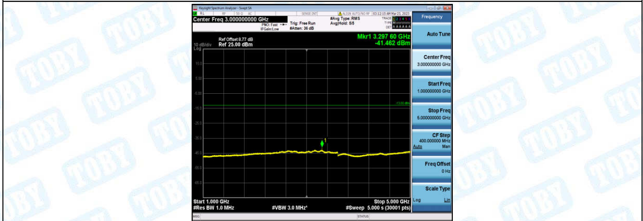
Band26-5MHz-QPSK-26815-1-0-Low-1000-5000--41.46-PASS
