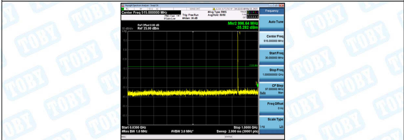
Band26-15MHz-16QAM-26965-1-0-High-30-1000--35.28-PASS
