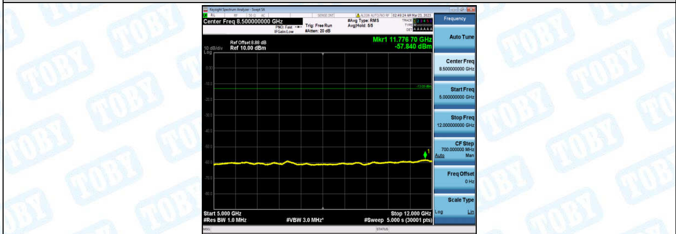
Band26-3MHz-16QAM-27025-1-0-High-5000-12000--57.84-PASS
