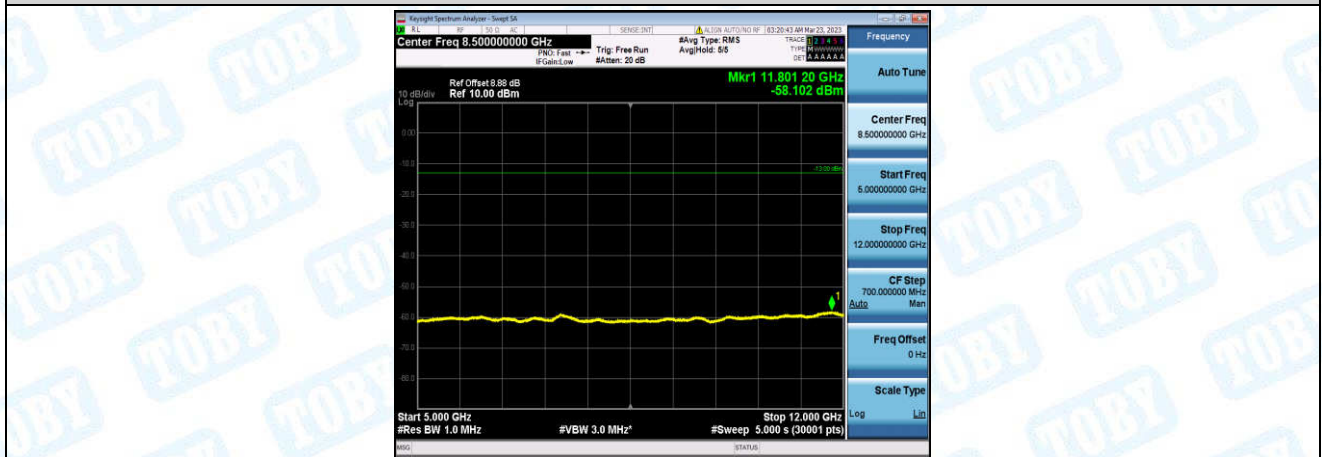
Band26-5MHz-QPSK-27015-1-0-High-5000-12000--58.1-PASS
