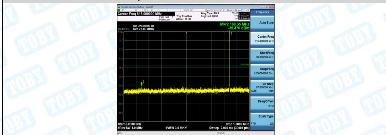
Band26-3MHz-QPSK-27025-1-0-High-30-1000--35.47-PASS
