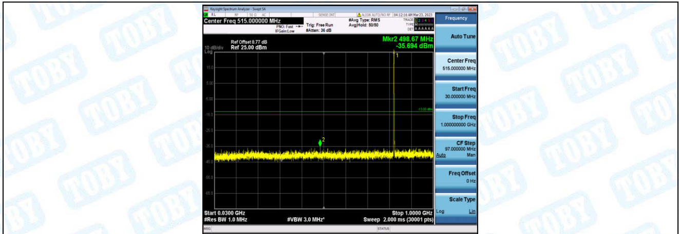
Band26-15MHz-QPSK-26865-1-0-Low-30-1000--35.69-PASS
