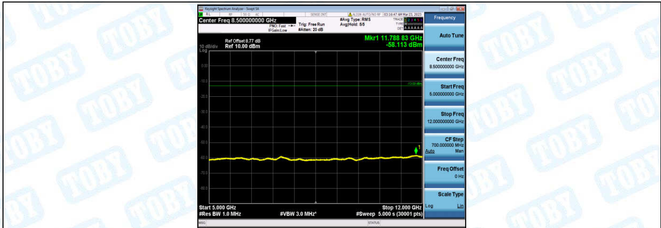
Band26-5MHz-QPSK-26915-1-0-Low-5000-12000--58.11-PASS
