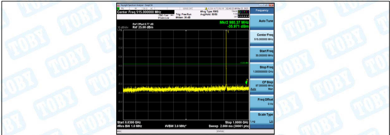
Band26-3MHz-16QAM-26805-1-0-Low-30-1000--35.97-PASS
