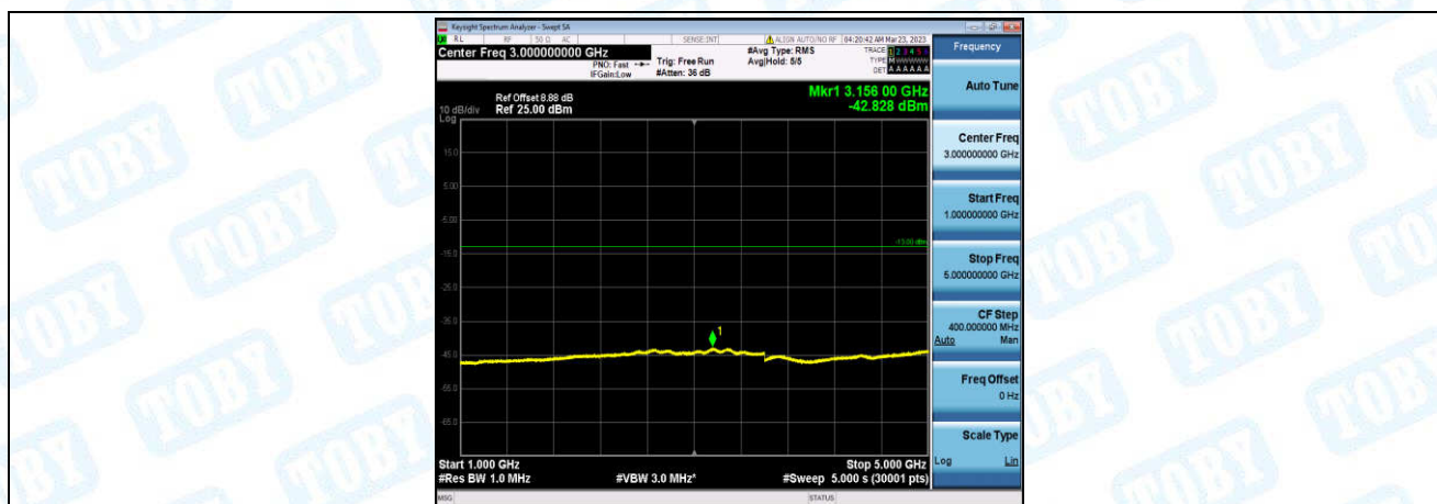
Band26-15MHz-QPSK-26965-1-0-High-1000-5000--42.83-PASS
