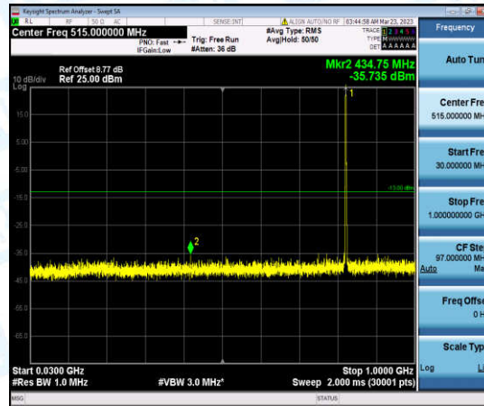
Band26-10MHz-16QAM-26840-1-0-Low-30-1000--35.74-PASS
