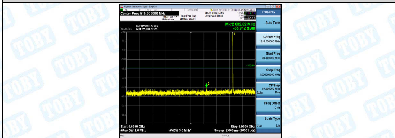
Band26-15MHz-QPSK-26915-1-0-Low-30-1000--35.91-PASS
