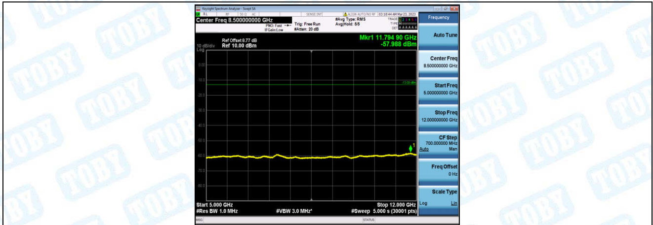
Band26-5MHz-16QAM-26915-1-0-Low-5000-12000--57.99-PASS
