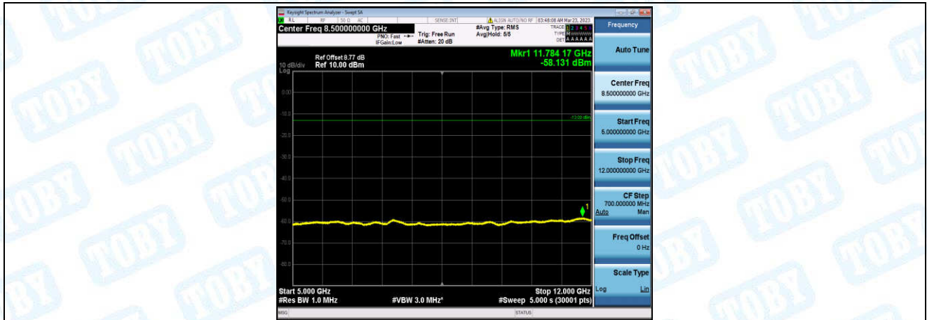
Band26-10MHz-QPSK-26915-1-0-Low-5000-12000--58.13-PASS
