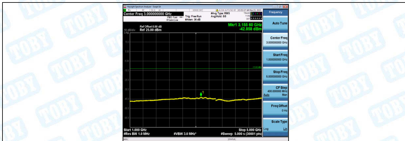
Band26-10MHz-16QAM-26990-1-0-High-1000-5000--42.86-PASS
