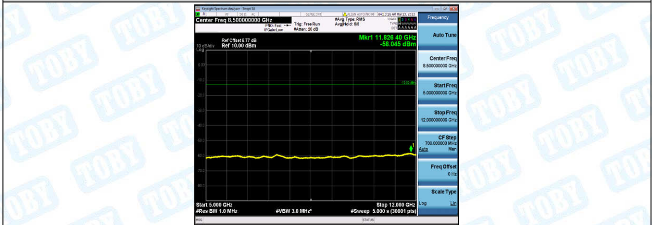
Band26-15MHz-QPSK-26865-1-0-Low-5000-12000--58.05-PASS
