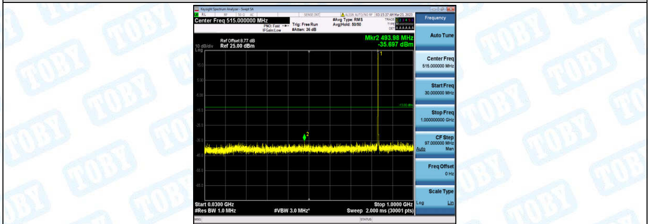
Band26-5MHz-QPSK-26915-1-0-Low-30-1000--35.7-PASS
