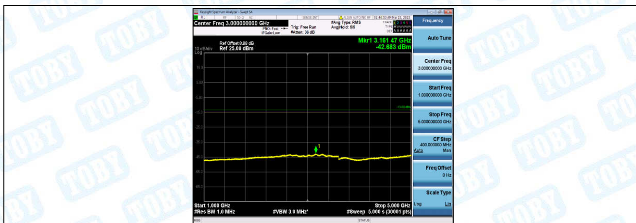
Band26-3MHz-QPSK-27025-1-0-High-1000-5000--42.68-PASS
