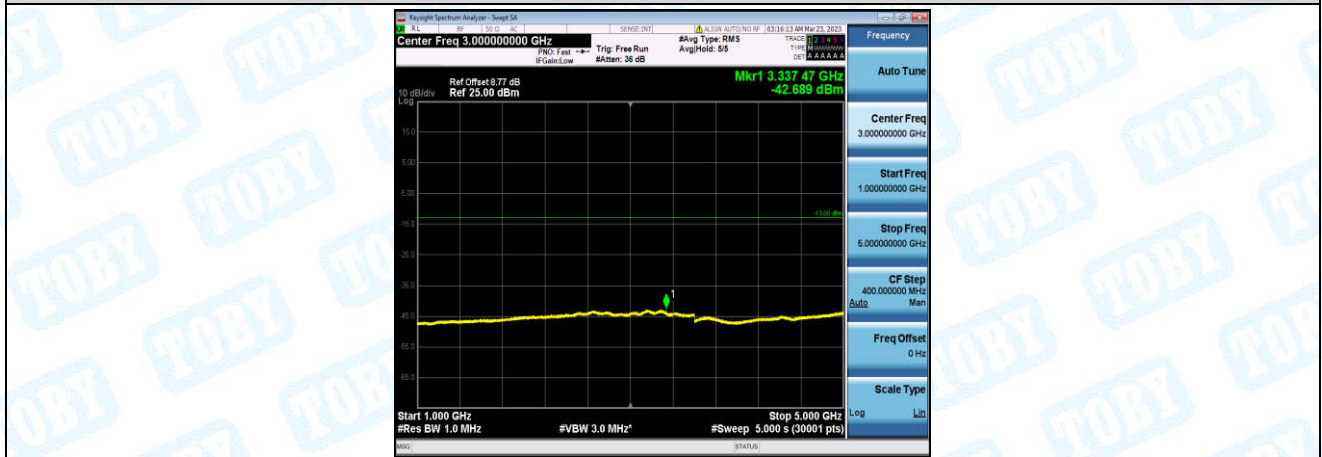
Band26-5MHz-QPSK-26915-1-0-Low-1000-5000--42.69-PASS
