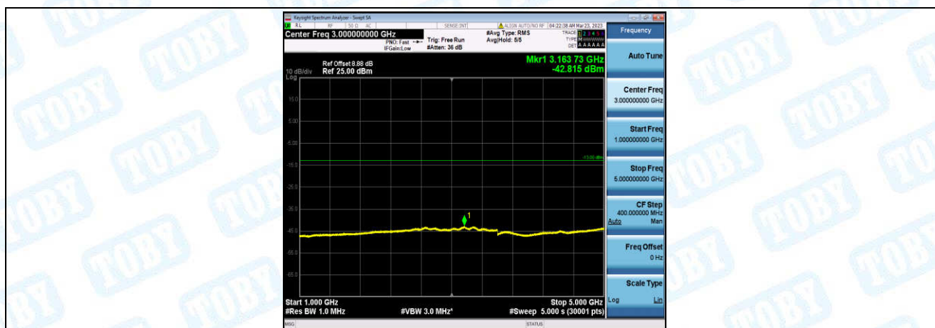
Band26-15MHz-16QAM-26965-1-0-High-1000-5000--42.82-PASS
