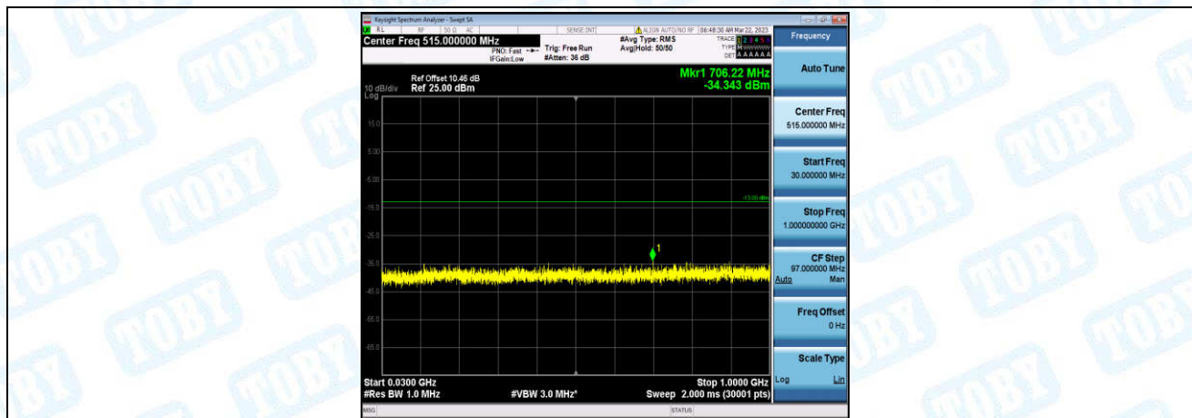
Band4-5MHz-QPSK-19975-1-0-Low-30-1000--34.34-PASS
