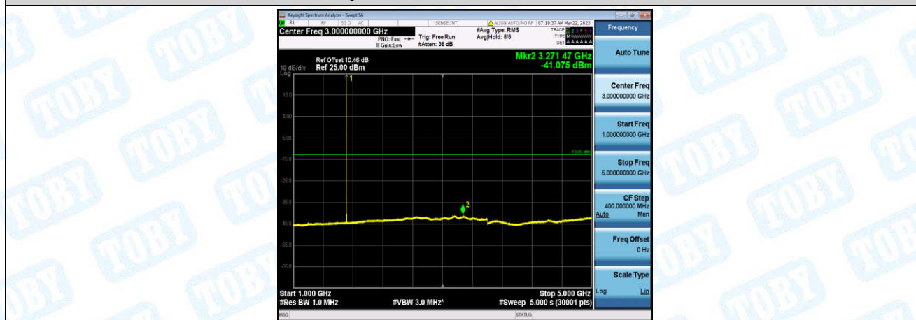
Band4-10MHz-QPSK-20000-1-0-Low-1000-5000--41.08-PASS
