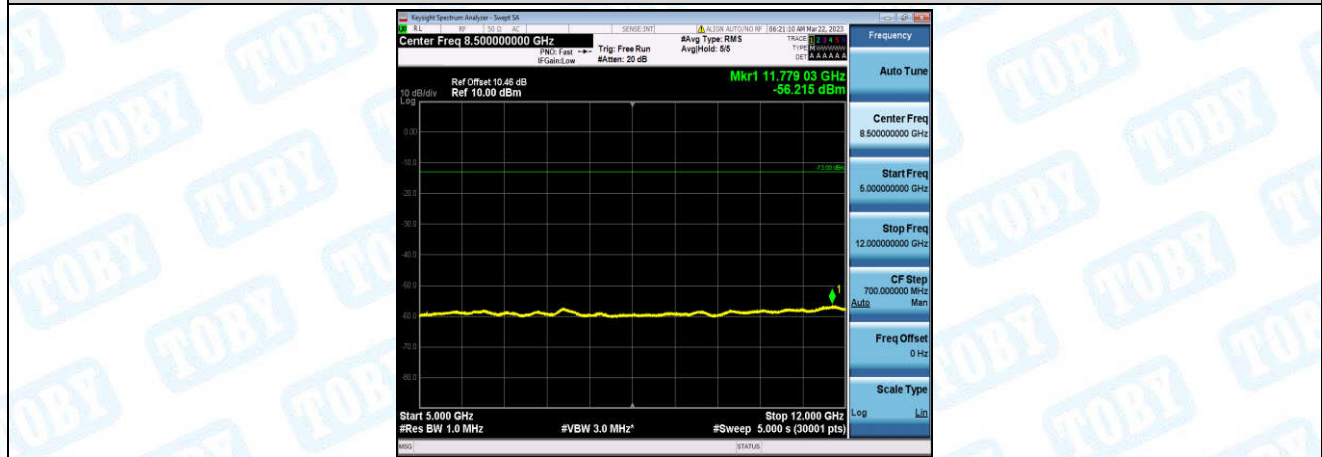
Band4-3MHz-16QAM-19965-1-0-Low-5000-12000--56.22-PASS
