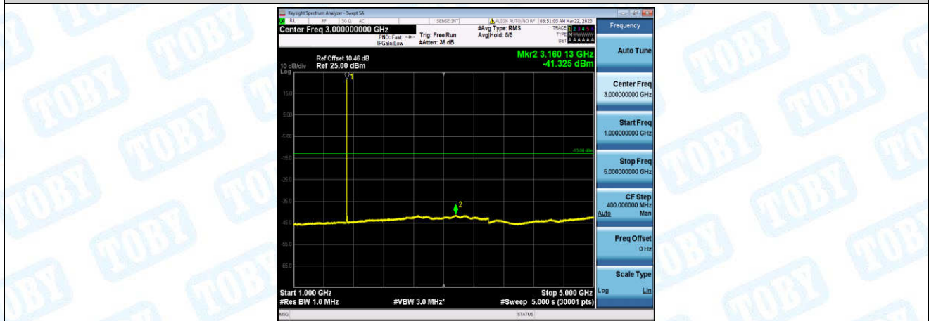
Band4-5MHz-16QAM-19975-1-0-Low-1000-5000--41.33-PASS
