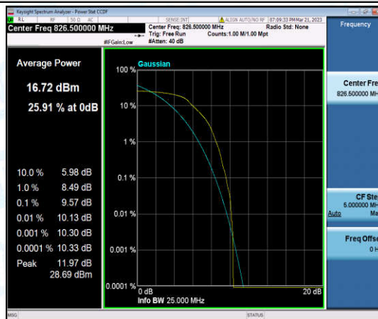
Band5-5MHz-QPSK-20425-6-0-Low-9.57-<=13-PASS
