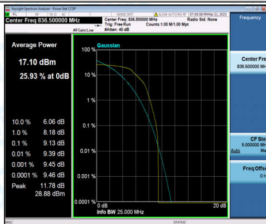
Band5-5MHz-QPSK-20525-1-0-Low-9.13-<=13-PASS
