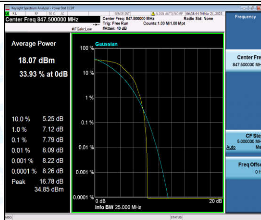
Band5-3MHz-QPSK-20635-1-0-High-7.79-<=13-PASS
