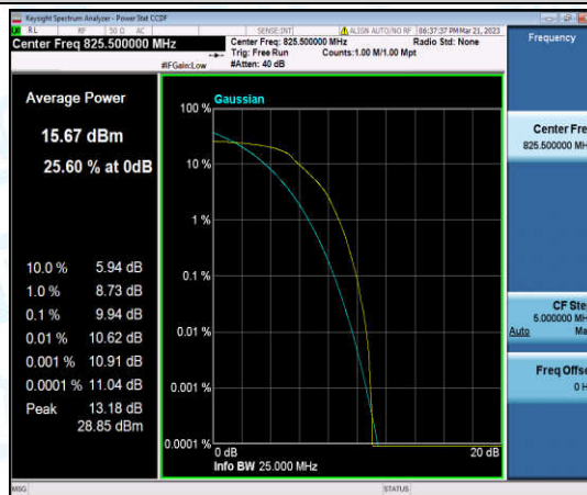
Band5-3MHz-QPSK-20415-6-0-Low-9.94-≤13-PASS
