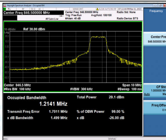
Band5-5MHz-QPSK-20625-6-0-High-1.2141-1.499-PASS
