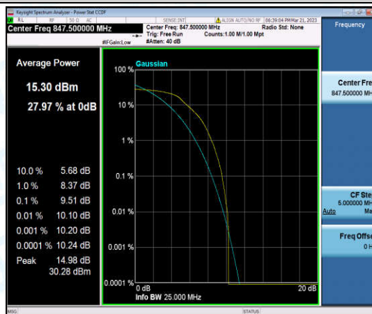
Band5-3MHz-QPSK-20635-6-0-High-9.51-<=13-PASS
