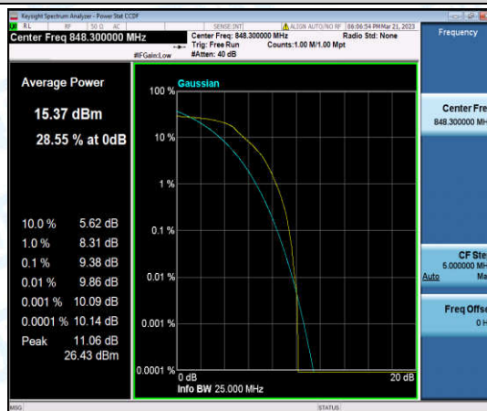
Band5-1.4MHz-16QAM-20643-6-0-High-9.38-<=13-PASS
