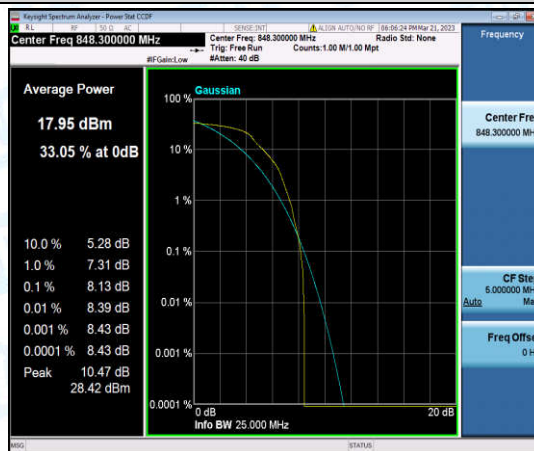
Band5-1.4MHz-QPSK-20643-1-0-High-8.13-<=13-PASS
