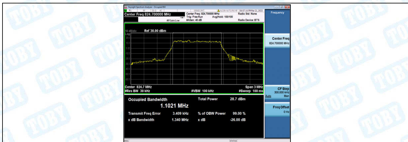
Band5-1.4MHz-QPSK-20407-6-0-Low-1.1021-1.340-PASS
