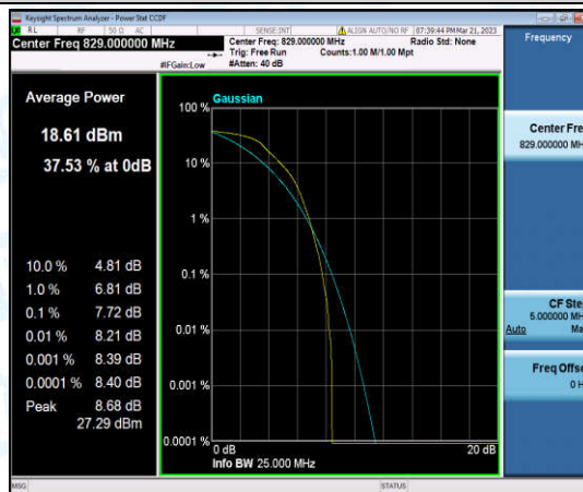
Band5-10MHz-16QAM-20450-6-0-Low-7.72-<=13-PASS
