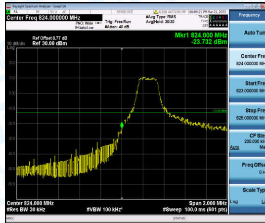
Band5-1.4MHz-16QAM-20407-1-0-Low--23.73-PASS
