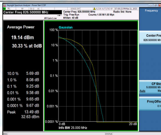
Band5-5MHz-16QAM-20425-1-0-Low-9.25-<=13-PASS
