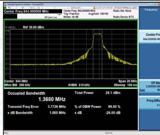
Band5-10MHz-16QAM-20600-6-0-High-1.3680-1.860-PASS
