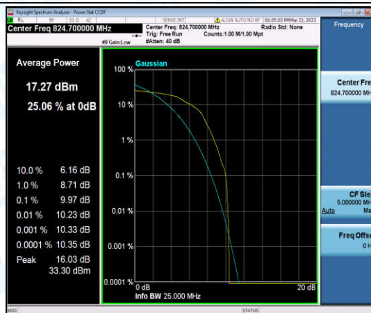
Band5-1.4MHz-16QAM-20407-1-0-Low-9.97-<=13-PASS
