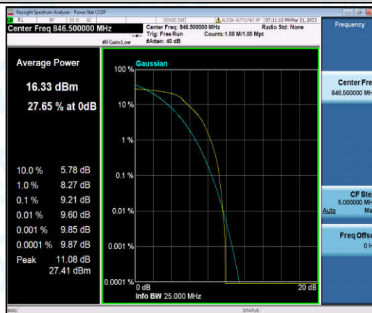
Band5-5MHz-16QAM-20625-6-0-High-9.21-<=13-PASS
