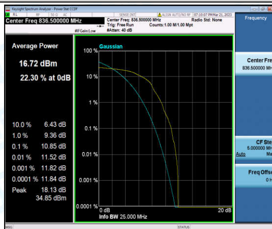
Band5-5MHz-16QAM-20525-1-0-Low-10.85-<=13-PASS
