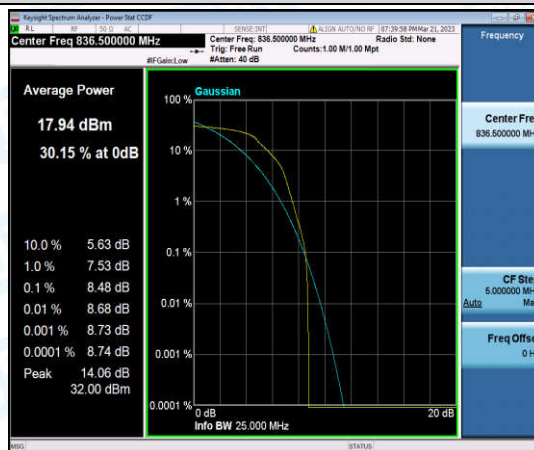
Band5-10MHz-QPSK-20525-1-0-Low-8.48-<=13-PASS
