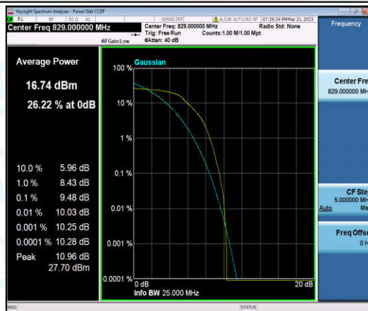
Band5-10MHz-QPSK-20450-6-0-Low-9.48-<=13-PASS
