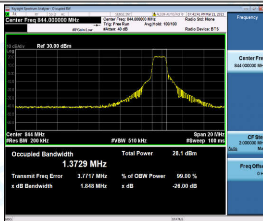
Band5-10MHz-QPSK-20600-6-0-High-1.3729-1.848-PASS
