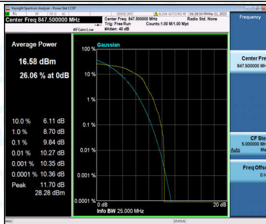
Band5-3MHz-16QAM-20635-1-0-High-9.84-<=13-PASS
