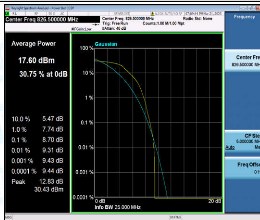
Band5-5MHz-16QAM-20425-6-0-Low-8.70-<=13-PASS
