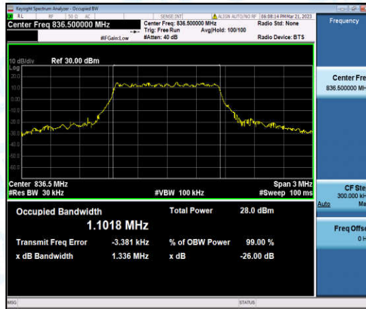
Band5-1.4MHz-16QAM-20525-6-0-Low-1.1018-1.336-PASS
