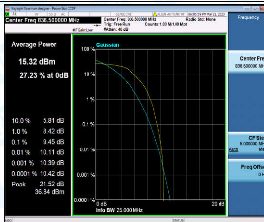
Band5-1.4MHz-QPSK-20525-6-0-Low-9.45-<=13-PASS
