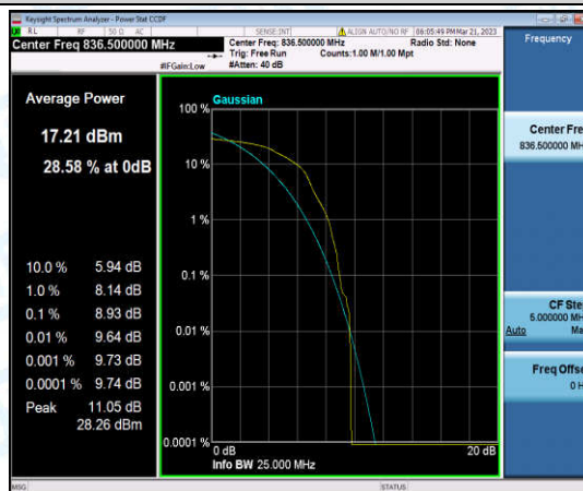
Band5-1.4MHz-16QAM-20525-1-0-Low-8.93-<=13-PASS
