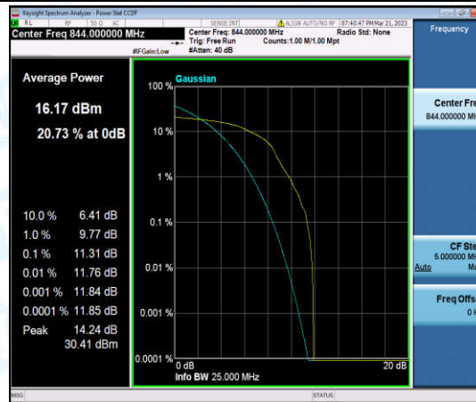
Band5-10MHz-16QAM-20600-1-0-High-11.31-<=13-PASS
