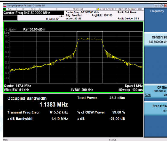
Band5-3MHz-16QAM-20635-6-0-High-1.1383-1.410-PASS
