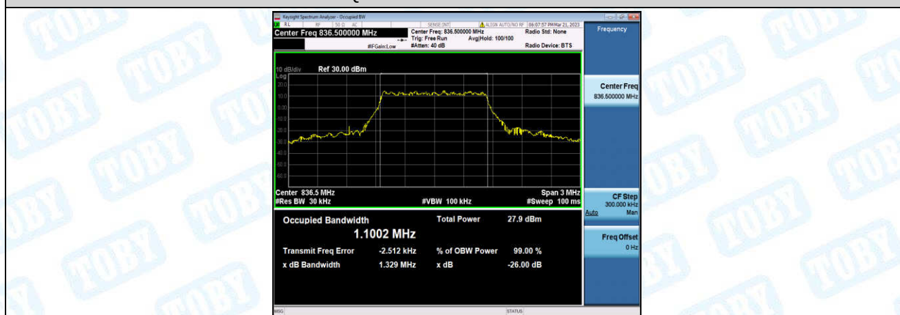
Band5-1.4MHz-QPSK-20525-6-0-Low-1.1002-1.329-PASS
