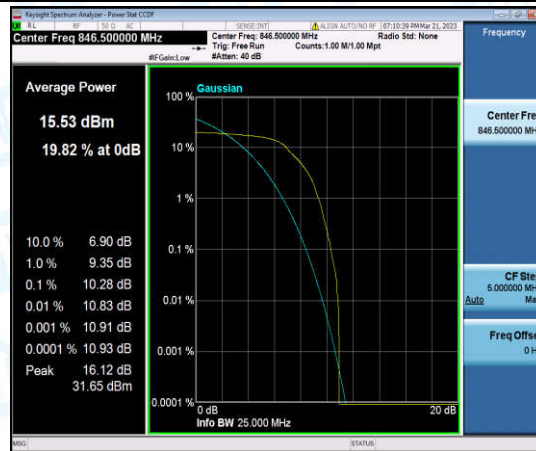
Band5-5MHz-QPSK-20625-1-0-High-10.28-<=13-PASS
