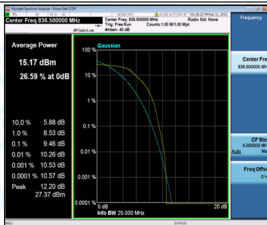
Band5-3MHz-QPSK-20525-6-0-Low-9.46-<=13-PASS
