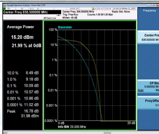
Band5-10MHz-QPSK-20525-6-0-Low-10.09-<=13-PASS
