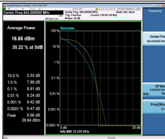
Band5-10MHz-QPSK-20600-6-0-High-8.81-<=13-PASS
