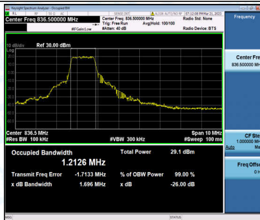
Band5-5MHz-QPSK-20525-6-0-Low-1.2126-1.696-PASS
