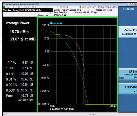
Band5-10MHz-QPSK-20600-1-0-High-10.05-<=13-PASS
