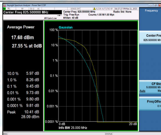
Band5-3MHz-16QAM-20415-1-0-Low-9.45-<=13-PASS
