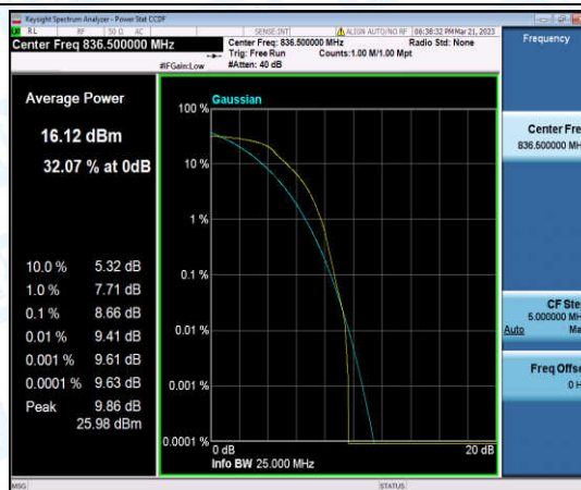
Band5-3MHz-16QAM-20525-6-0-Low-8.66-<=13-PASS
