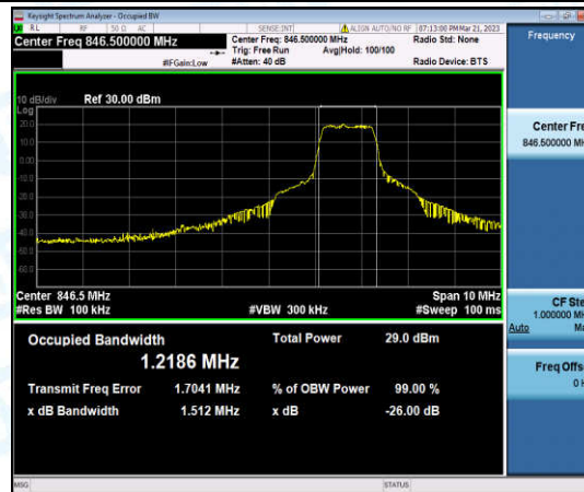
Band5-5MHz-16QAM-20625-6-0-High-1.2186-1.512-PASS
