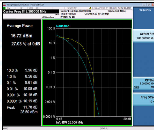
Band5-1.4MHz-16QAM-20643-1-0-High-9.61-<=13-PASS
