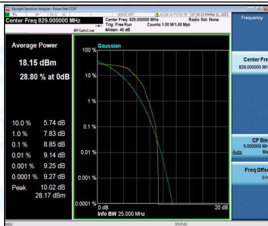
Band5-10MHz-QPSK-20450-1-0-Low-8.85-<=13-PASS
