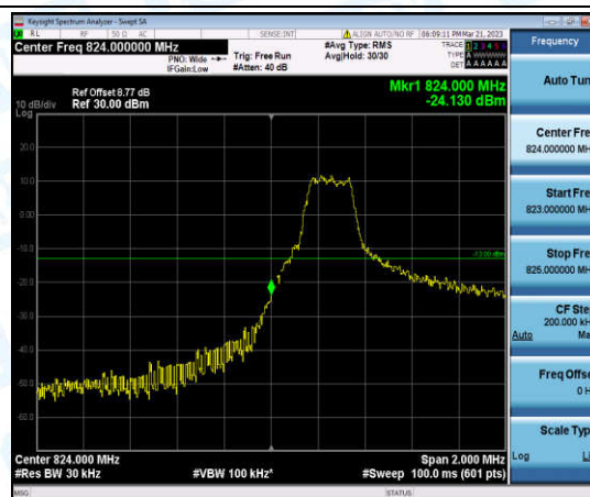
Band5-1.4MHz-QPSK-20407-1-0-Low--24.13-PASS
