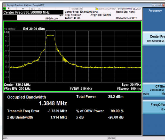
Band5-10MHz-QPSK-20525-6-0-Low-1.3848-1.914-PASS
