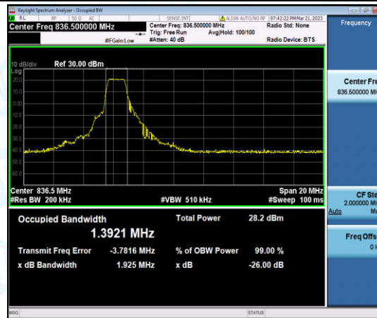
Band5-10MHz-16QAM-20525-6-0-Low-1.3921-1.925-PASS
