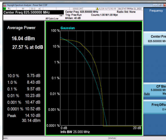
Band5-3MHz-16QAM-20415-6-0-Low-9.57-<=13-PASS
