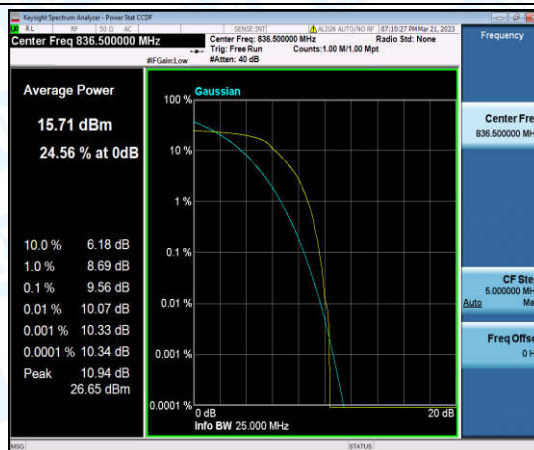
Band5-5MHz-16QAM-20525-6-0-Low-9.56-<=13-PASS
