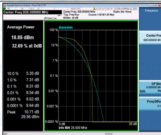
Band5-5MHz-QPSK-20425-1-0-Low-8.31-<=13-PASS
