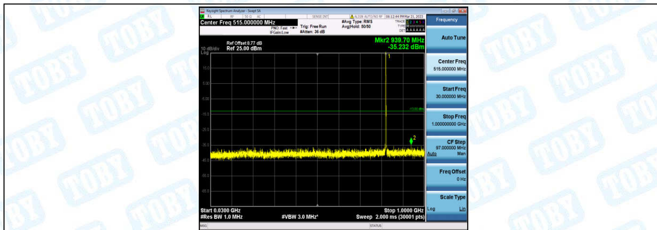
Band5-1.4MHz-16QAM-20407-1-0-Low-30-1000--35.23-PASS
