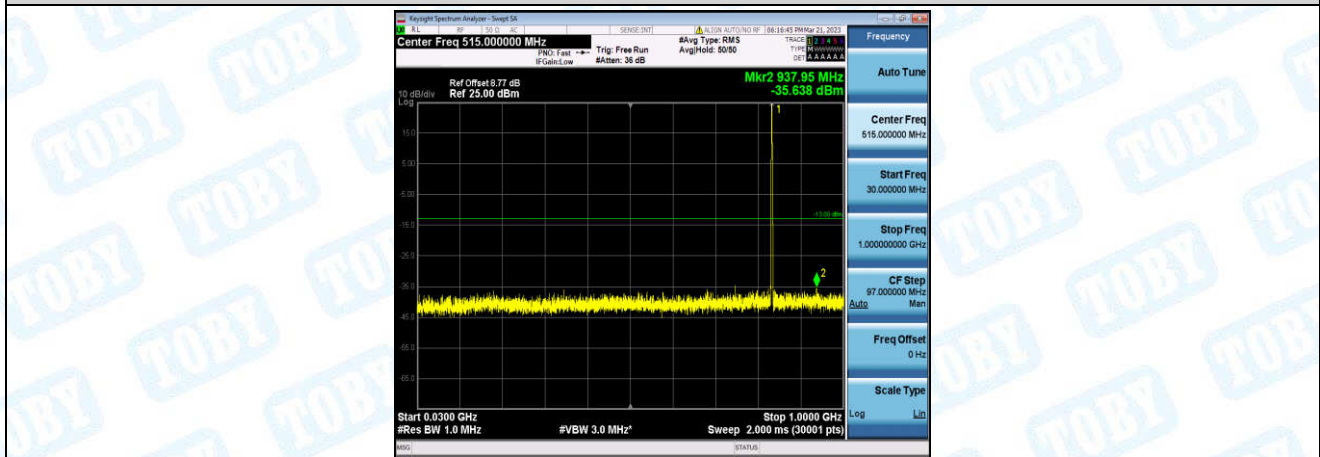
Band5-1.4MHz-16QAM-20525-1-0-Low-30-1000--35.64-PASS
