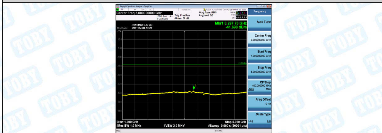
Band5-3MHz-QPSK-20415-1-0-Low-1000-5000--41.7-PASS
