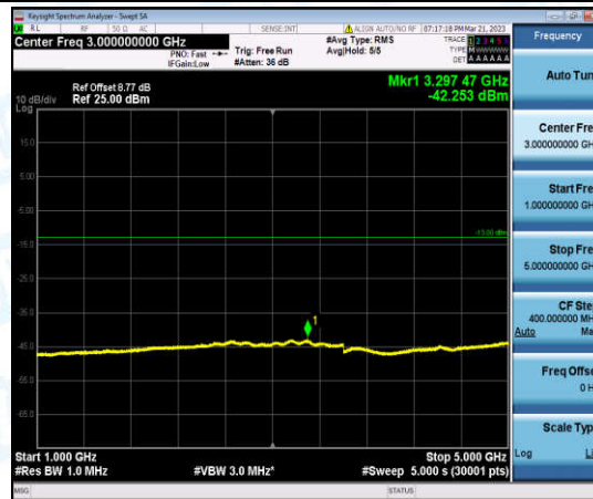
Band5-5MHz-16QAM-20425-1-0-Low-1000-5000--42.25-PASS
