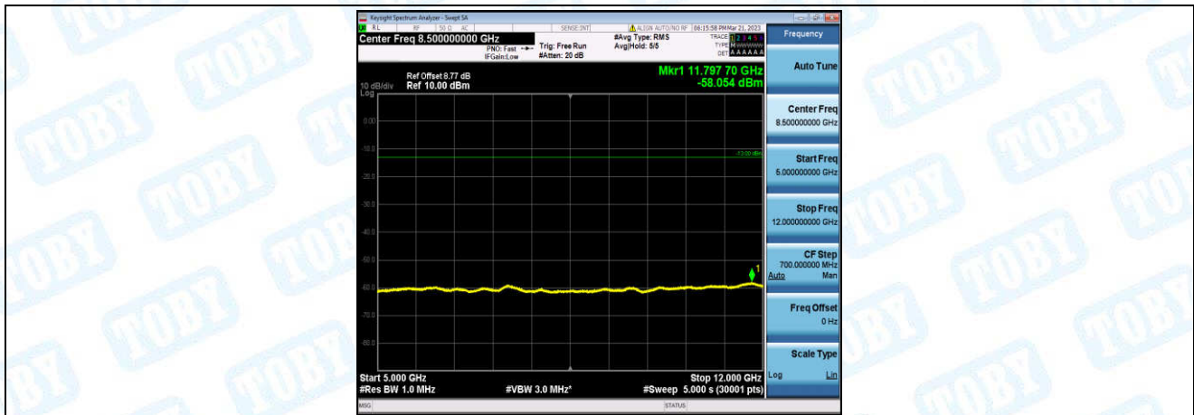
Band5-1.4MHz-QPSK-20525-1-0-Low-5000-12000--58.05-PASS
