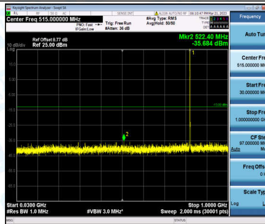
Band5-1.4MHz-QPSK-20407-1-0-Low-30-1000--35.68-PASS
