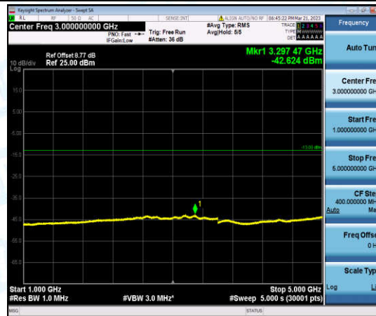
Band5-3MHz-16QAM-20415-1-0-Low-1000-5000--42.62-PASS
