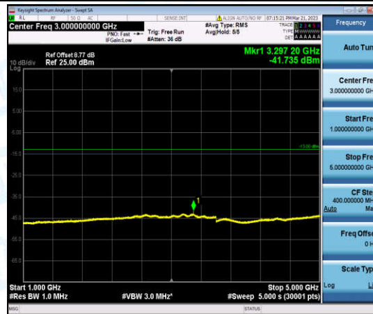
Band5-5MHz-QPSK-20425-1-0-Low-1000-5000--41.74-PASS
