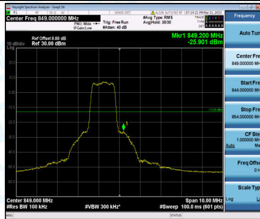
Band5-5MHz-QPSK-20625-6-0-High--25.90-PASS
