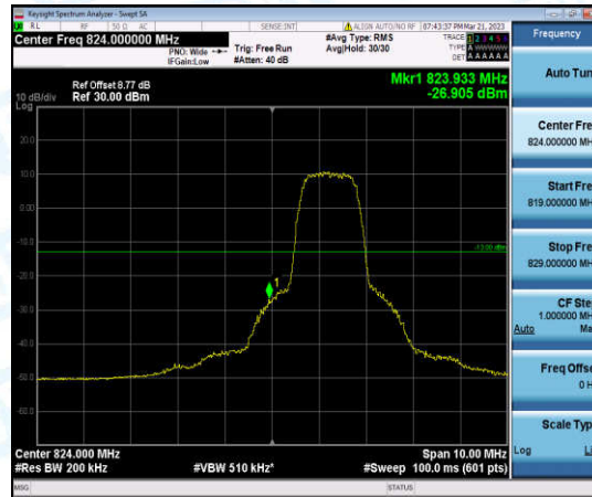
Band5-10MHz-16QAM-20450-6-0-Low--26.91-PASS
