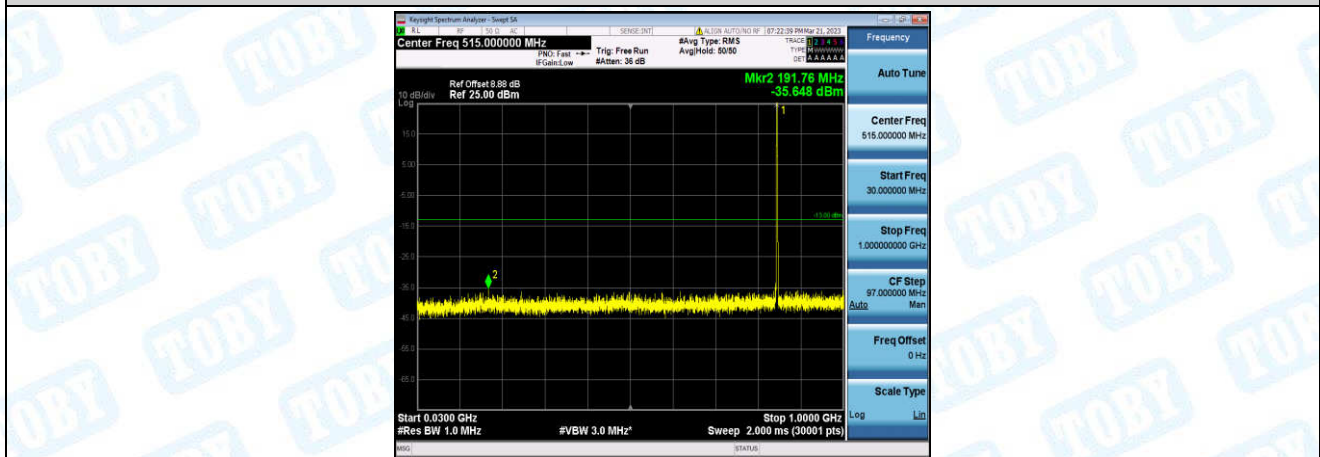
Band5-5MHz-QPSK-20625-1-0-High-30-1000--35.65-PASS
