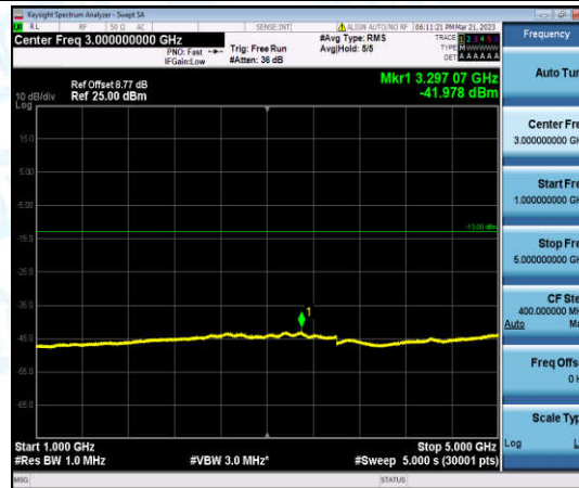
Band5-1.4MHz-QPSK-20407-1-0-Low-1000-5000--41.98-PASS
