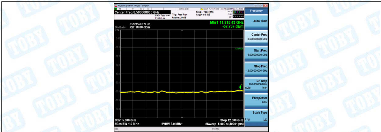
Band5-3MHz-16QAM-20525-1-0-Low-5000-12000--57.74-PASS
