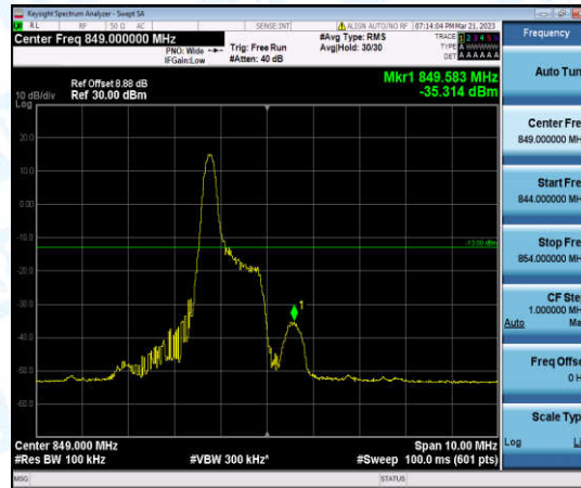
Band5-5MHz-QPSK-20625-1-0-High--35.31-PASS
