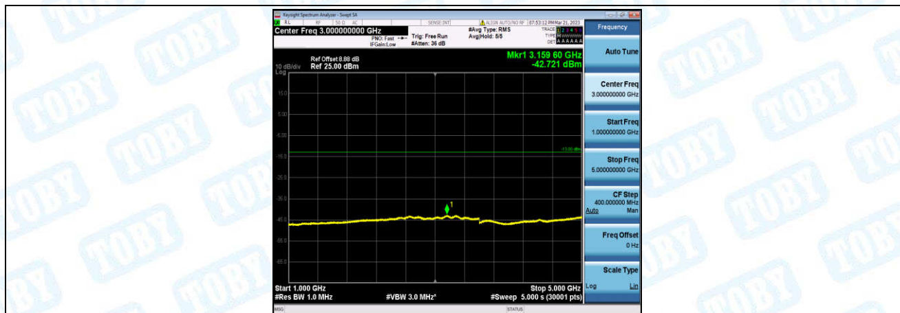
Band5-10MHz-QPSK-20600-1-0-High-1000-5000--42.72-PASS
