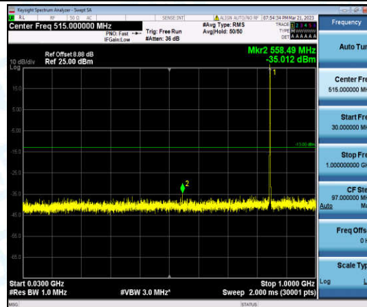
Band5-10MHz-16QAM-20600-1-0-High-30-1000--35.01-PASS
