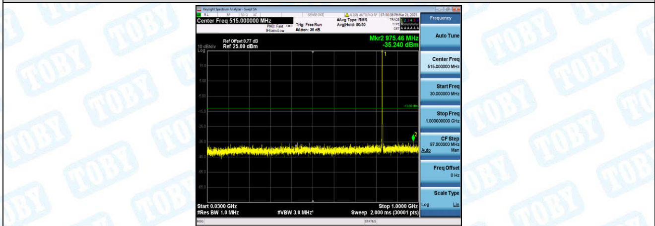
Band5-10MHz-16QAM-20525-1-0-Low-30-1000--35.24-PASS
