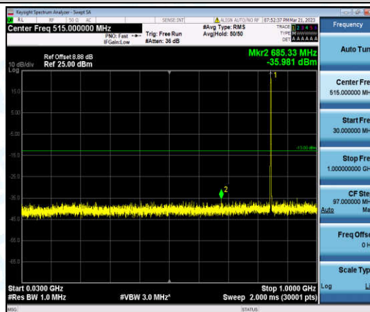
Band5-10MHz-QPSK-20600-1-0-High-30-1000--35.98-PASS
