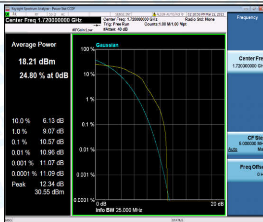
Band66-20MHz-16QAM-132072-1-0-Low-10.57-<=13-PASS
