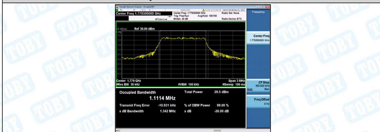
Band66-1.4MHz-QPSK-132665-6-0-High-1.1114-1.342-PASS
