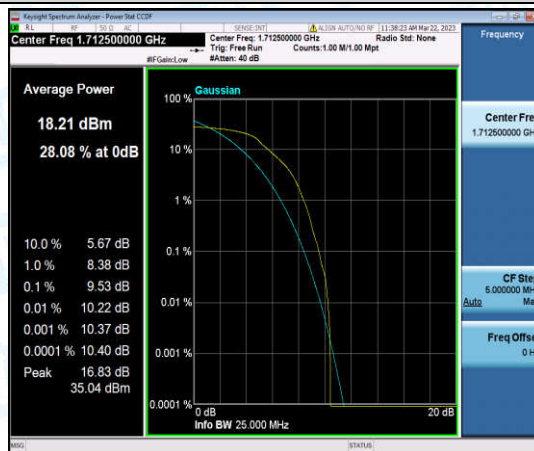
Band66-5MHz-QPSK-131997-6-0-Low-9.53-<=13-PASS
