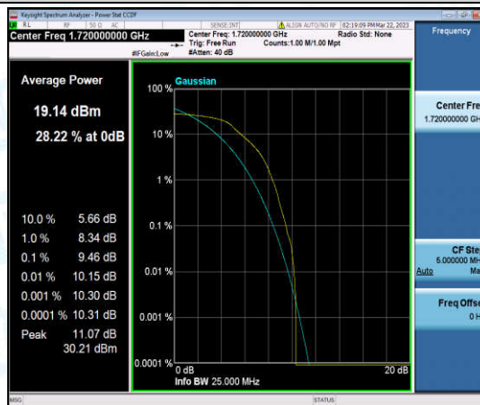
Band66-20MHz-16QAM-132072-6-0-Low-9.46-<=13-PASS
