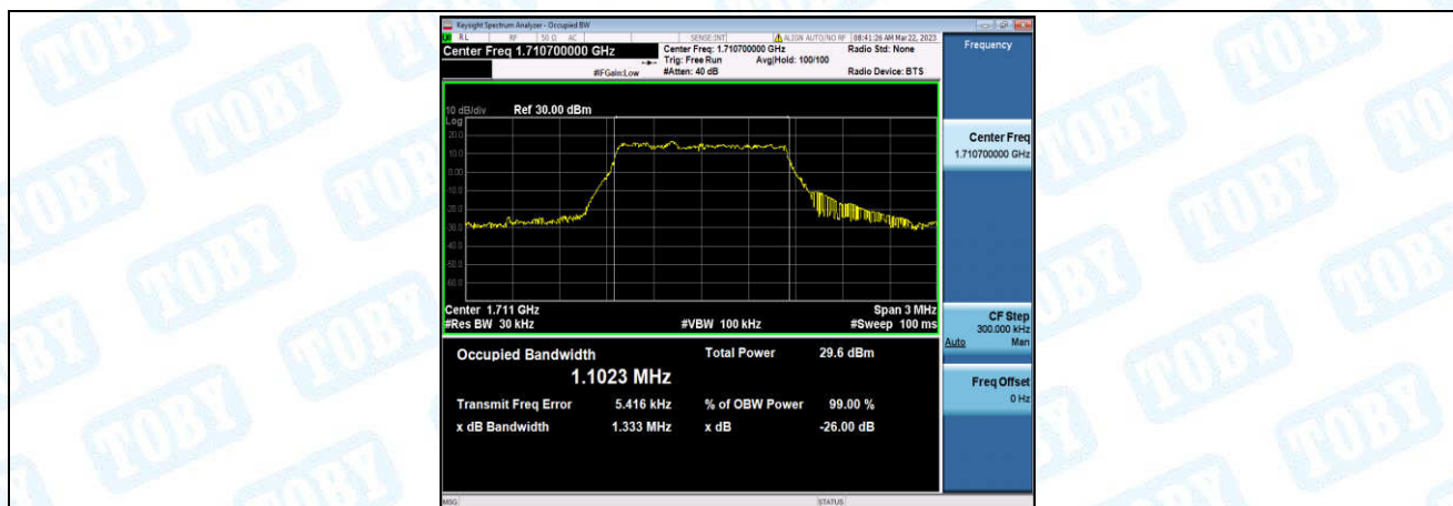
Band66-1.4MHz-QPSK-131979-6-0-Low-1.1023-1.333-PASS
