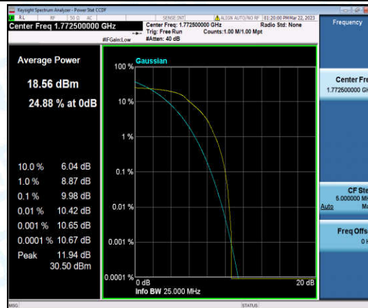
Band66-15MHz-QPSK-132597-6-0-High-9.98-<=13-PASS
