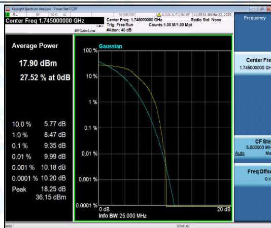
Band66-5MHz-16QAM-132322-6-0-Low-9.35-<=13-PASS
