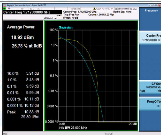
Band66-5MHz-QPSK-131997-1-0-Low-9.59-<=13-PASS
