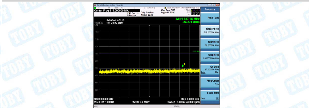
Band66-1.4MHz-QPSK-132322-1-0-Low-30-1000--34.37-PASS
