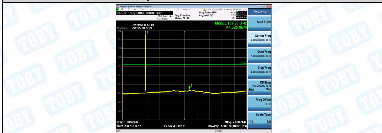
Band66-1.4MHz-QPSK-132322-1-0-Low-1000-5000--41.33-PASS
