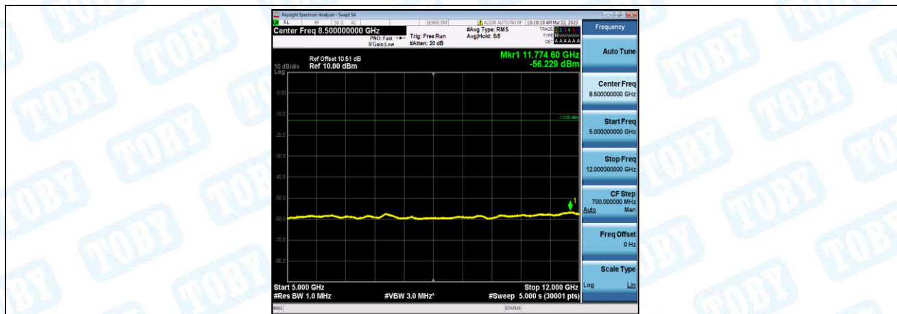
Band66-3MHz-16QAM-132322-1-0-Low-5000-12000--56.23-PASS
