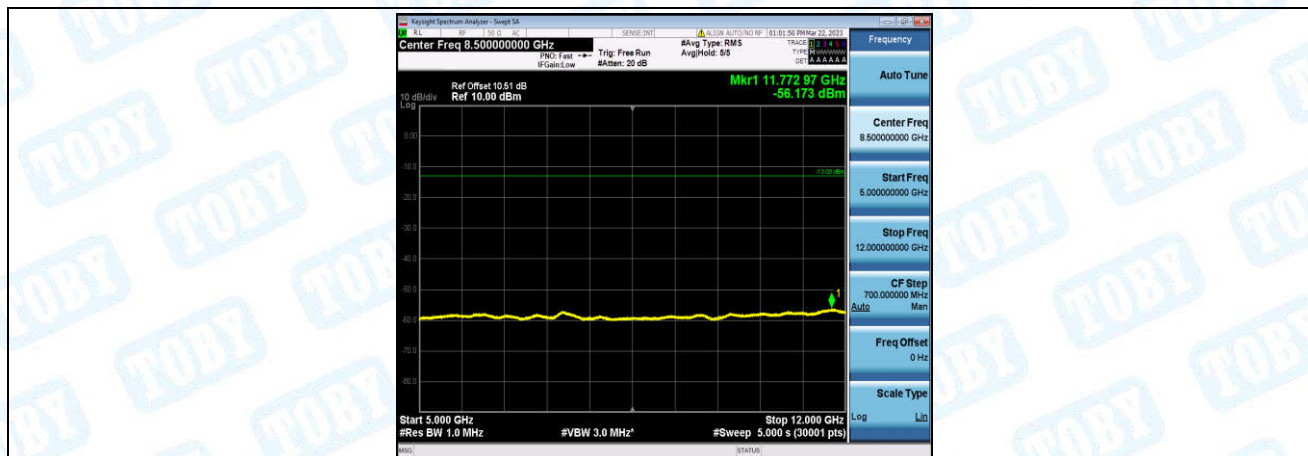
Band66-10MHz-16QAM-132322-1-0-Low-5000-12000--56.17-PASS
