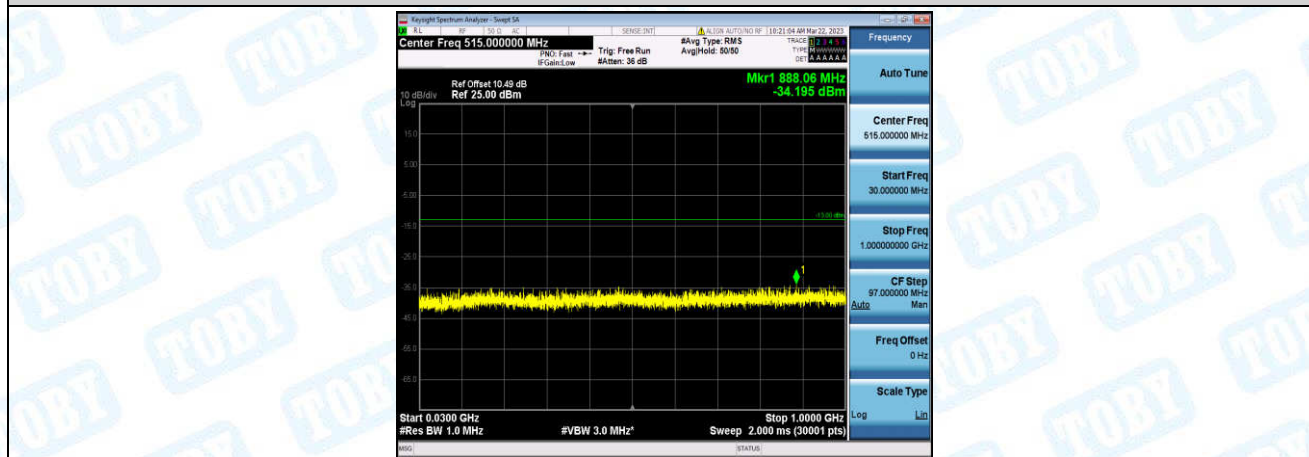
Band66-3MHz-16QAM-132657-1-0-High-30-1000--34.2-PASS
