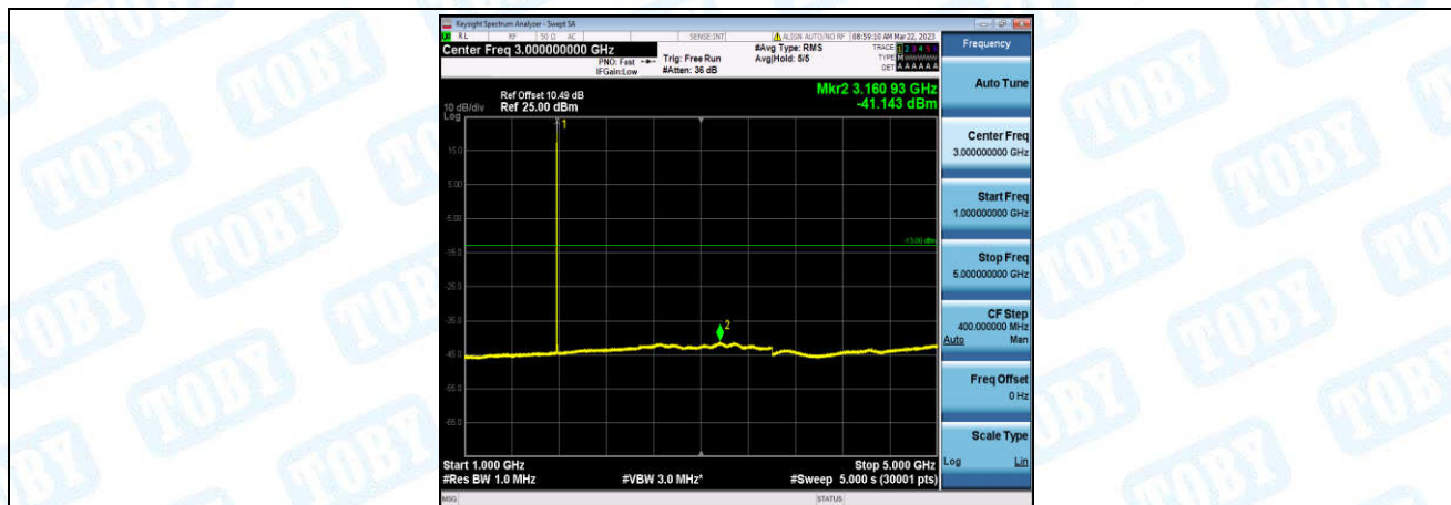
Band66-1.4MHz-16QAM-132665-1-0-High-1000-5000--41.14-PASS
