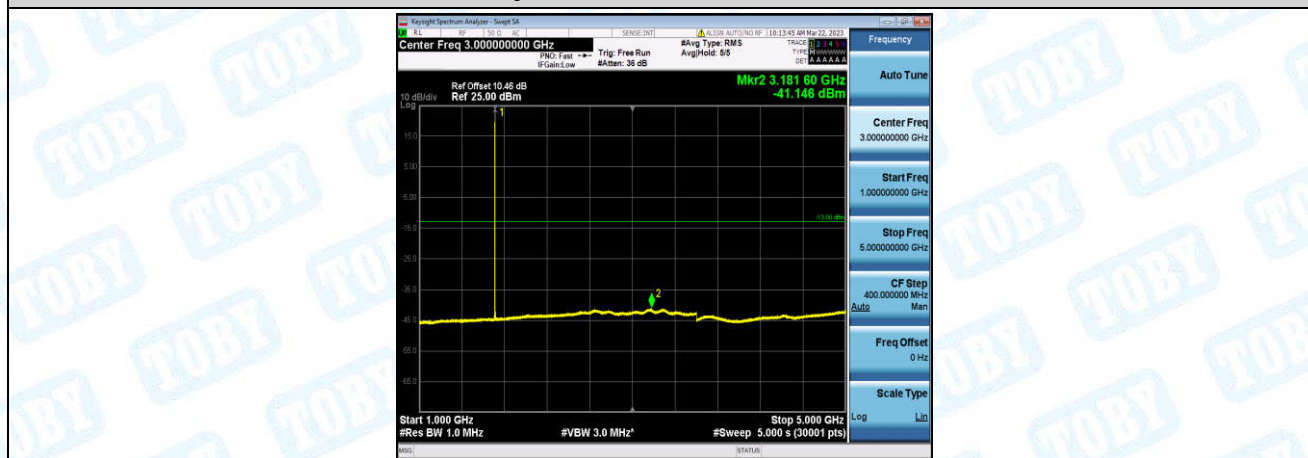
Band66-3MHz-16QAM-131987-1-0-Low-1000-5000--41.15-PASS
