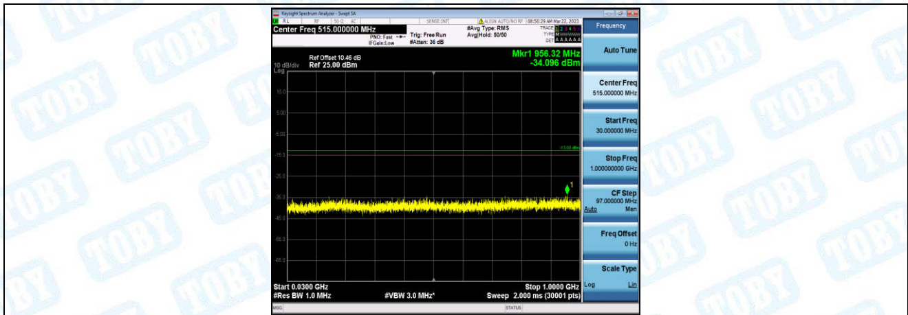
Band66-1.4MHz-16QAM-131979-1-0-Low-30-1000--34.1-PASS
