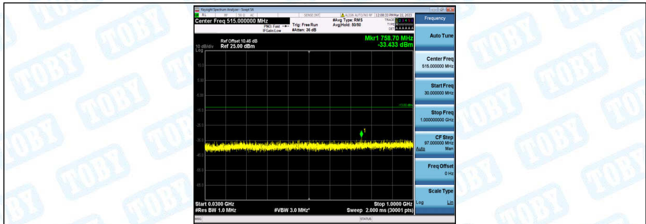
Band66-5MHz-16QAM-131997-1-0-Low-30-1000--33.43-PASS
