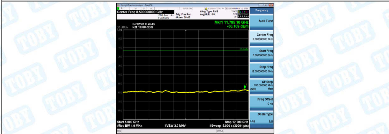
Band66-5MHz-QPSK-131997-1-0-Low-5000-12000--56.17-PASS
