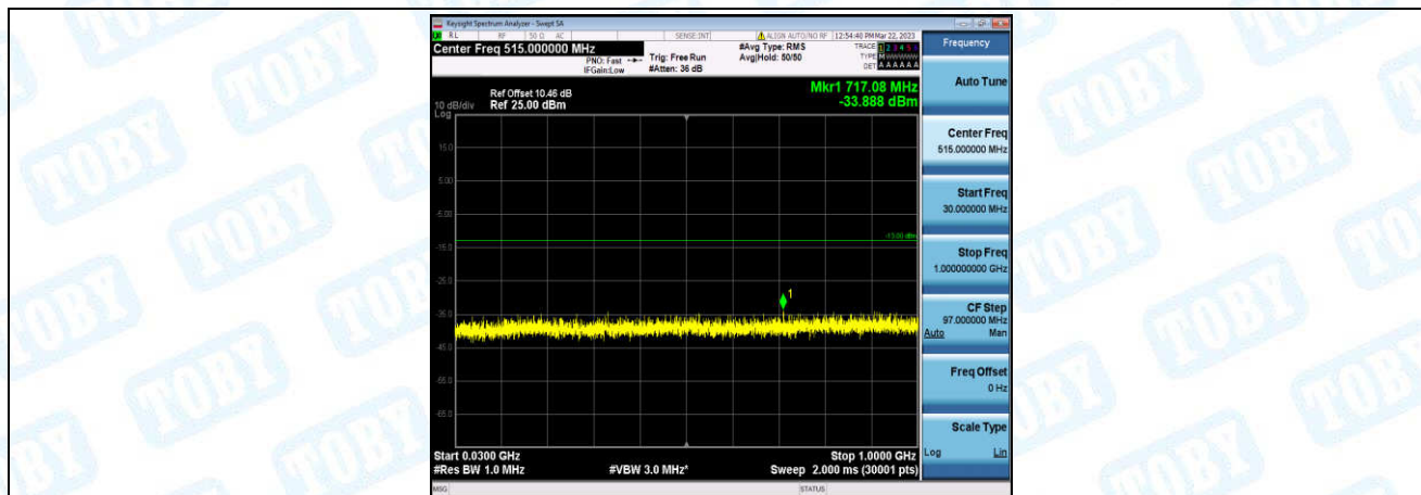
Band66-10MHz-QPSK-132022-1-0-Low-30-1000--33.89-PASS
