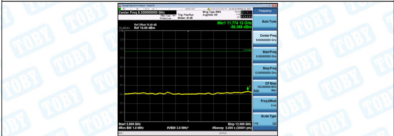
Band66-3MHz-QPSK-132657-1-0-High-5000-12000--56.37-PASS
