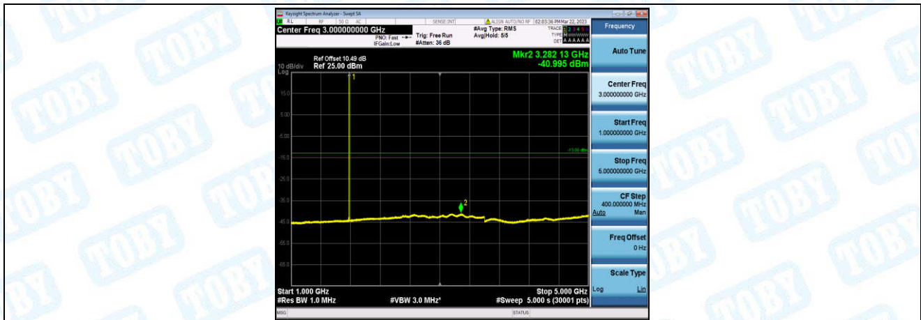
Band66-15MHz-QPSK-132597-1-0-High-1000-5000--41-PASS
