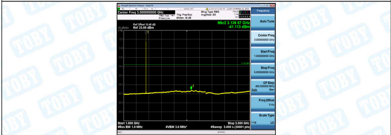
Band66-5MHz-QPSK-131997-1-0-Low-1000-5000--41.11-PASS
