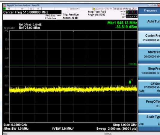
Band66-1.4MHz-QPSK-132665-1-0-High-30-1000--33.82-PASS
