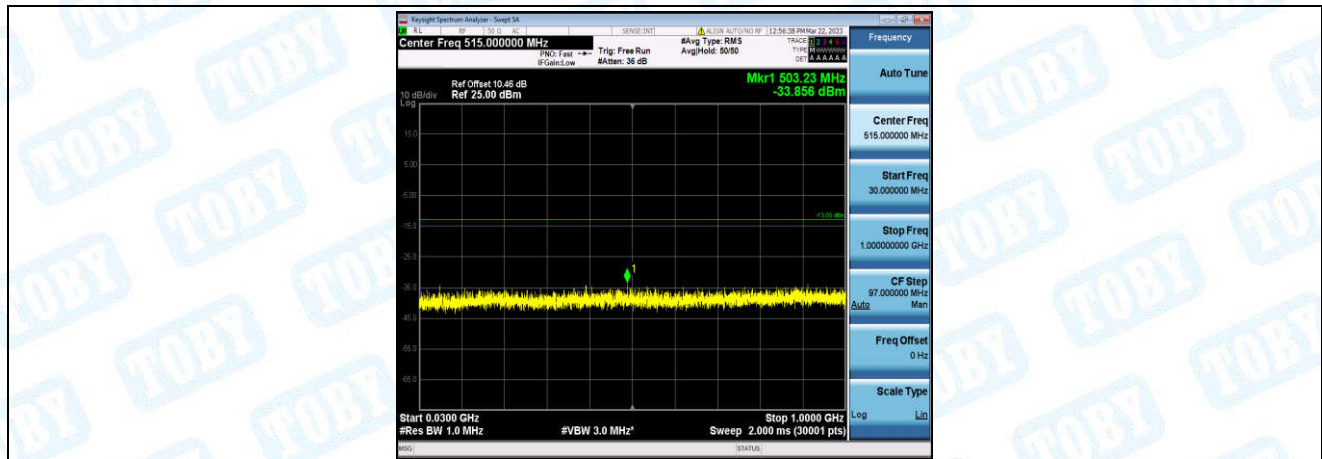
Band66-10MHz-16QAM-132022-1-0-Low-30-1000--33.86-PASS
