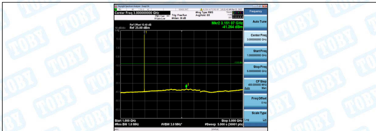
Band66-3MHz-16QAM-132657-1-0-High-1000-5000--41.26-PASS
