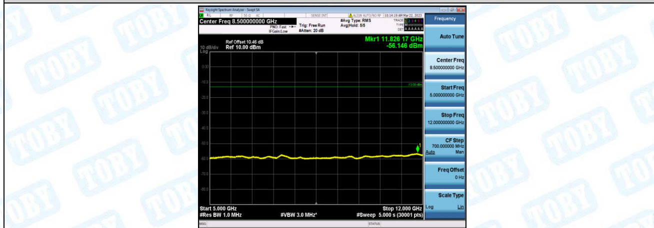
Band66-3MHz-16QAM-131987-1-0-Low-5000-12000--56.15-PASS
