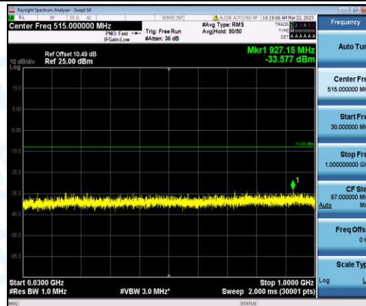
Band66-3MHz-QPSK-132657-1-0-High-30-1000--33.58-PASS
