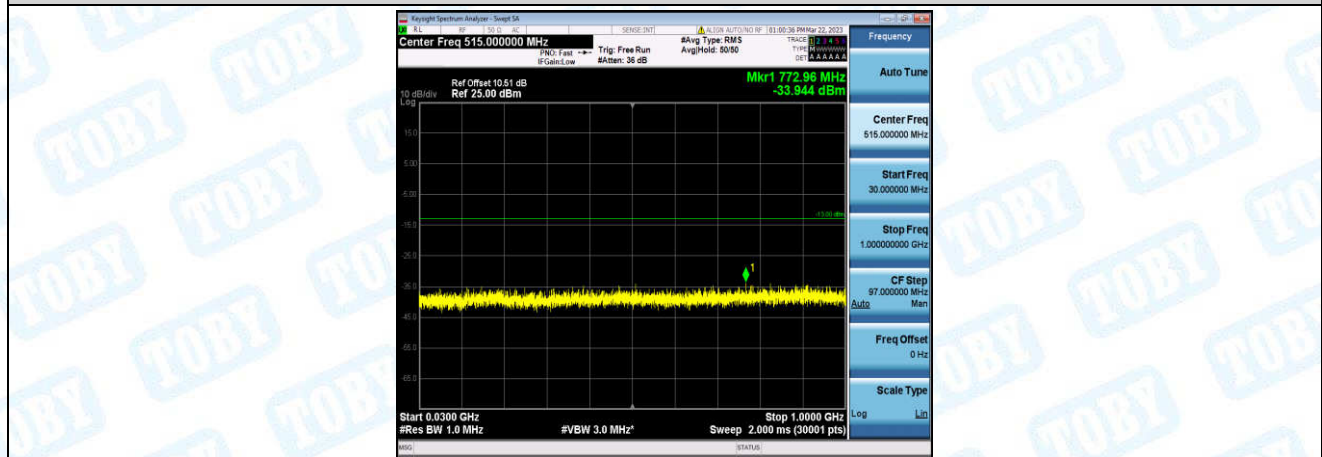
Band66-10MHz-16QAM-132322-1-0-Low-30-1000--33.94-PASS
