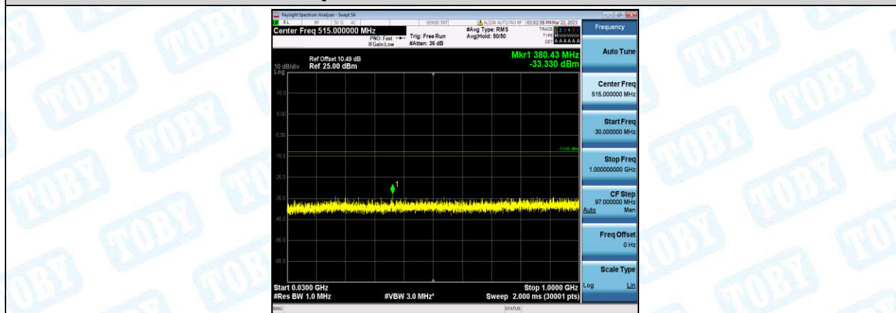
Band66-15MHz-QPSK-132597-1-0-High-30-1000--33.33-PASS
