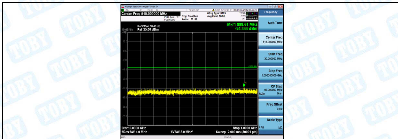
Band66-3MHz-16QAM-131987-1-0-Low-30-1000--34.44-PASS
