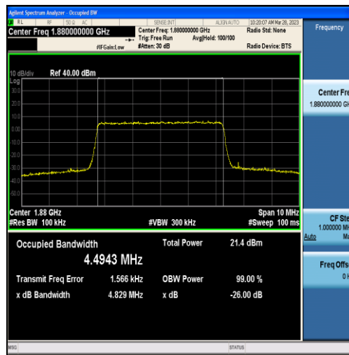
Band2-5MHz-16QAM-18900-25RB#0-4.4943
