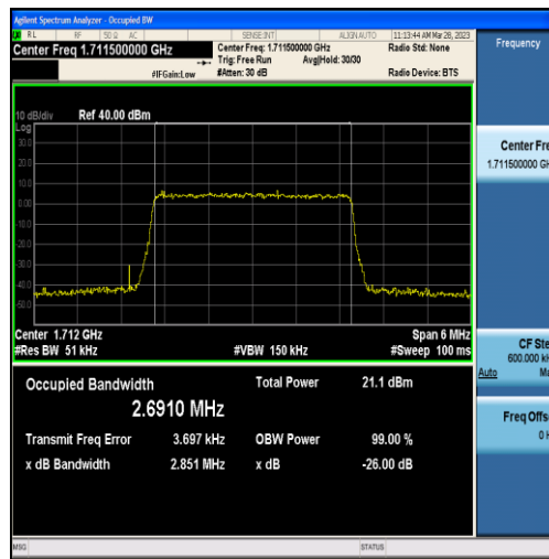
Band4-3MHz-QPSK-19965-15RB#0-2.6910
