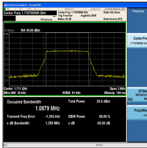
Band4-1.4MHz-16QAM-19957-6RB#0-1.0879
