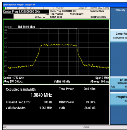
Band4-1.4MHz-16QAM-20175-6RB#0-1.0849
