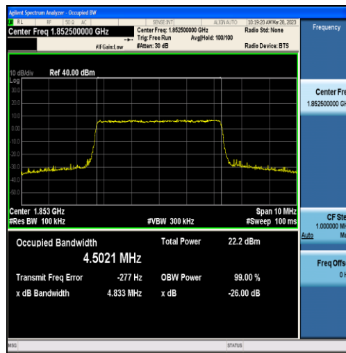
Band2-5MHz-QPSK-18625-25RB#0-4.5021
