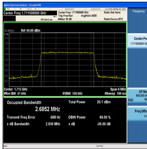
Band4-3MHz-16QAM-19965-15RB#0-2.6852
