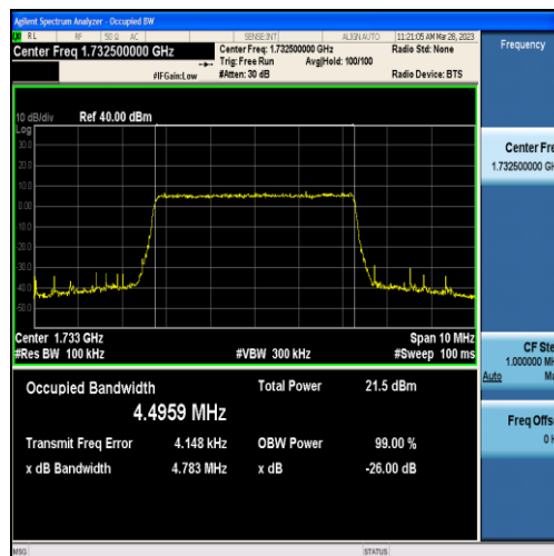
Band4-5MHz-QPSK-20175-25RB#0-4.4959
