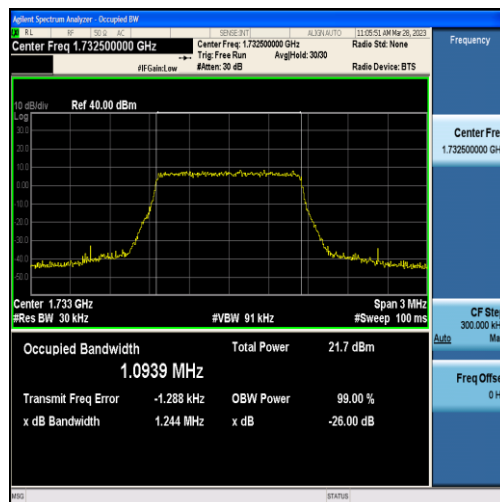
Band4-1.4MHz-QPSK-20175-6RB#0-1.0939
