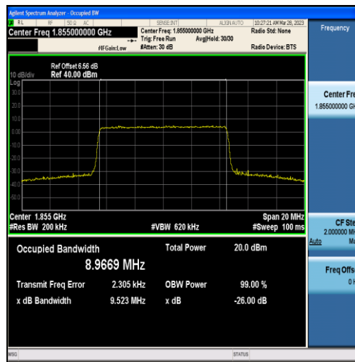
Band2-10MHz-16QAM-18650-50RB#0-8.9669
