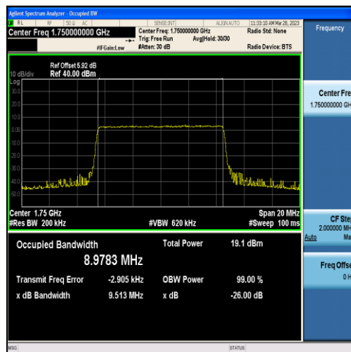
Band4-10MHz-16QAM-20350-50RB#0-8.9783
