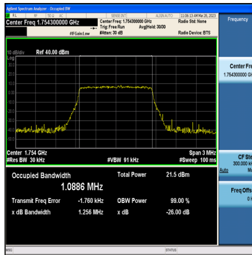
Band4-1.4MHz-QPSK-20393-6RB#0-1.0886
