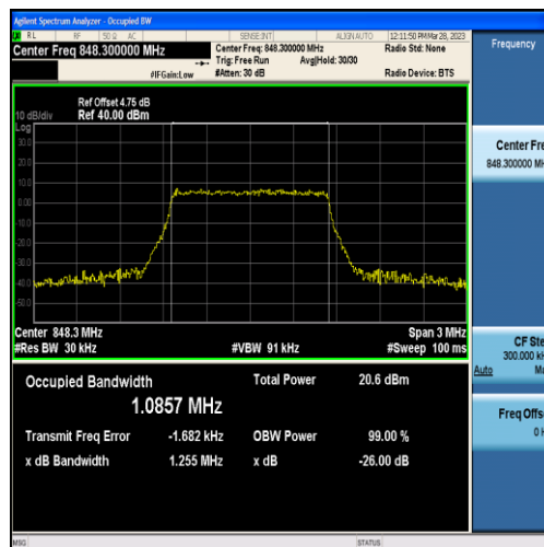
Band5-1.4MHz-16QAM-20643-6RB#0-1.0857
