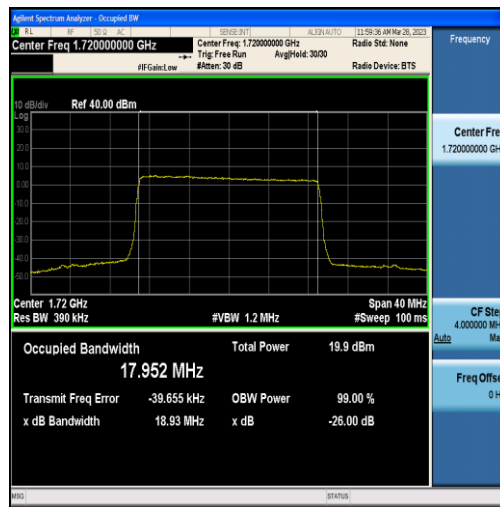
Band4-20MHz-QPSK-20050-100RB#0-17.952
