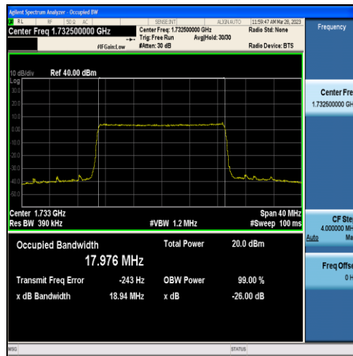
Band4-20MHz-QPSK-20175-100RB#0-17.976
