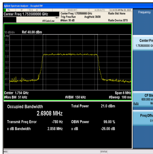
Band4-3MHz-QPSK-20385-15RB#0-2.6908
