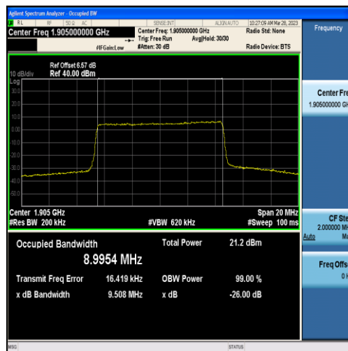
Band2-10MHz-QPSK-19150-50RB#0-8.9954
