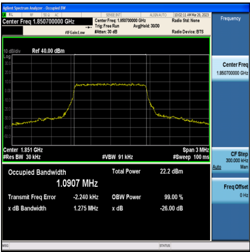
Band2-1.4MHz-QPSK-18607-6RB#0-1.0907
