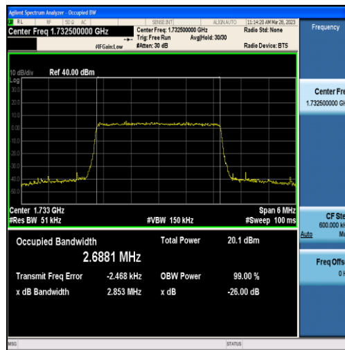
Band4-3MHz-16QAM-20175-15RB#0-2.6881
