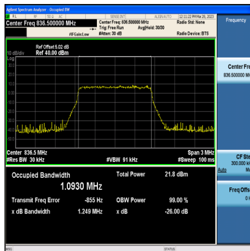
Band5-1.4MHz-QPSK-20525-6RB#0-1.0930
