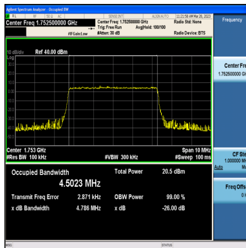
Band4-5MHz-16QAM-20375-25RB#0-4.5023
