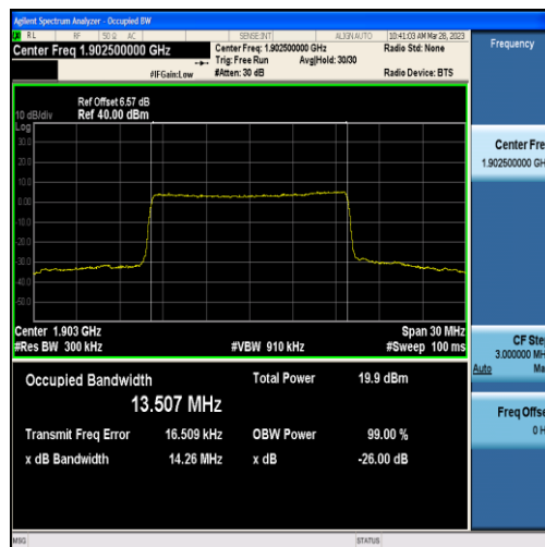
Band2-15MHz-16QAM-19125-75RB#0-13.507
