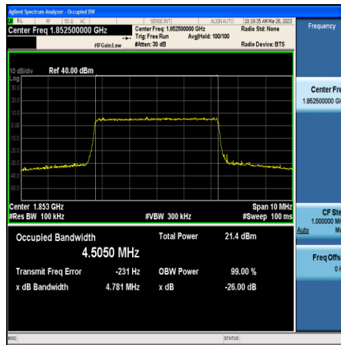
Band2-5MHz-16QAM-18625-25RB#0-4.5050
