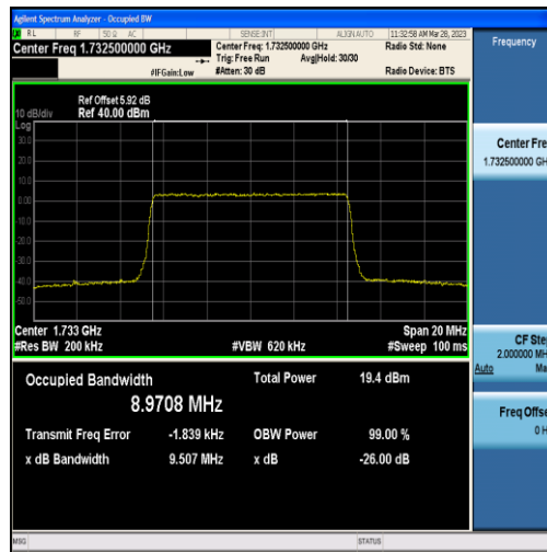
Band4-10MHz-16QAM-20175-50RB#0-8.9708
