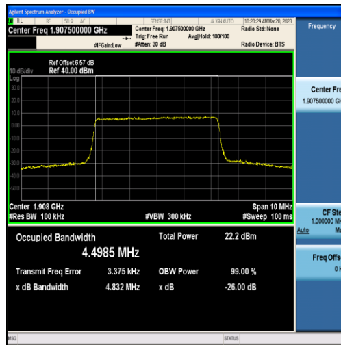
Band2-5MHz-QPSK-19175-25RB#0-4.4985
