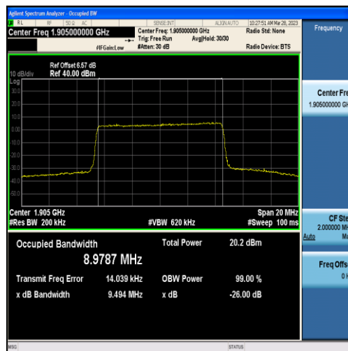
Band2-10MHz-16QAM-19150-50RB#0-8.9787
