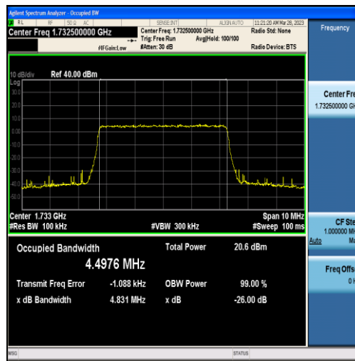
Band4-5MHz-16QAM-20175-25RB#0-4.4976
