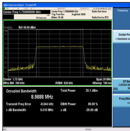
Band4-10MHz-QPSK-20350-50RB#0-8.9888
