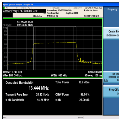
Band4-15MHz-16QAM-20325-75RB#0-13.444
