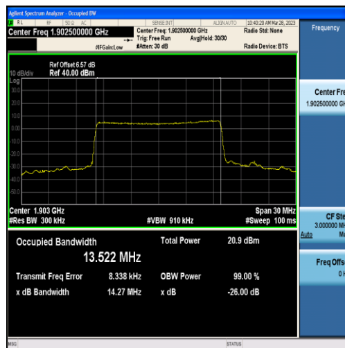
Band2-15MHz-QPSK-19125-75RB#0-13.522
