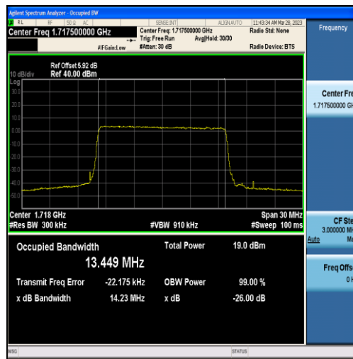
Band4-15MHz-16QAM-20025-75RB#0-13.449
