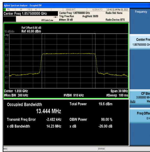
Band2-15MHz-16QAM-18675-75RB#0-13.444
