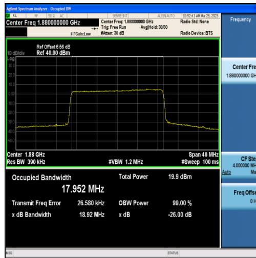
Band2-20MHz-16QAM-18900-100RB#0-17.952
