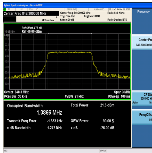
Band5-1.4MHz-QPSK-20643-6RB#0-1.0866
