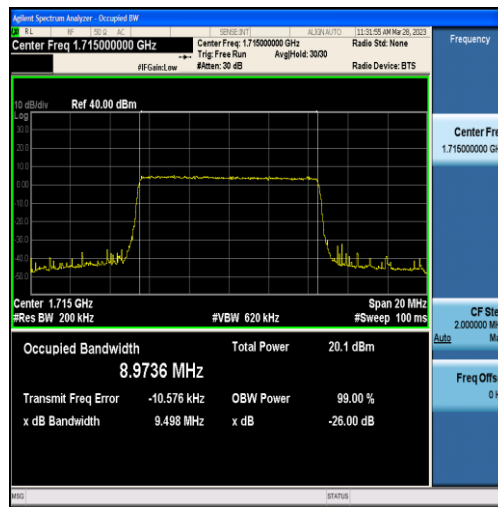
Band4-10MHz-QPSK-20000-50RB#0-8.9736
