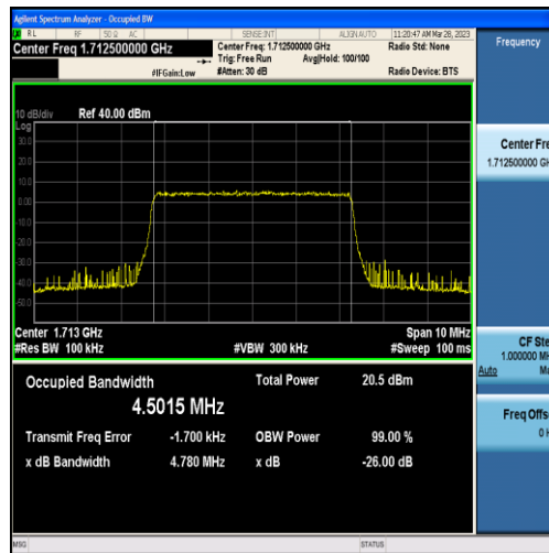
Band4-5MHz-16QAM-19975-25RB#0-4.5015
