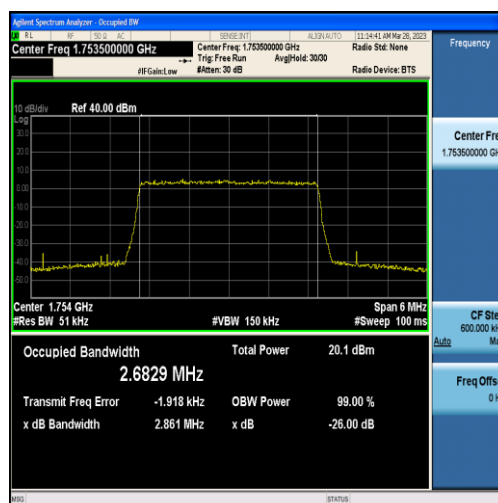
Band4-3MHz-16QAM-20385-15RB#0-2.6829
