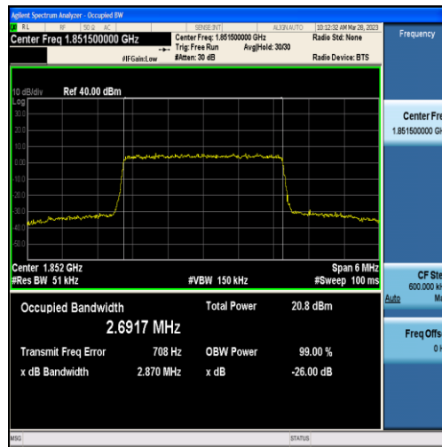
Band2-3MHz-16QAM-18615-15RB#0-2.6917
