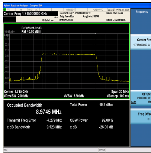
Band4-10MHz-16QAM-20000-50RB#0-8.9745
