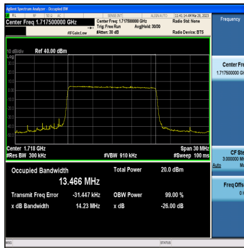
Band4-15MHz-QPSK-20025-75RB#0-13.466
