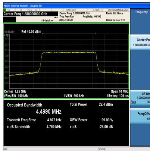
Band2-5MHz-QPSK-18900-25RB#0-4.4990
