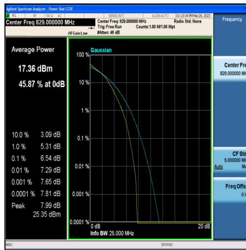
Band5-10MHz-16QAM-20450-50RB#0
