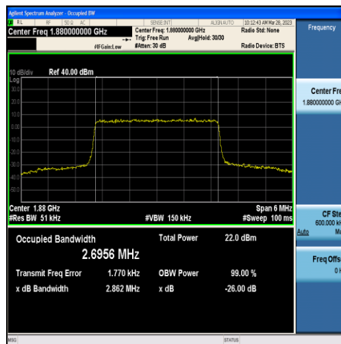
Band2-3MHz-QPSK-18900-15RB#0-2.6956
