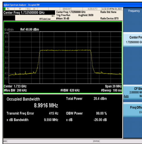
Band4-10MHz-QPSK-20175-50RB#0-8.9916
