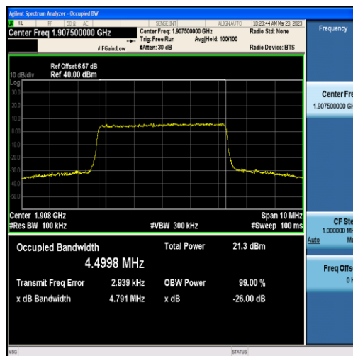
Band2-5MHz-16QAM-19175-25RB#0-4.4998
