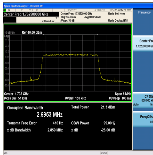
Band4-3MHz-QPSK-20175-15RB#0-2.6953
