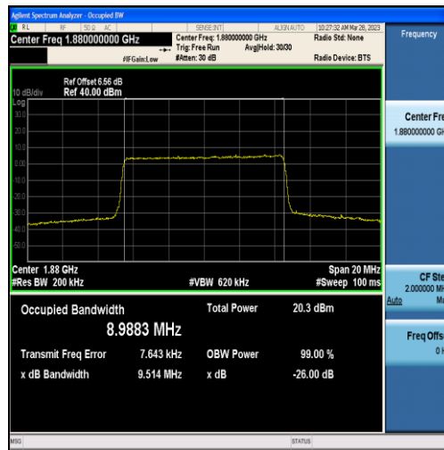
Band2-10MHz-16QAM-18900-50RB#0-8.9883
