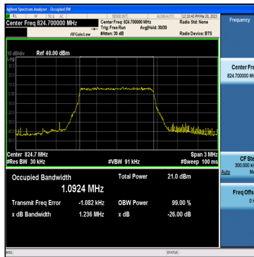
Band5-1.4MHz-QPSK-20407-6RB#0-1.0924
