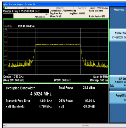
Band4-5MHz-QPSK-20375-25RB#0-4.5024
