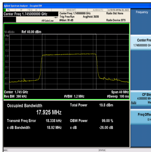
Band4-20MHz-QPSK-20300-100RB#0-17.925
