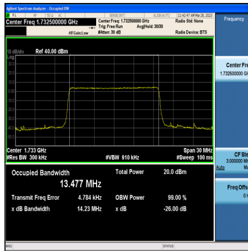
Band4-15MHz-QPSK-20175-75RB#0-13.477
