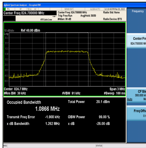
Band5-1.4MHz-16QAM-20407-6RB#0-1.0866
