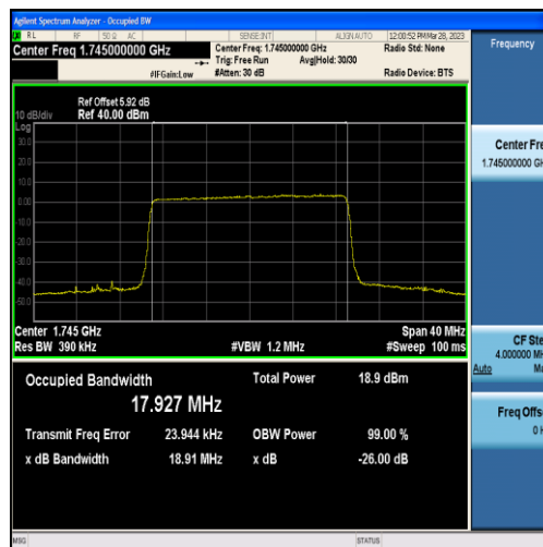
Band4-20MHz-16QAM-20300-100RB#0-17.927
