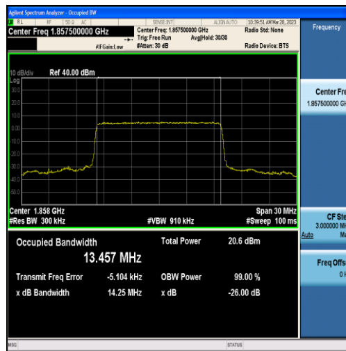
Band2-15MHz-QPSK-18675-75RB#0-13.457
