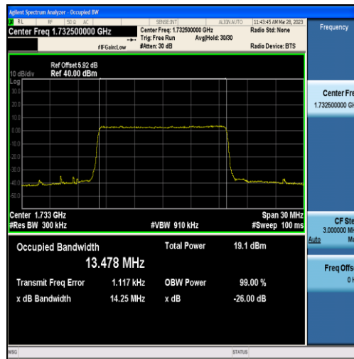
Band4-15MHz-16QAM-20175-75RB#0-13.478
