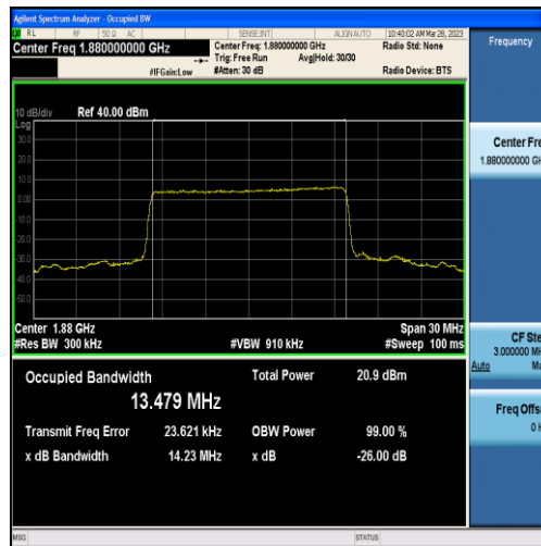
Band2-15MHz-QPSK-18900-75RB#0-13.479
