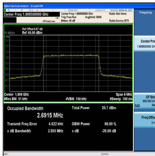
Band2-3MHz-16QAM-19185-15RB#0-2.6915
