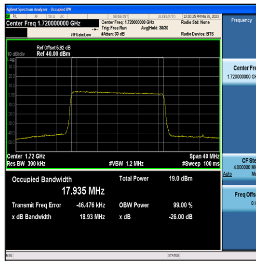
Band4-20MHz-16QAM-20050-100RB#0-17.935
