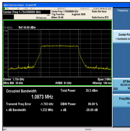
Band4-1.4MHz-16QAM-20393-6RB#0-1.0873
