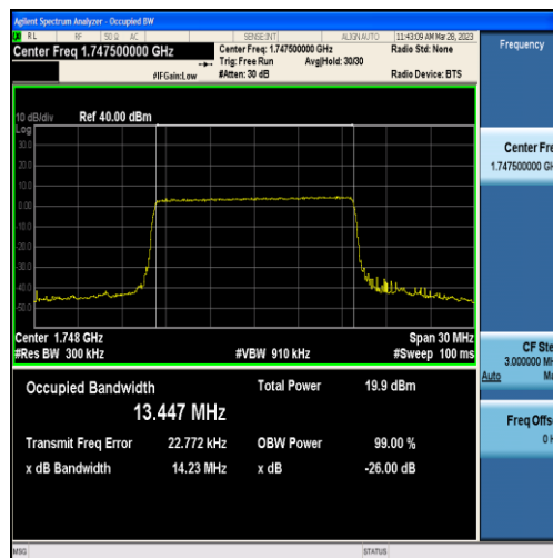
Band4-15MHz-QPSK-20325-75RB#0-13.447
