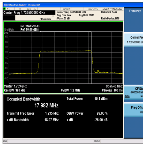
Band4-20MHz-16QAM-20175-100RB#0-17.982
