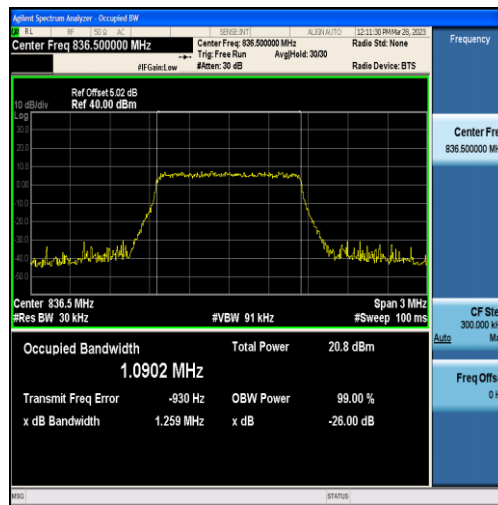
Band5-1.4MHz-16QAM-20525-6RB#0-1.0902
