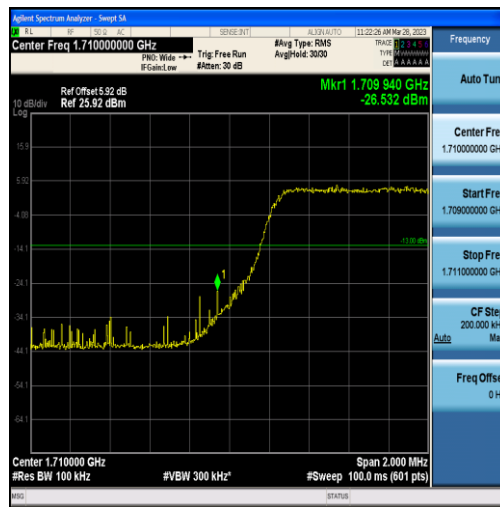
Band4-5MHz-16QAM-19975-25RB#0
