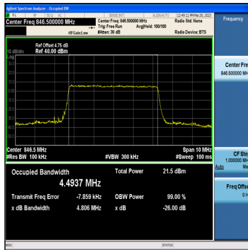
Band5-5MHz-QPSK-20625-25RB#0-4.4937
