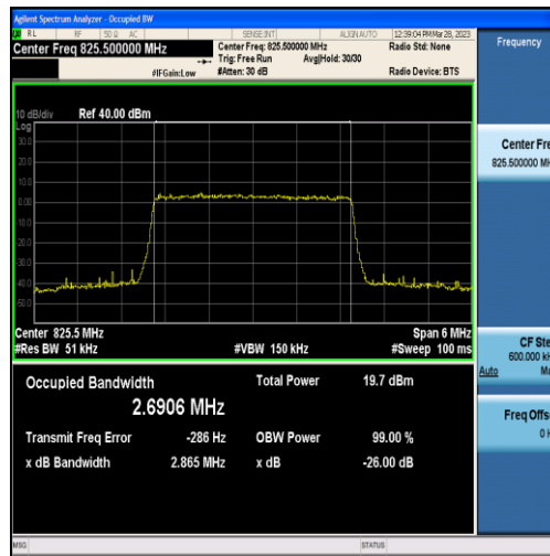
Band5-3MHz-16QAM-20415-15RB#0-2.6906
