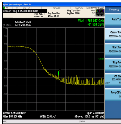
Band4-10MHz-16QAM-20350-50RB#0
