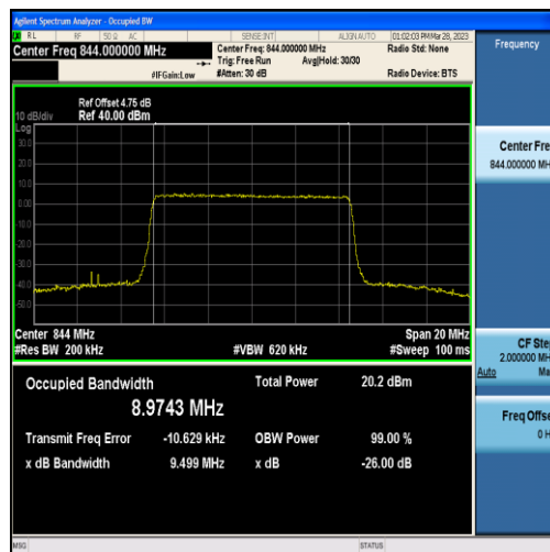
Band5-10MHz-QPSK-20600-50RB#0-8.9743
