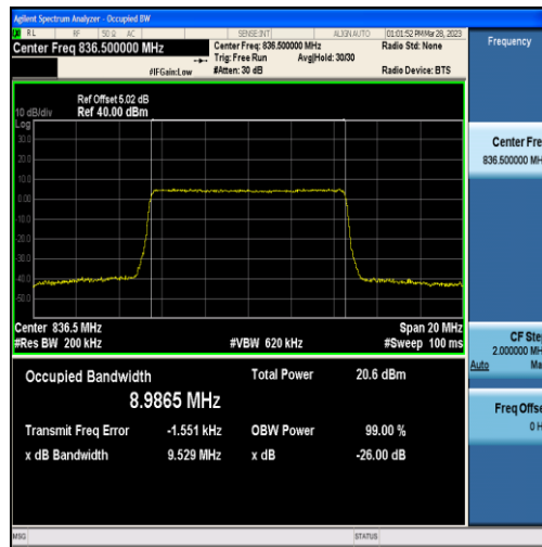
Band5-10MHz-QPSK-20525-50RB#0-8.9865
