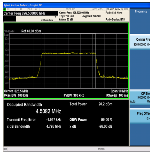
Band5-5MHz-16QAM-20425-25RB#0-4.5082
