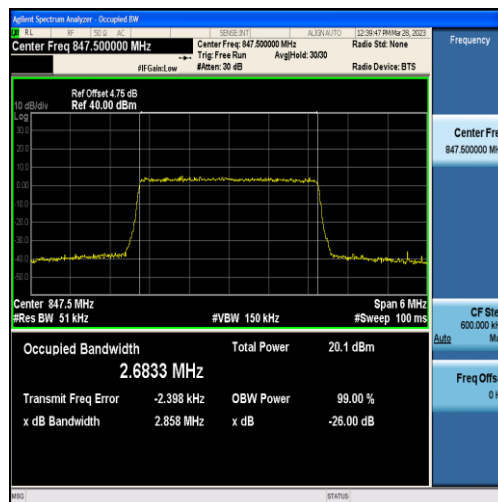
Band5-3MHz-16QAM-20635-15RB#0-2.6833
