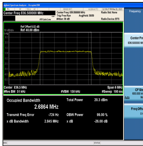
Band5-3MHz-16QAM-20525-15RB#0-2.6864
