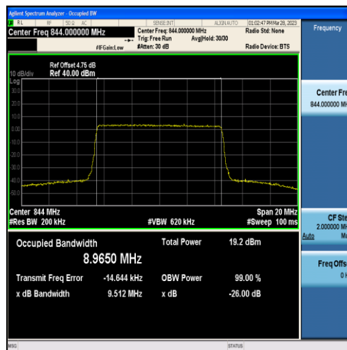
Band5-10MHz-16QAM-20600-50RB#0-8.9650
