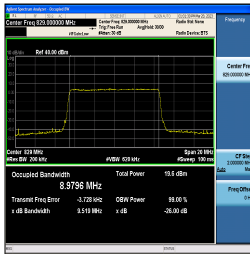
Band5-10MHz-QPSK-20450-50RB#0-8.9796
