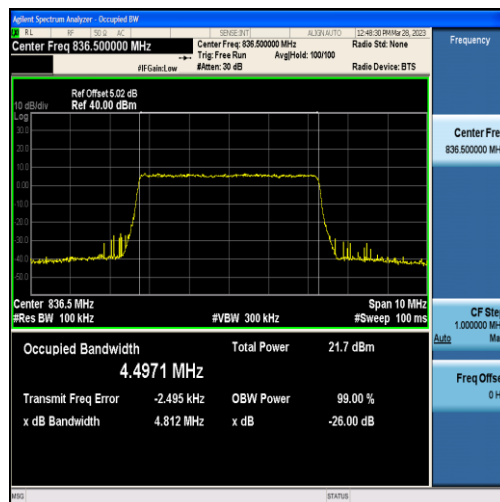
Band5-5MHz-QPSK-20525-25RB#0-4.4971
