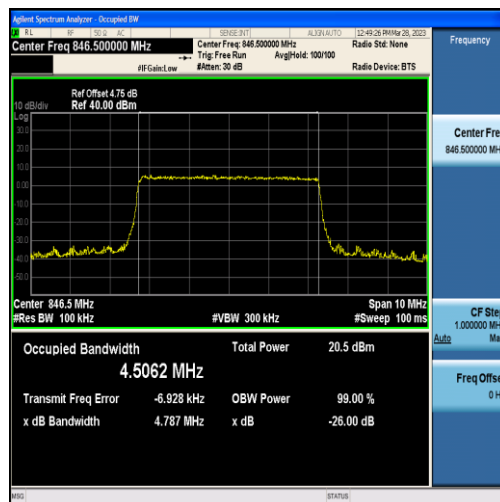
Band5-5MHz-16QAM-20625-25RB#0-4.5062
