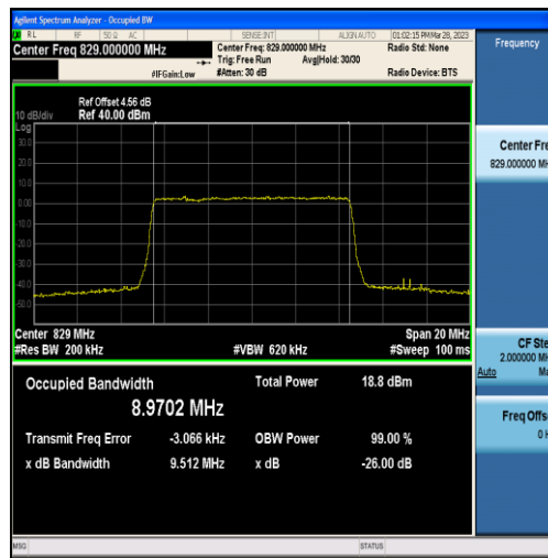
Band5-10MHz-16QAM-20450-50RB#0-8.9702
