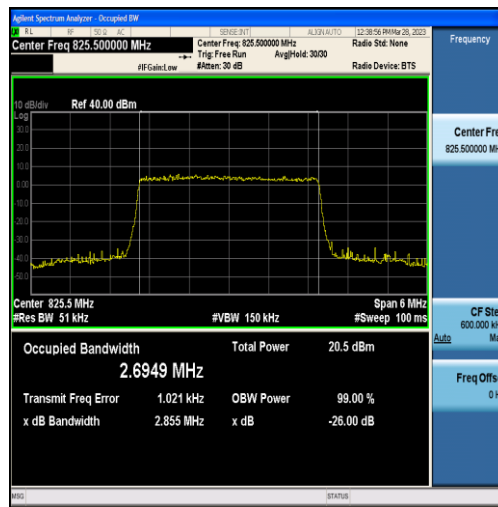
Band5-3MHz-QPSK-20415-15RB#0-2.6949
