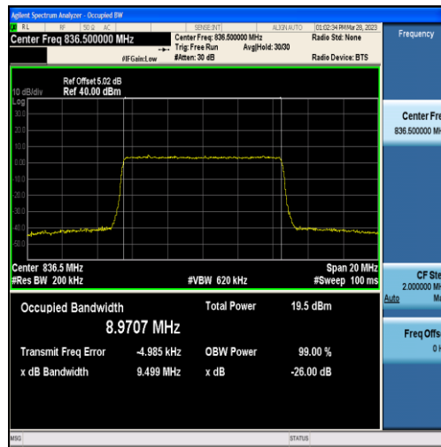
Band5-10MHz-16QAM-20525-50RB#0-8.9707
