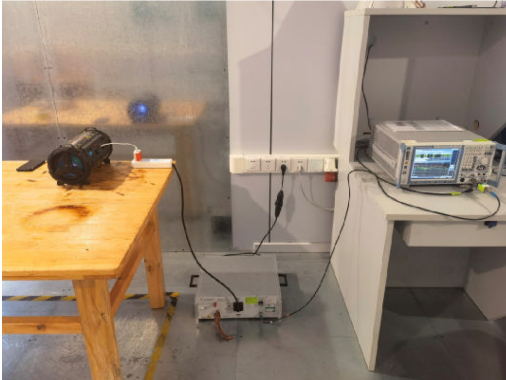
Setup Photo FCC ID: 2BAPK-M18
