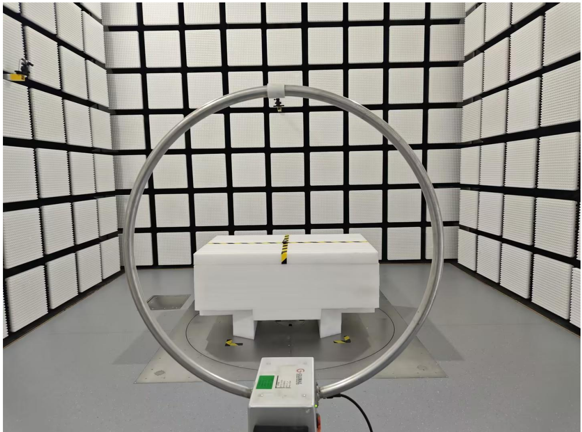
Radiated Emission 9 kHz-30 MHz Parallel View
