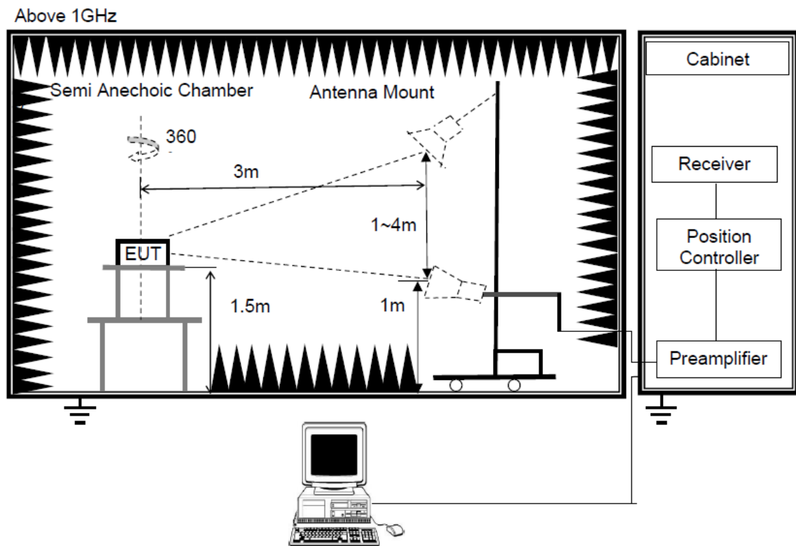
(A) Radiated Emission Test Set-Up, Frequency above 1GHz
