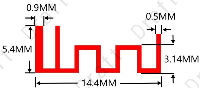
Antenna Dimensions
