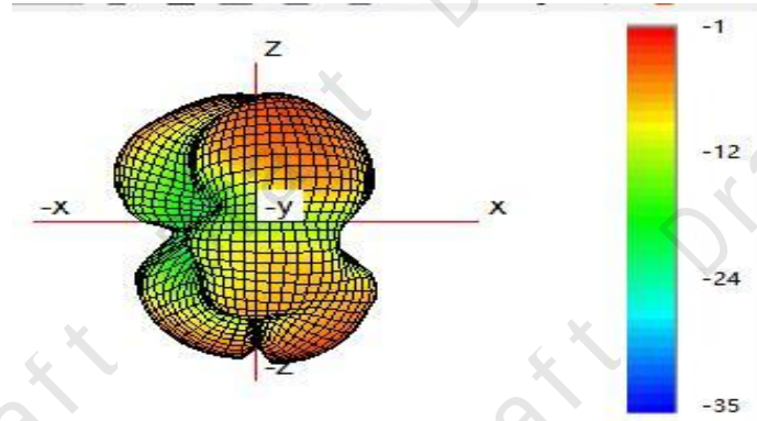
(4) Typical Free Space 3D Radiation Pattern at 2400MHz(unit:dBi)
