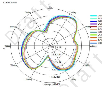
(1) X-Y Plane(unit:dBi):
