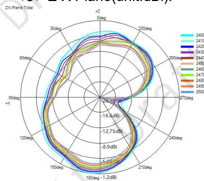
(3) Z-X Plane(unit:dBi):
