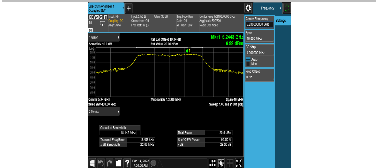
11N20SISO_Ant1_5240
