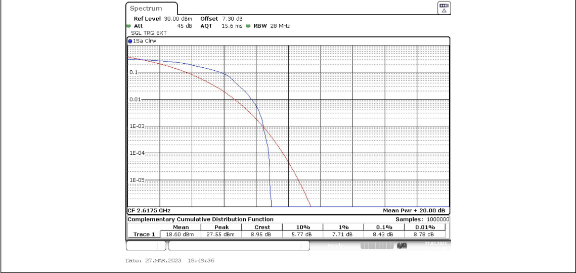
Band38-5MHz-16QAM-38225-25RB#0
