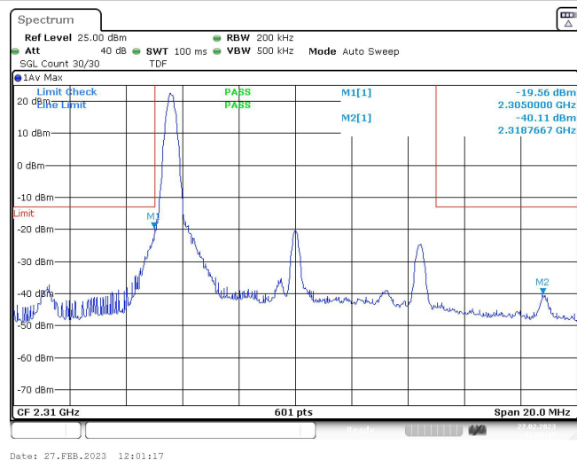
Band40-10MHz-QPSK-38750-1RB#49
