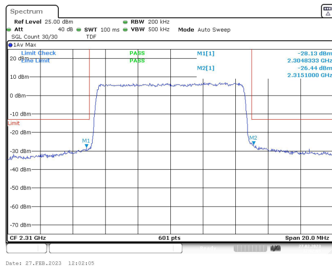
Band40-10MHz-16QAM-38750-1RB#0
