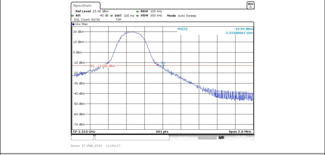
Band40-5MHz-16QAM-38775-25RB#0
