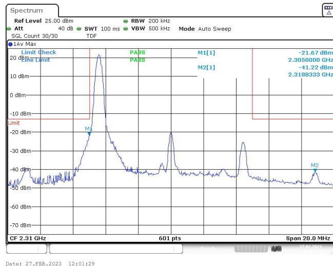
Band40-10MHz-16QAM-38750-1RB#49
