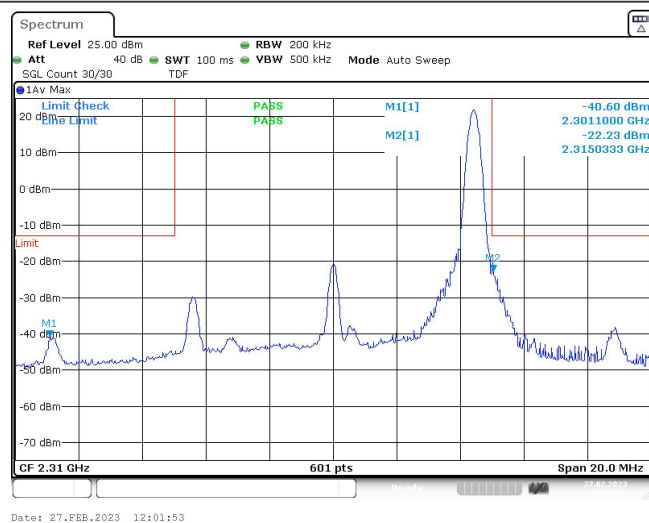
Band40-10MHz-16QAM-38750-50RB#0
