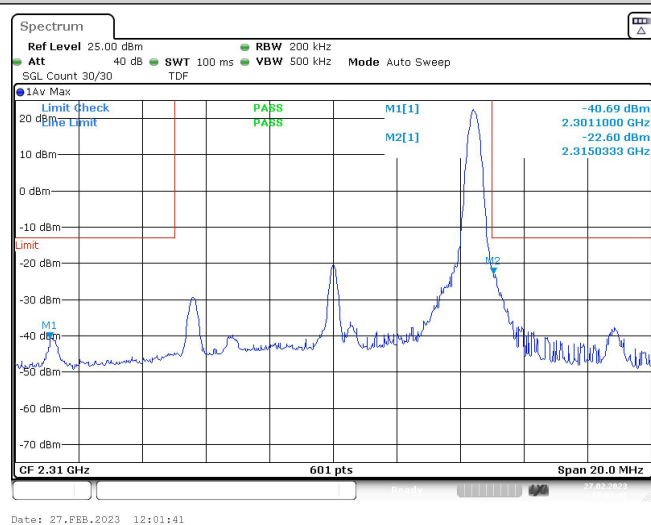
Band40-10MHz-QPSK-38750-50RB#0
