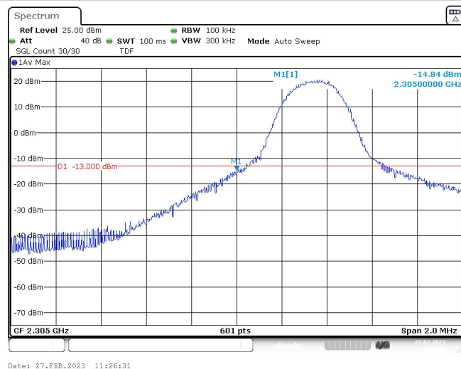
Band40-5MHz-16QAM-38725-1RB#24
