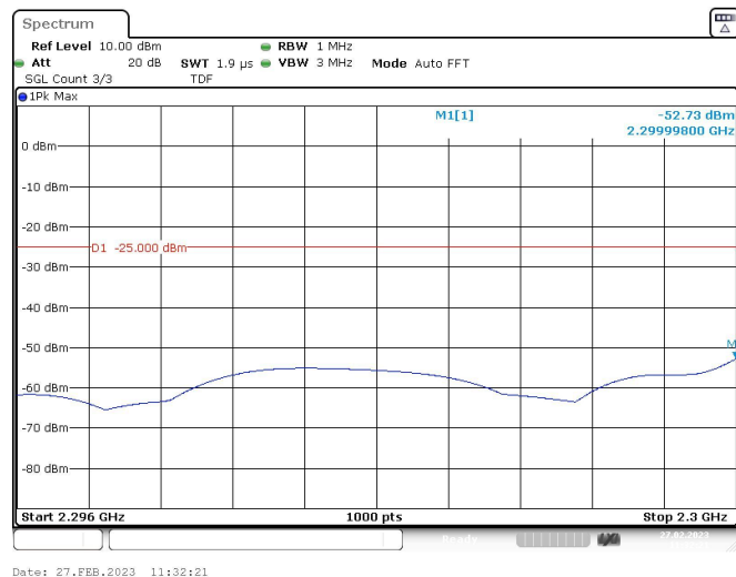
Band40-5MHz-16QAM-38725-1RB#0-Range6:2300~2305MHz
