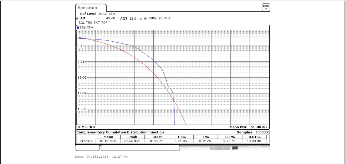
Band41-5MHz-16QAM-40690-25RB#0
