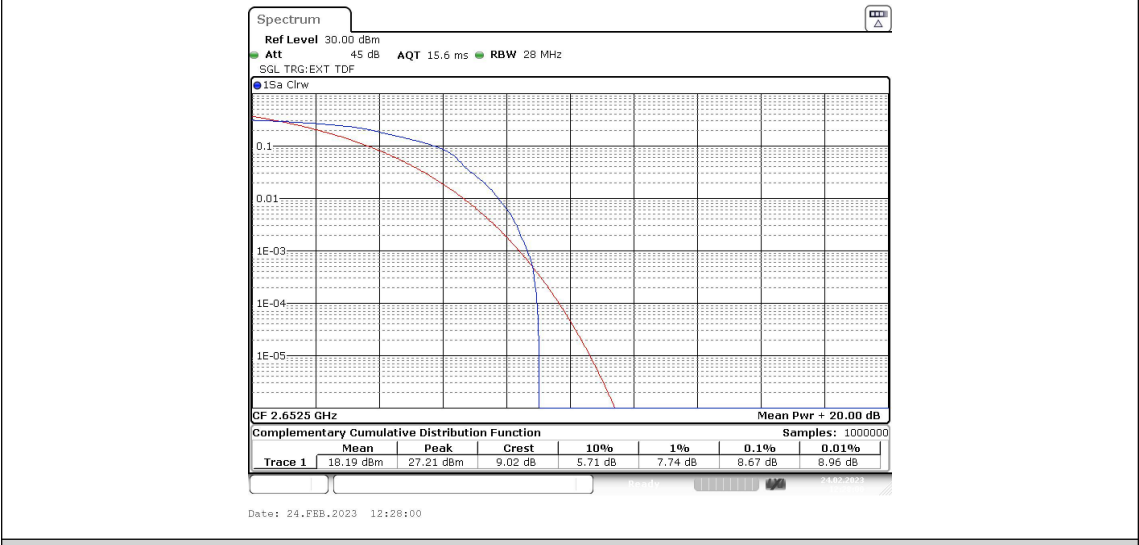
Band41-5MHz-16QAM-41215-25RB#0
