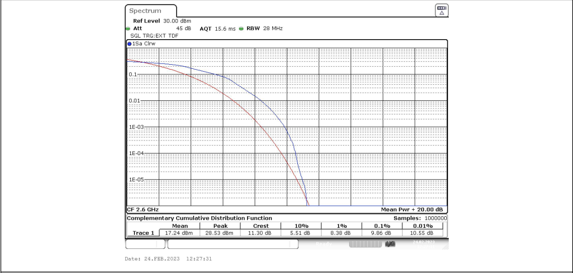
Band41-5MHz-16QAM-41215-1RB#0
