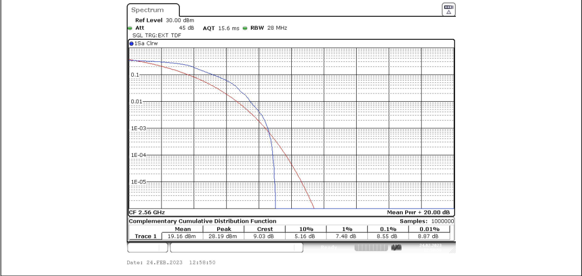
Band41-10MHz-QPSK-40290-50RB#0
