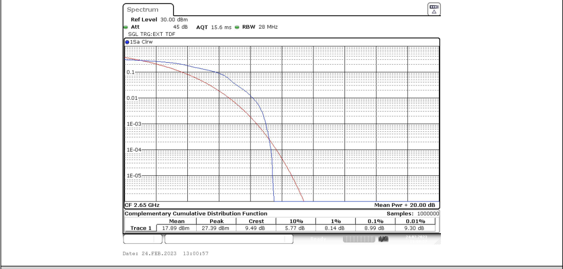
Band41-10MHz-16QAM-41190-50RB#0
