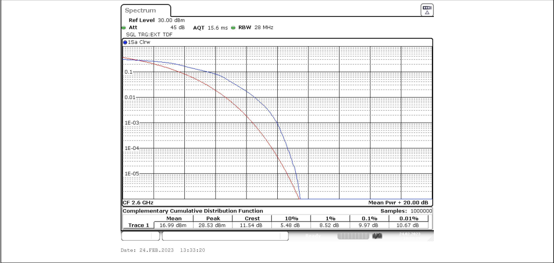
Band41-15MHz-16QAM-41165-1RB#0
