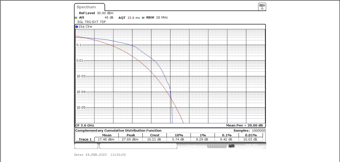
Band41-15MHz-16QAM-40690-75RB#0
