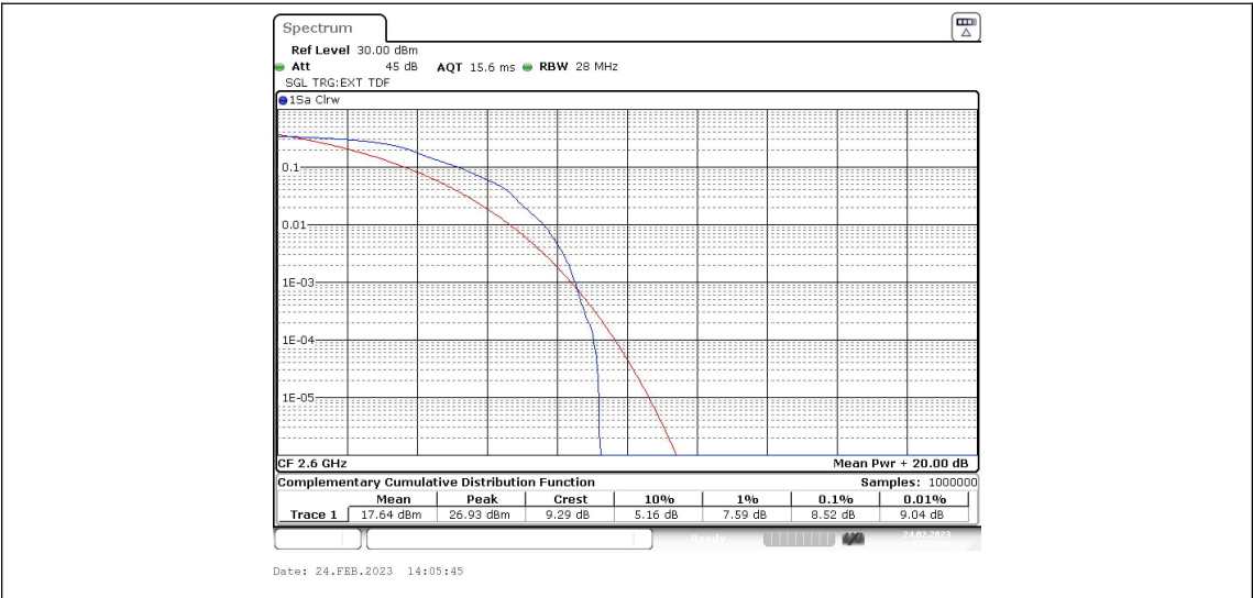
Band41-20MHz-QPSK-40690-100RB#0
