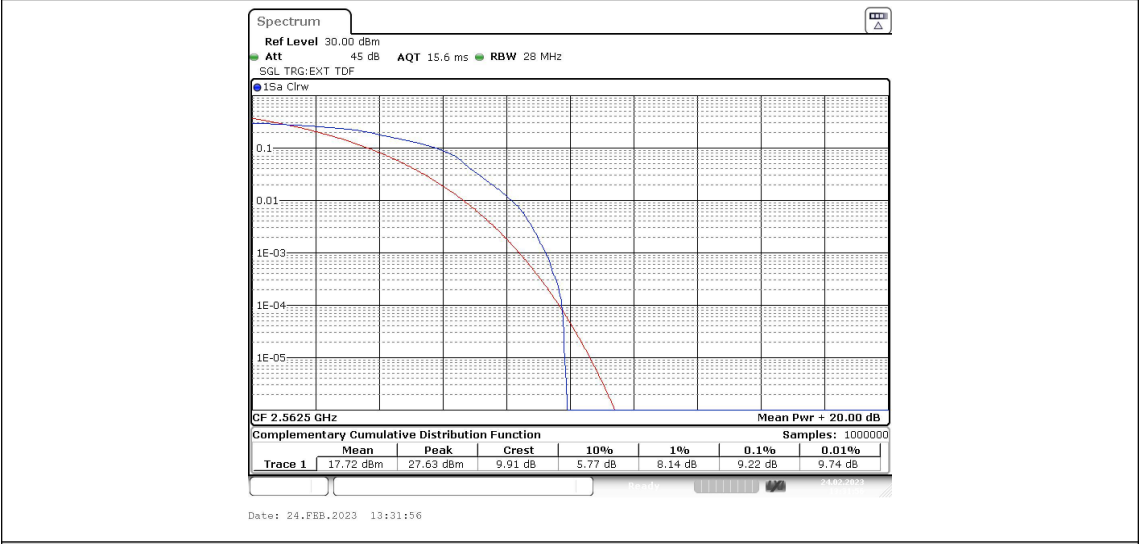
Band41-15MHz-16QAM-40315-75RB#0
