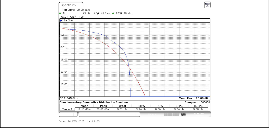
Band41-20MHz-16QAM-40340-100RB#0
