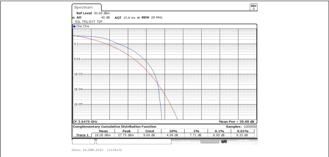
Band41-15MHz-16QAM-40315-1RB#0
