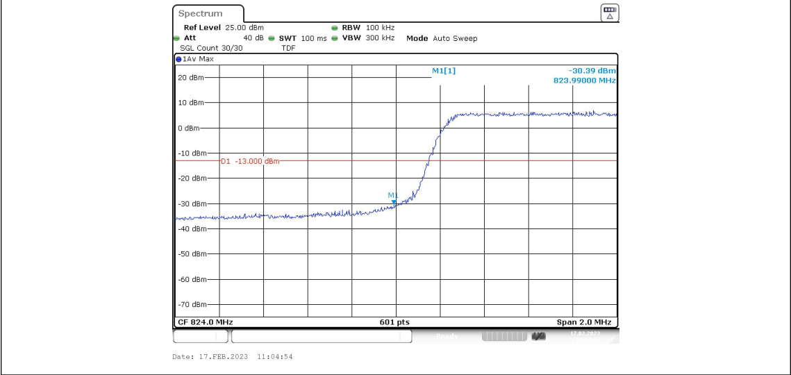
Band5-5MHz-16QAM-20625-1RB#0
