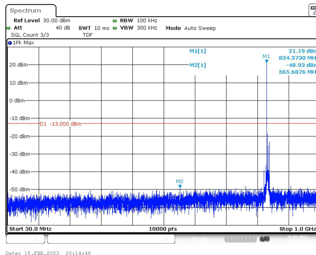
Band5-5MHz-16QAM-20525-1RB#0-Range2:1000~10000MHz
