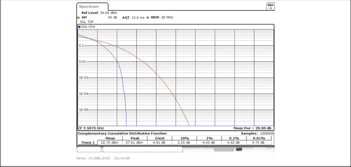
Band7-15MHz-QPSK-20825-75RB#0
