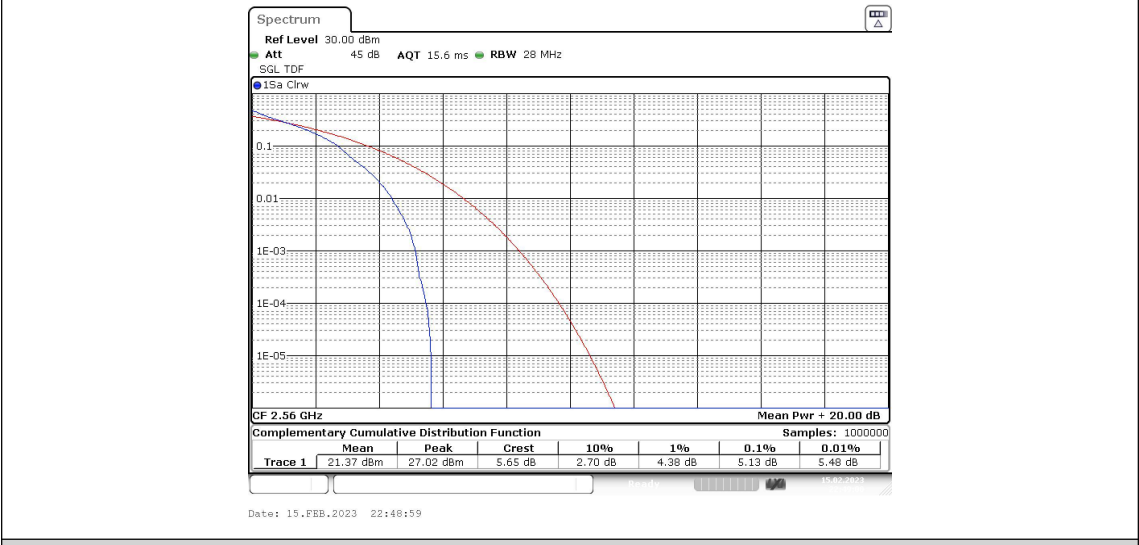
Band7-20MHz-QPSK-21350-100RB#0
