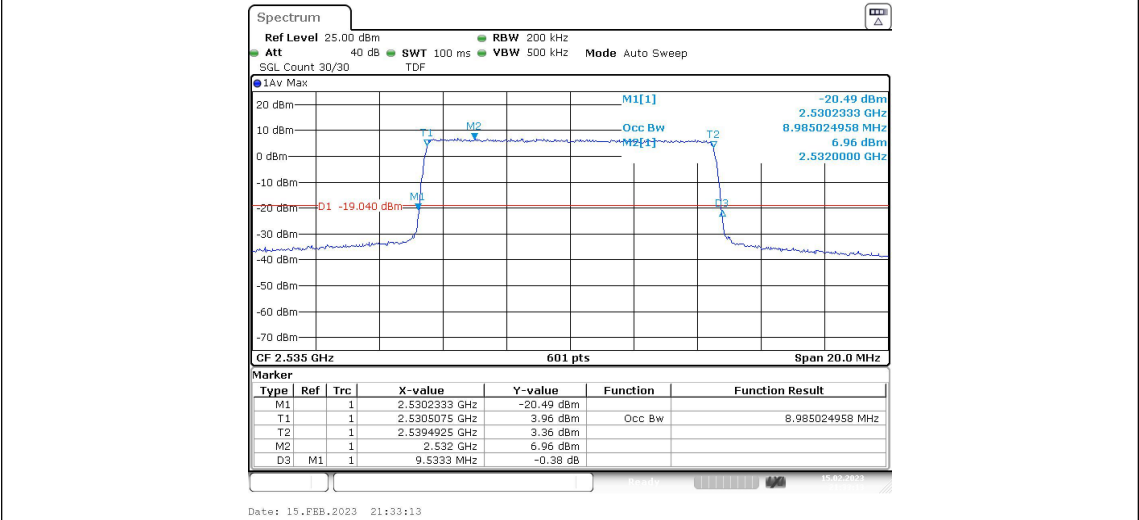
Band7-10MHz-QPSK-21400-50RB#0
