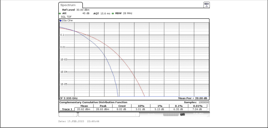
Band7-20MHz-16QAM-21350-1RB#0
