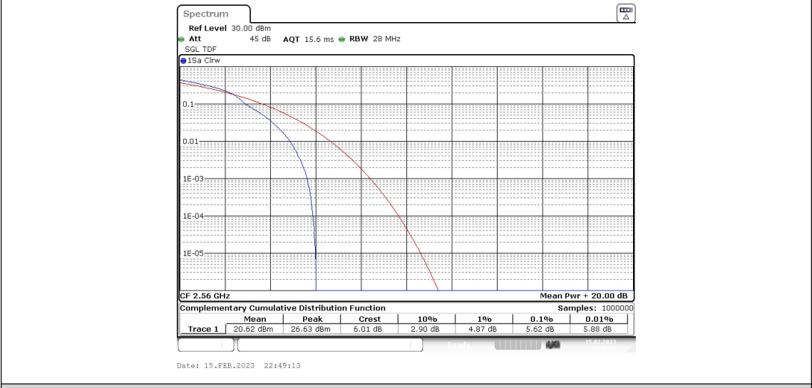
Band7-20MHz-16QAM-21350-100RB#0
