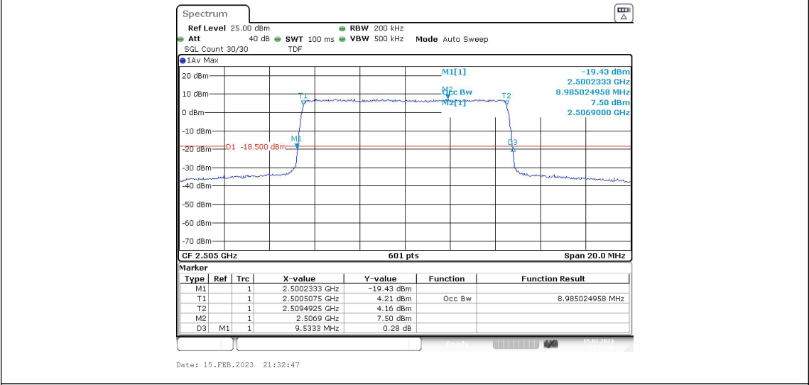
Band7-10MHz-QPSK-21100-50RB#0
