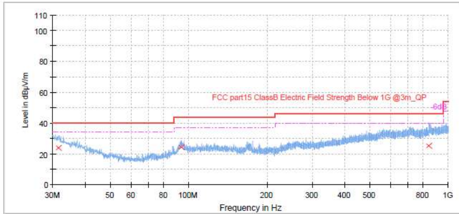
Figure 12: Spectral Diagrams, Radiated Spurious Emission, Mode A.2
