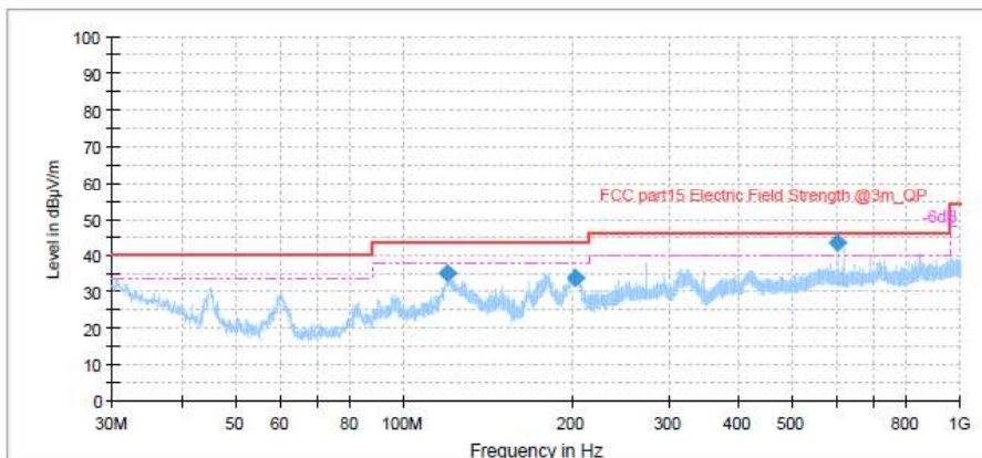
Figure 17: Spectral Diagrams, Radiated Emission, Mode E, Adapter 1 30MHz-1000MHz, Horizontal
