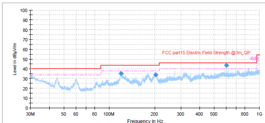
Figure 19: Spectral Diagrams, Radiated Emission, Mode C, Adapter 1
