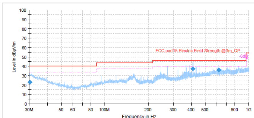
Figure 22: Spectral Diagrams, Radiated Emission, Mode D, Adapter 2
