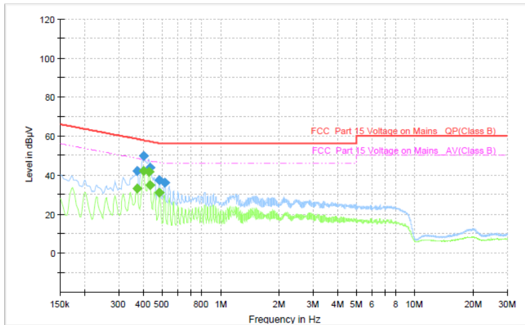
Figure 11: Spectral Diagrams, Conducted Emission, 150KHz - 30MHz, L, Adapter 1, Mode D
