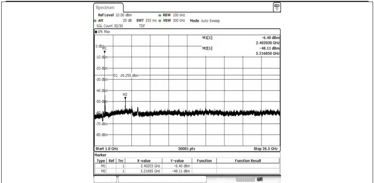
DH5-Ant1-2402-1000~26500-PASS
