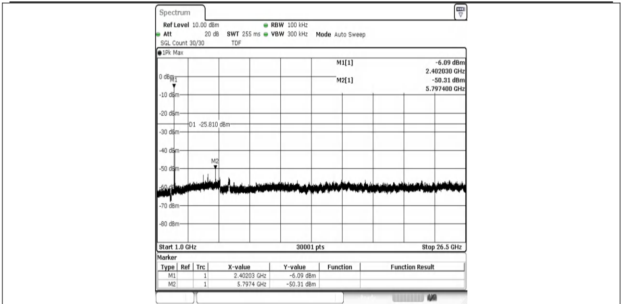
3DH5-Ant1-2402-1000~26500-PASS
