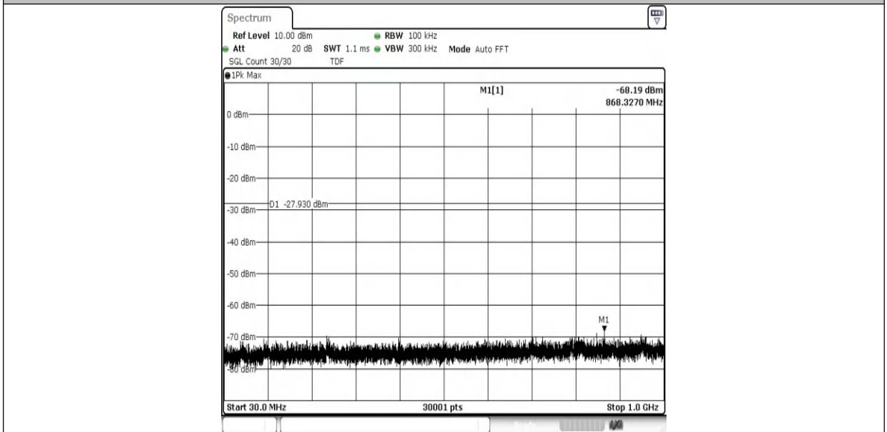
2DH5-Ant1-2441-0~Reference-PASS
