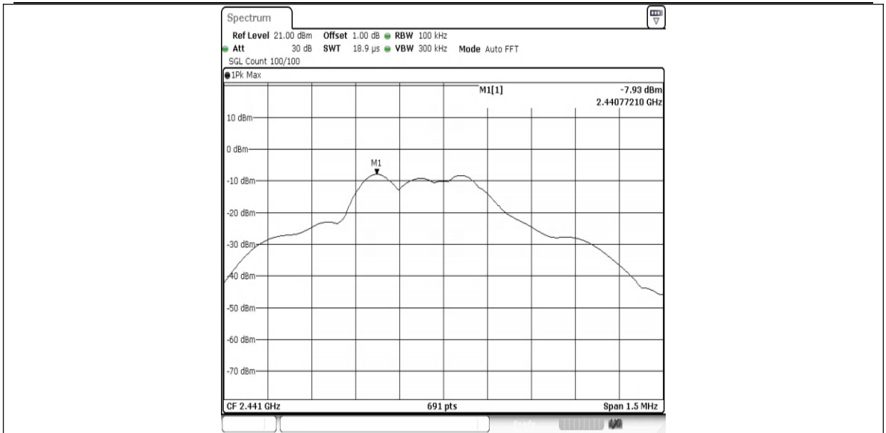
2DH5-Ant1-2441-0~Reference-PASS
